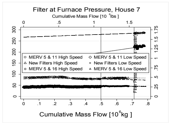
Figure 6: Pressure across the plenum filter for House 7.
