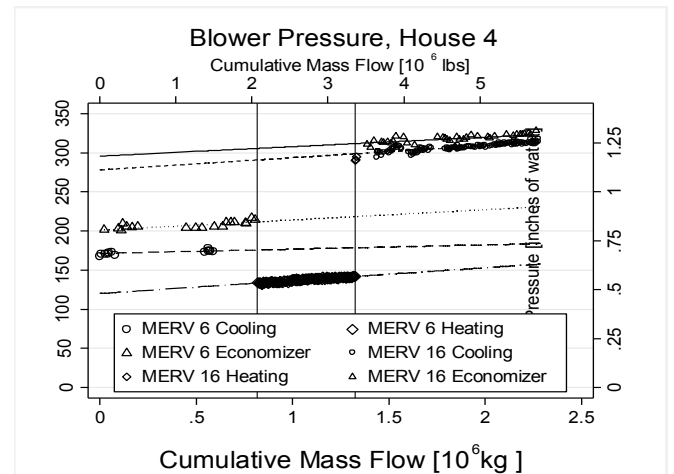
Figure 3: Pressure across the blower for House 4.
