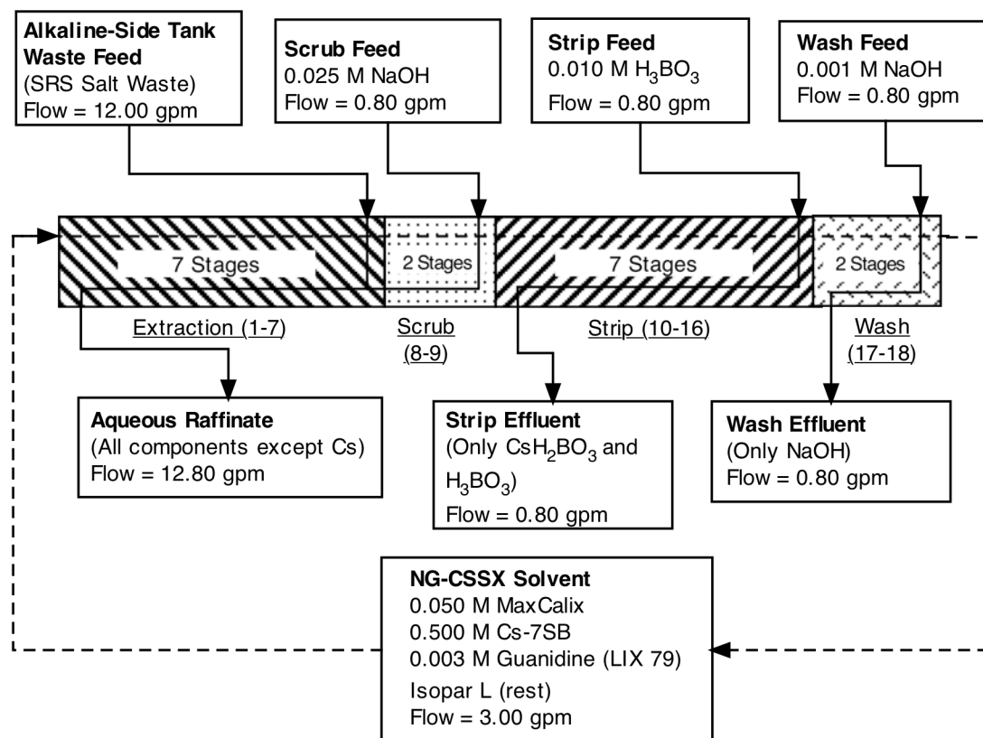
Fig. 13.1. Using simulant test data provided by ORNL as verified by real-waste test data at SRNL, the above flowsheet was calculated to have \text{DF} \geq 40,000 in the MCU equipment configuration (see Chapter 3 39 ).
