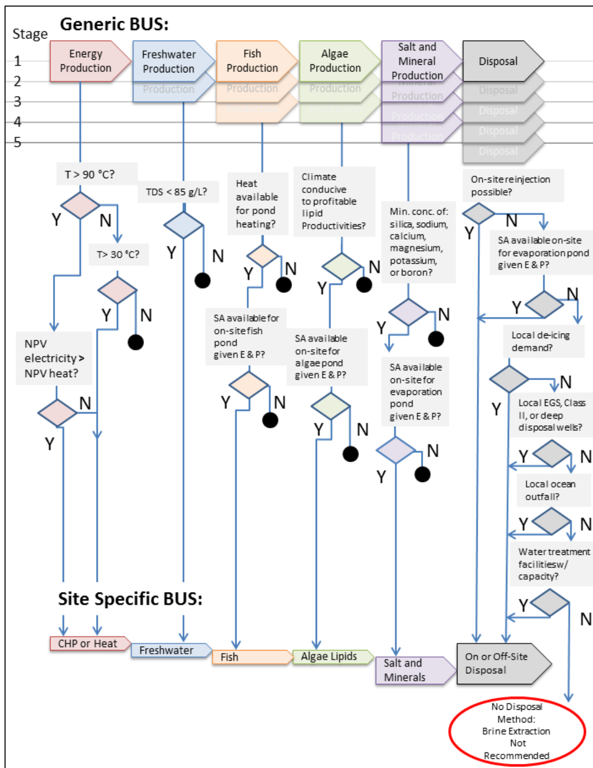
Figure 4. Diagram of BUS method for sequencing on- and off-site brine management stages included in study. Brine temperature (T), brine TDS, treatment net present value (NPV), and surface area (SA) requirements calculated from evaporation (E) or precipitation (P) data are some inputs. Combined heat and power (CHP) is the generation of electricity as well as heat. A black dot indicates the brine management option cannot be included in the site specific BUS. See text for explanation (Breunig et al. 2013).
