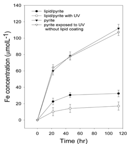
Figure 9: The amount of iron release (i.e., pyrite oxidation) for a given time interval is lowest for the lipid/pyrite surface that had been exposed to UV radiation prior to the start of the Fe release measurements.
