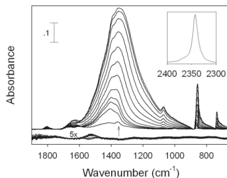
Figure 2: In situ ATR-FTIR data associated with the transformation of nano hematite to siderite in the presence of supercritical carbon dioxide and sulfide. All spectra were taken at 70 °C under 82 bar CO 2 and are offset for clarity. Siderite formation becomes noticeable from these data after 1 h of reaction time. Pyrite is another reaction product. 2
