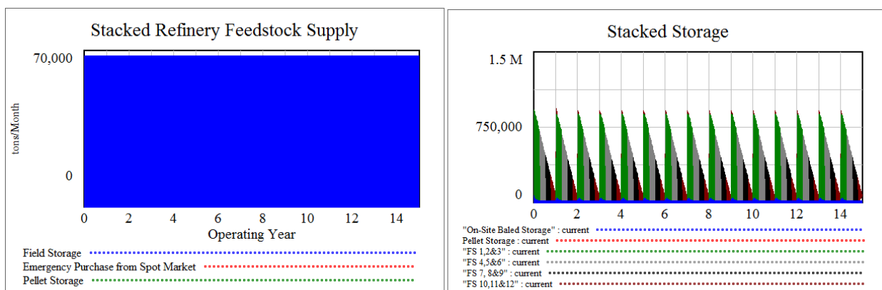
Figure 7: Base case simulation results, the biorefinery experiences consistent harvest values and no supply interruptions occur.
