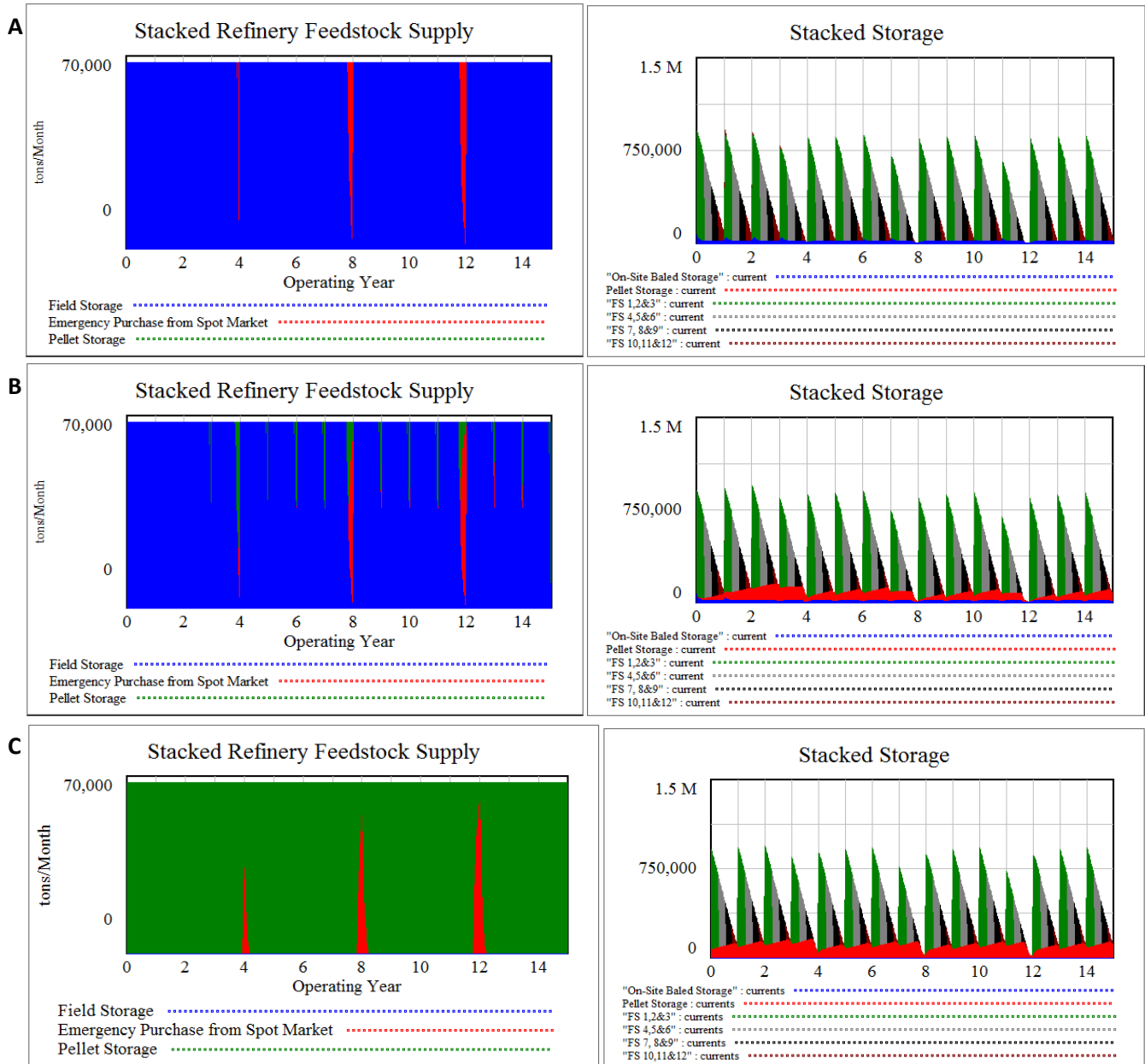
Figure 8: Base case model output for the three configurations under A) Conventional B) Hybrid and C) Uniform-Format Configurations
