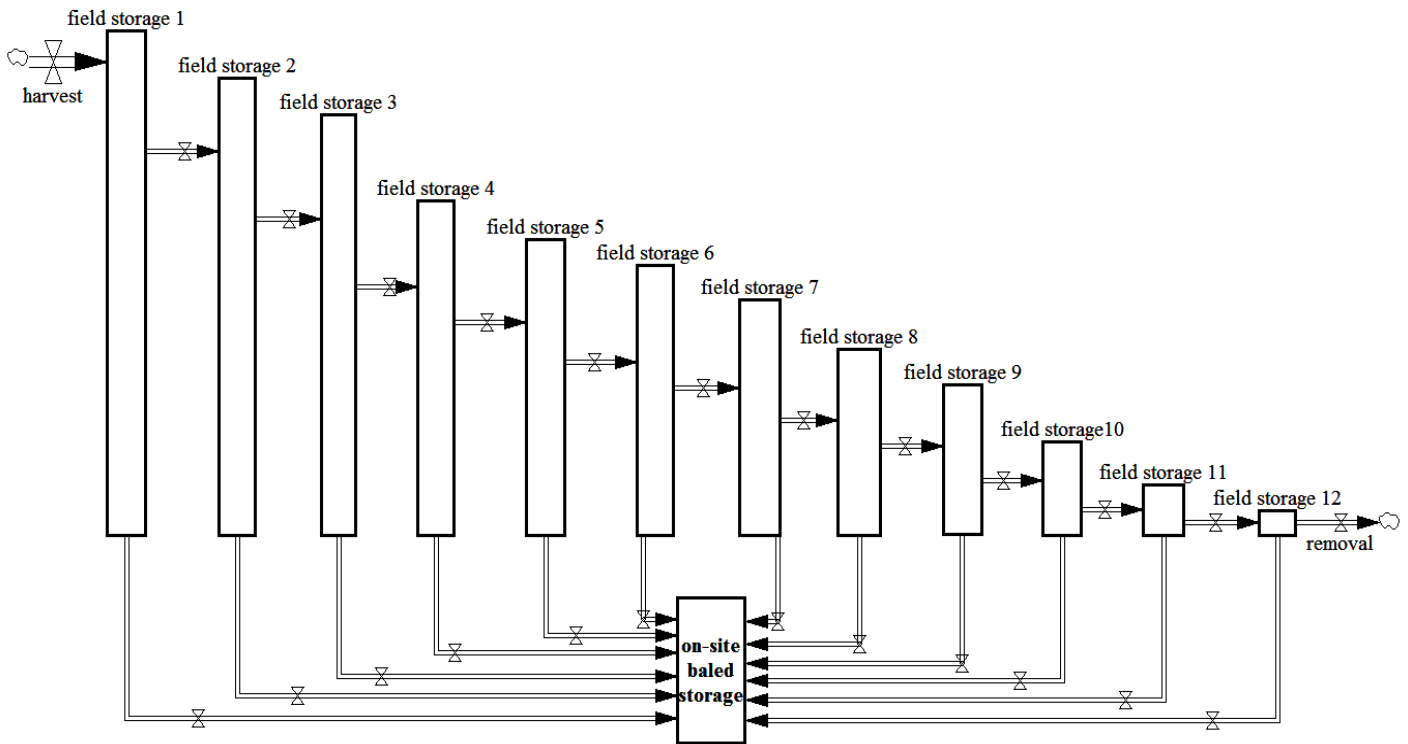
Figure 5: The aging chain structure of BPSS, each field storage stock number corresponds to the age of the biomass. At the end of the operational year any remaining biomass is removed.
