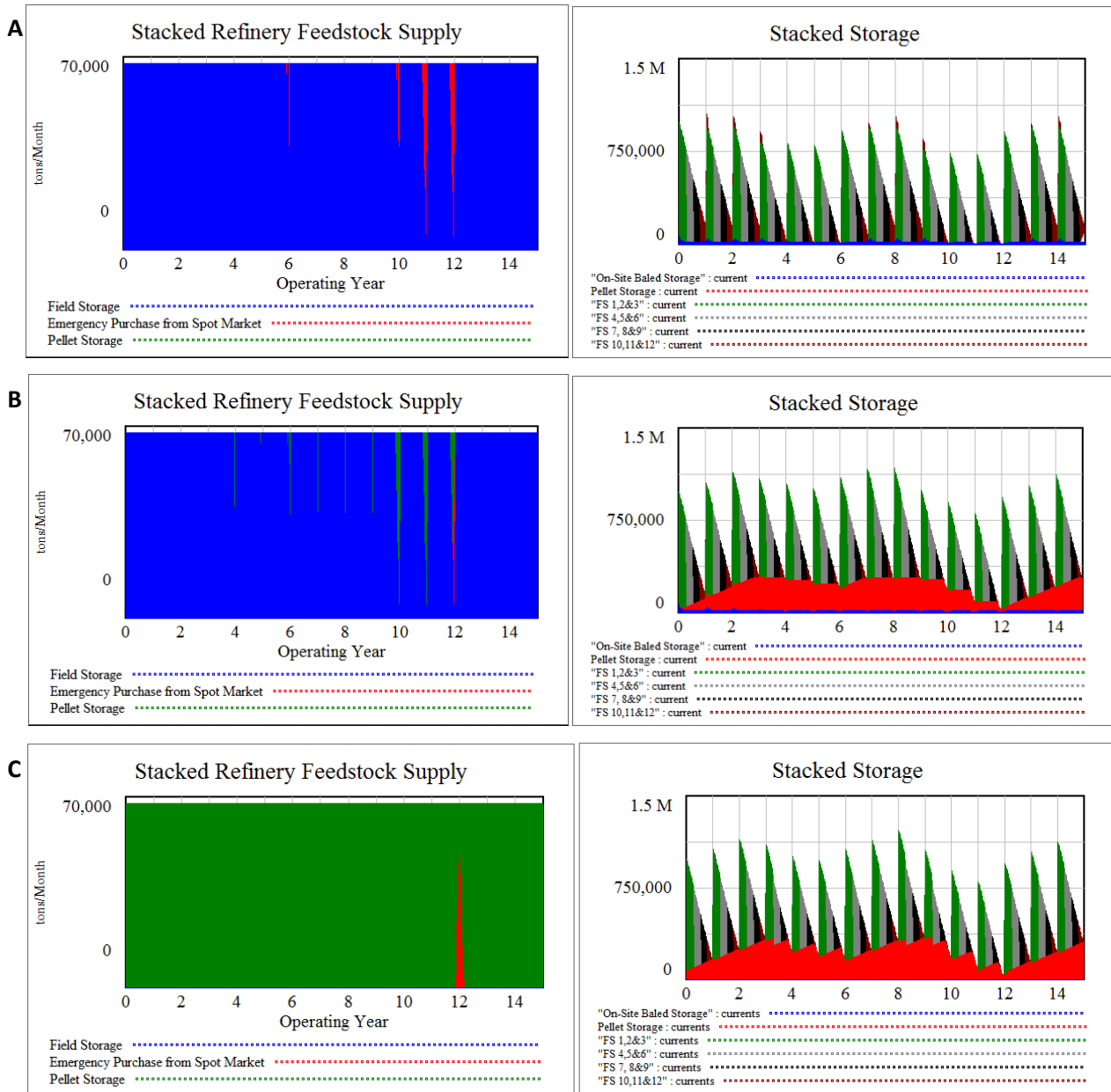
Figure 10: Extended drought may occur thereby placing different demands on the biorefinery.
