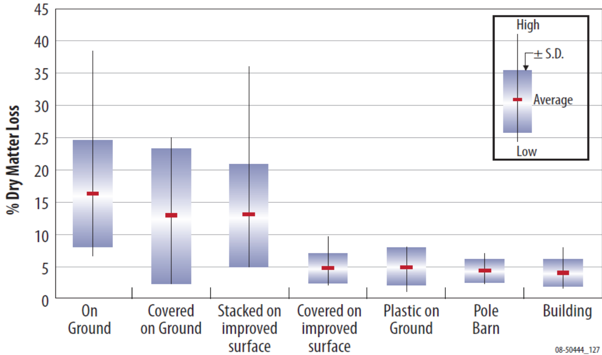
Figure 3: Average losses experienced under different storage configurations (Hess et al., 2009)
