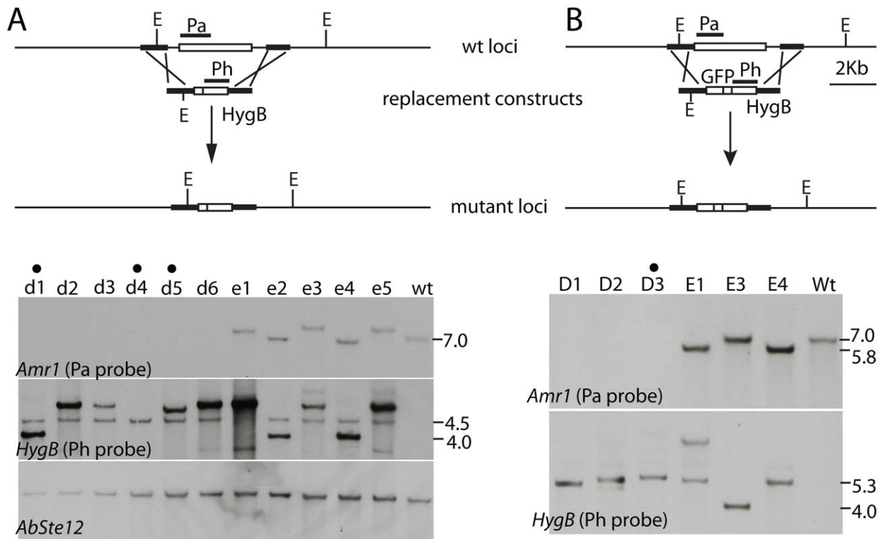
Figure 1. Verification of Amr1 deletion mutants. A. Replacement of the Amr1 coding region with the selectable marker, Hygromycin B transferase (HygB) resistance cassette. On the HygB-probed blot, the expected 4.5 Kb band indicates a single copy insertion of the Hyg B resistance cassette in lane d4. Additional bands in the other lanes suggest multiple insertions of the cassette. B. Replacement of the Amr1 coding region with a green fluorescent protein (GFP) coding region and a HygB cassette. The upper panel of both A and B is a schematic diagram of wild-type ( wt ) and mutant loci and the lower panel consists of five Southern blots showing loss of the Amr1 gene in selected mutants. Dots (•) indicate lanes of mutants used in this study. Probe regions are marked by P h and P a . Abbreviations: E = EcoRI enzyme digestion site. d1 = \Delta amr1 -1, d4 = \Delta amr1 -4, d5 = \Delta amr1 -5, and D3 = \Delta amr1 : Amr1p -GFP. e1-e5, E1, E3, and E4 are ectopic insertion mutants. doi:10.1371/journal.ppat.1002974.g001
