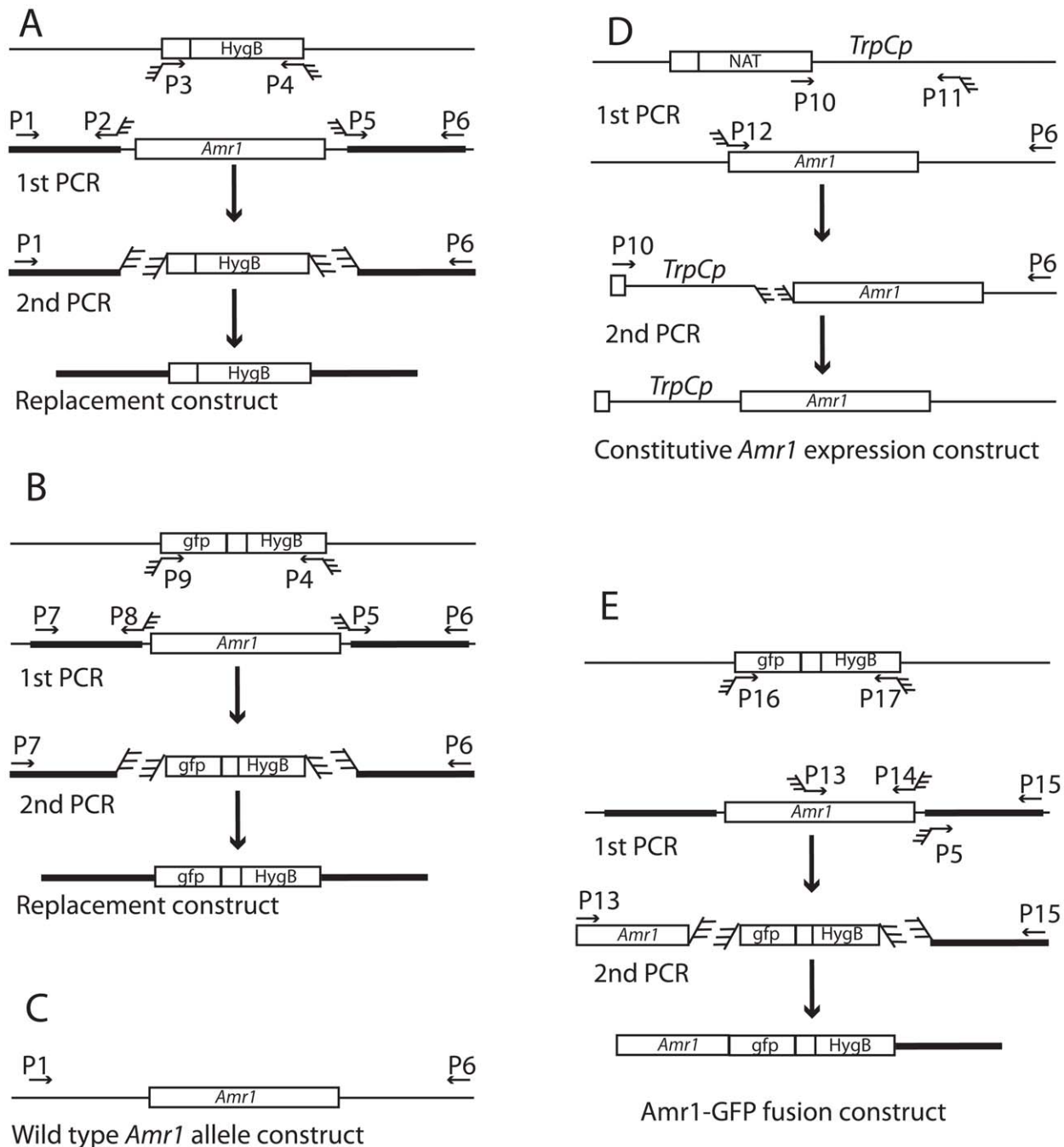
Figure 8. Schematic diagram of the PCR strategy used to make each construct. A. Construct for replacement of the Amr1 gene with a Hygromycin B resistance cassette. B. Construct for replacement of the Amr1 gene with a GFP coding region and Hygromycin B resistance cassette. C. Amplification of the wild-type allele of the Amr1 gene. D. Construct for the constitutive Amr1 expression cassette. E. Construct for the Amr1 -GFP fusion protein expression.
