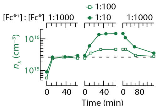
Figure 6. Hole majority carrier density, n_h (—), of two PbSe nanocrystal solid films as a function of the time duration of exposure to \text{Fc}^+/\text{Fc}^* doping solutions. The initial points represent untreated films. Both films were exposed to a 5 mM 1:1000 \text{Fc}^+/\text{Fc}^* doping solution in acetonitrile for the first and last time series whereas one was exposed to a 5 mM 1:10 (closed circles) and the other, a 5 mM 1:100 (open squares) \text{Fc}^+/\text{Fc}^* doping solution in between.
