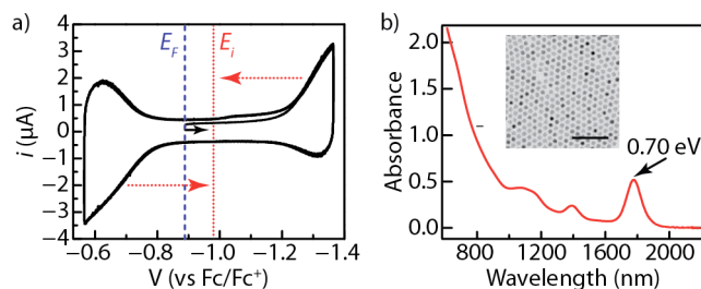
Figure 2. (a) Low temperature, -37^{\circ}\text{C} , cyclic voltammogram of an EDT-treated PbSe nanocrystal solid cast onto an ITO working electrode recorded in acetonitrile containing 0.1 M \text{Bu}_4\text{NPF}_6 . Scan initiated from the open-circuit potential, E_f (— blue —), in the negative direction (black arrow) at 200 mV/sec. Dotted red arrows serve as guides to the eye indicating the potential, E_i (■ ■ ■), equally separated from the rising anodic and cathodic waves as calculated in Figure S4. (b) Optical absorbance spectra of PbSe nanocrystals dispersed in carbon tetrachloride exhibiting a first exciton feature at 0.70 eV (1777 nm). Inset: Transmission electron micrograph of PbSe nanocrystals. Scale bar corresponds to 50 nm.
