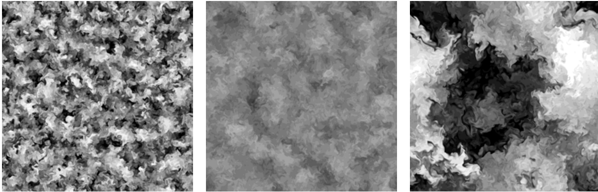
Figure: Volume fraction contours in the horizontal plane at early, intermediate (deceleration) and late-times (reacceleration).
