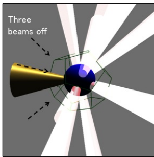
Figure 1: GekkoXII nine-beam irradiation.
