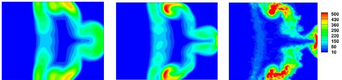
Figure 3: Maximum turbulent kinetic energy for the inverse chevron RM case; comparison of the original K-L (left), improved K-L (middle) and ILES.
