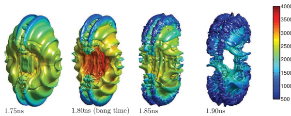
Figure 1: Fuel mass concentration c_{fuel} = 0.1 isosurface colored with T_{ion} (eV) [1].
