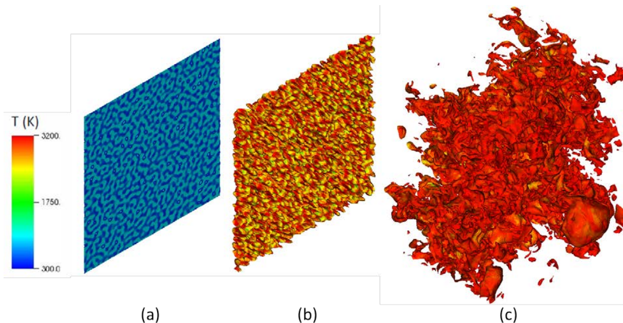
Contours of temperature superposed on the flame sheet (identified as the surface of stoichiometric mixture fraction) at (a) initial, (b) before reshock and (c) late times after reshock.
