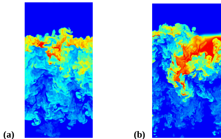
Figure 1: Break of a dense fluid layer due to RT instability. (a) ILES (256x256x512 meshes). (b) DNS, Re \sim 3000 , Sc=1 (1024x1024x2048 meshes).
