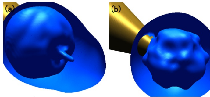
Figure 2: Density iso-surface corresponding to fuel-shell interface. (a) nine-beam (b) twelve-beam
