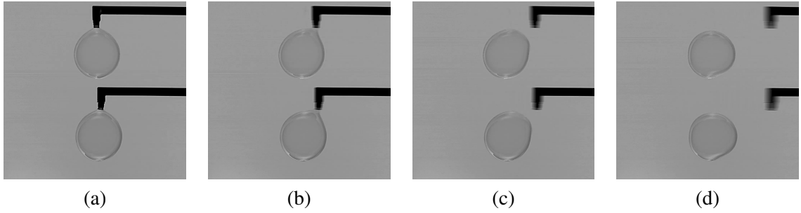
Figure 1: Initial condition setup. (a) Initial retractor position. Time after initiating retraction: (b) 36 ms, (c) 48 ms and (d) 64 ms.
