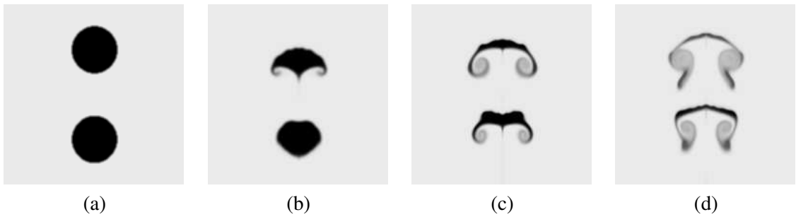
Figure 2: Simulation of shocked bubble pair for M=1.37 in N_2 with Xe bubble gas. Non-dimensional “cloud-crushing time” is t^* = \frac{Wt}{D} , where W is shock speed, t is time and D is bubble diameter. (a) Initial bubble position, t^* = 0 , (b) t^* = 4 , t^* = 8 and t^* = 12 .
