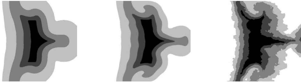
Figure 2: Volume fraction contours for the 2D inverse chevron RM case; comparison of the original K-L (left), improved K-L (middle), and ILES (right).
