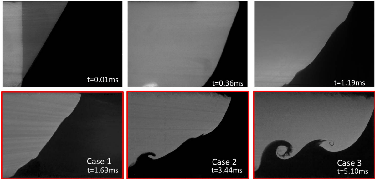
Figure 1: Initial shock development of inclined interface RMI for Mach 1.55, Atwood 0.23, and Angle of inclination 60°.
