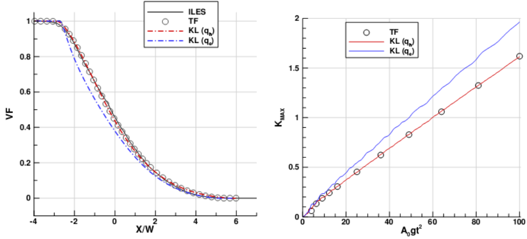
Figure 1: Volume fraction (left) and maximum turbulent kinetic energy for RT mixing with density ratio 20:1. Comparison of the two-fluid model (TF), original K-L (blue line), improved K-L (red line) and ILES data.
