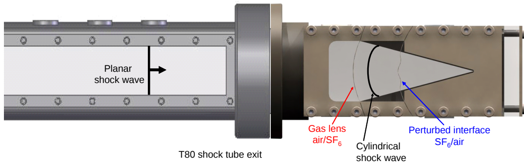
Figure 1: Sketch of the new convergent test section implemented on T80 shock tube exit.
