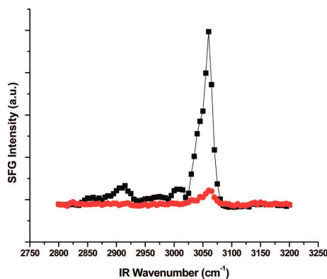
Figure 2.13: SFG spectra of equivalent polystyrene film on a prism (black) and a flat slab (red).
