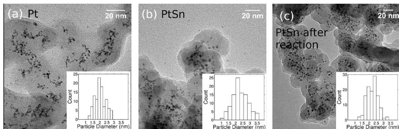
Figure S.6.1: Colloidally prepared Pt nanoparticles. The nanoparticles shown are encapsulated in a porous silica shell to inhibit nanoparticle sintering during heat treatments. (b) Colloidally prepared PtSn nanoparticles encapsulated in silica. (c) PtSn nanoparticles after treatment and reaction studies. The nanoparticle morphology is maintained. Histogram insets show the average and deviation of the particle size in nanometers.
