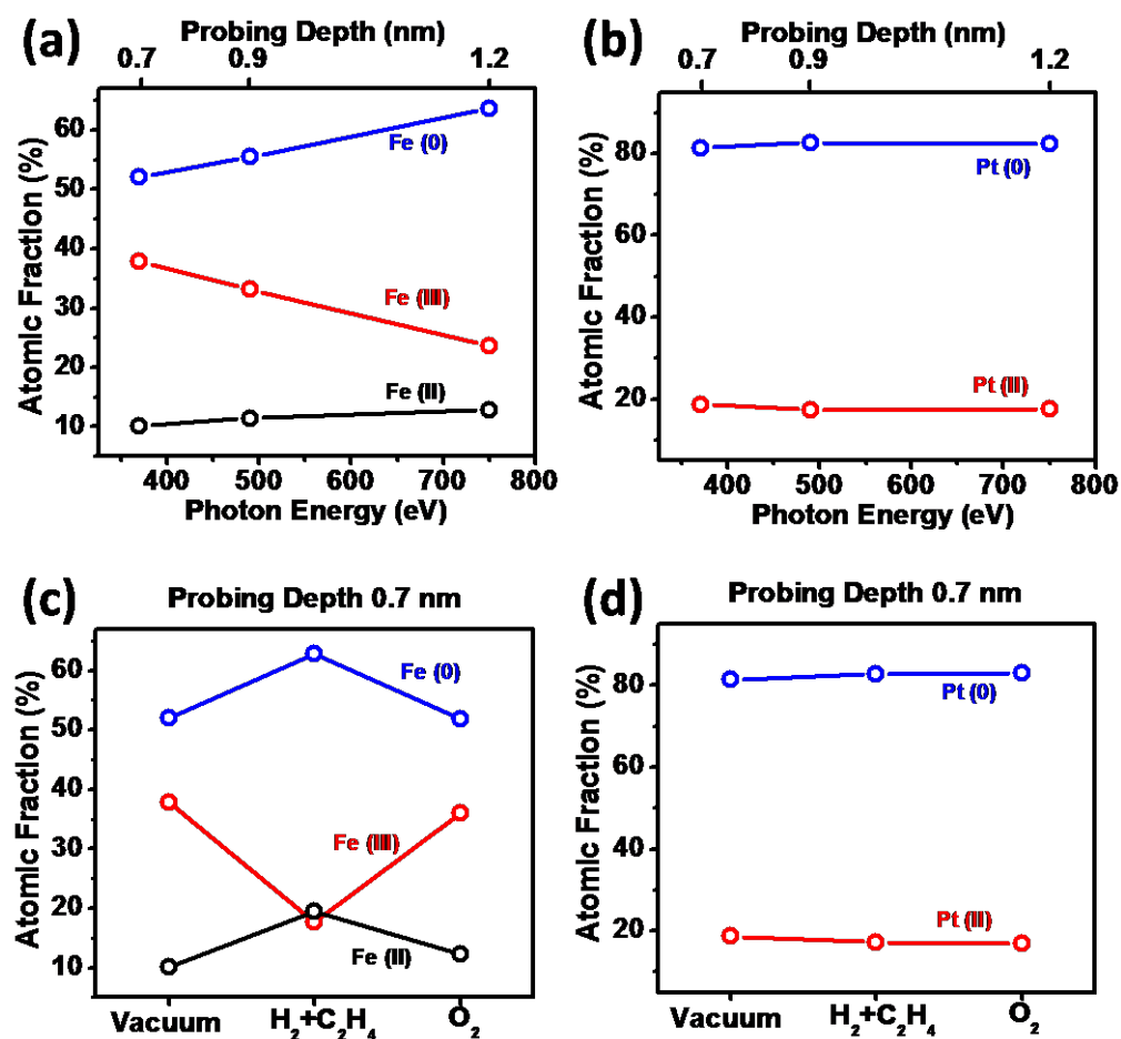
Figure 7.4: Probing depth and gas atmosphere dependent oxidation state distributions of Pt and Fe in 2 nm PtFe nanoparticles as probed by AP-XPS. Probing depth dependent oxidation states were probed by XPS in vacuum with incident X-ray photon energies of 370, 490 and 750 eV (corresponding to approximate probing depths of 0.7, 0.9 and 1.2 nm) at 25°C. Gas atmosphere dependent oxidation states were probed by XPS in H_2 + C_2H_4 (100 + 10 mTorr) and O_2 (100 mTorr) environment at 25°C with incident X-ray photon energy of 370 eV (~0.7 nm probing depth). (a) Atomic fractions of Fe species with different oxidation states in the PtFe nanoparticles vs. incident X-ray photon energy and probing depth. (b) Atomic fractions of Pt species with different oxidation states in the PtFe nanoparticles vs. incident X-ray photon energy and probing depth. (c) Atomic fractions of Fe species with different oxidation states at the
