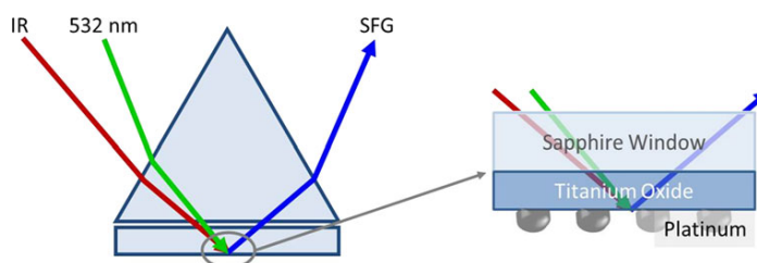
Figure 4.1: Diagram showing how a sapphire prism directed the VIS and IR beams onto the catalyst surface for SFG vibrational spectroscopy. The catalyst was prepared on the back side of a sapphire window and consisted of a thin film of \text{TiO}_2 acting as a support for Pt nanoparticles.
