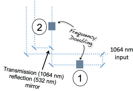
Figure 2.8: Frequency double with non-linear crystals is the first step after the laser. The orientation of (1) can affect the power of the visible and tunable infrared beams used for SFG.
