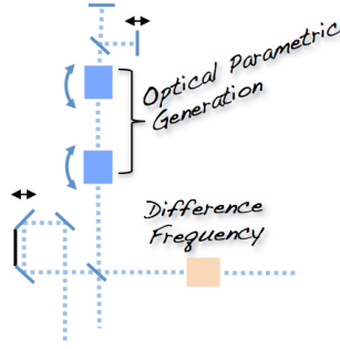
Figure 2.10: Two KTP crystals perform optical parametric generation (OPG) with 532 nm input.
