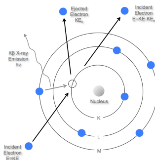
Figure 2.17: Fundamental process required for energy dispersive X-ray spectroscopy (EDS).
