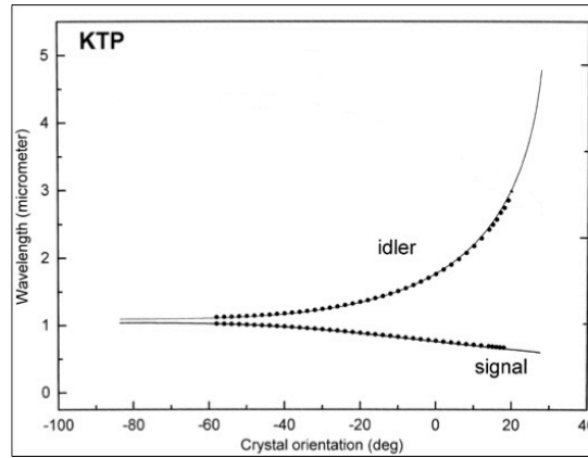
Figure 2.11: Example type II KTP (KTiOPO 4 ) tuning curve from Girardeau-Montaut et al. 3
