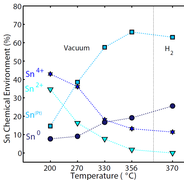
Figure S.6.5: Progression of the different Sn chemical environments in the PtSn nanoparticle catalysts during pretreatment under vacuum and H 2 atmospheres measured using ambient pressure X-ray photoelectron spectroscopy. Each trend line corresponds to a feature in the XPS spectra in Figure S.6.4. The as-prepared 2 nm PtSn catalyst comprised Sn 4+ and Sn 2+ oxides that were reduced during heat treatment.
