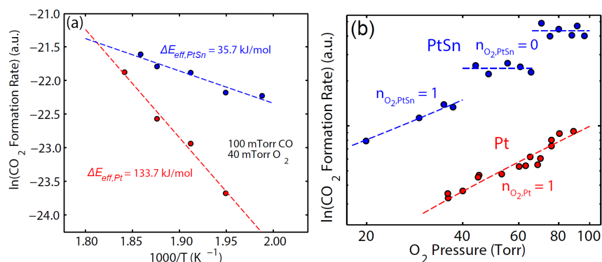
Figure 6.1: (a) Arrhenius plot for CO 2 formation on 2 nm Pt (red) and 2 nm PtSn (blue) nanoparticle catalysts. The reaction rates were determined between 200 and 300 °C. (b) Plot of the ln(CO 2 formation rate) versus ln(P O 2 ) yields the reaction order in O 2 for 2 nm Pt (red) and 2 nm PtSn (blue) catalysts.
