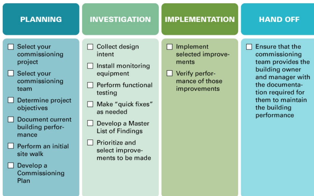
Figure 3. Phases of a building commissioning project
