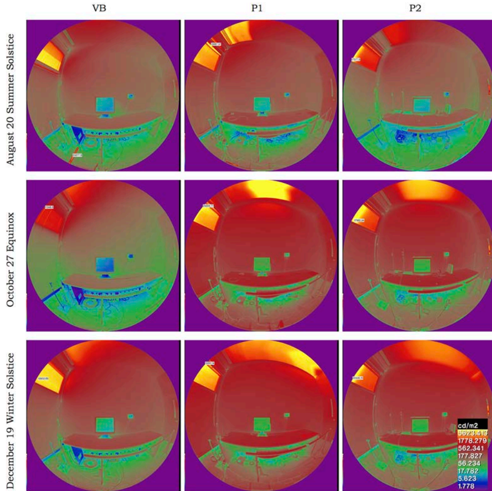
Fig. 6. Falsecolor luminance images ( \text{cd/m}^2 ) of the test room looking toward the west side wall (window on the left) at noon on August 20, 2012 (top), October 27, 2012 (middle), and December 19, 2012 (bottom). Venetian blind (VB) (left), P1 system (middle), P2 system (right).
