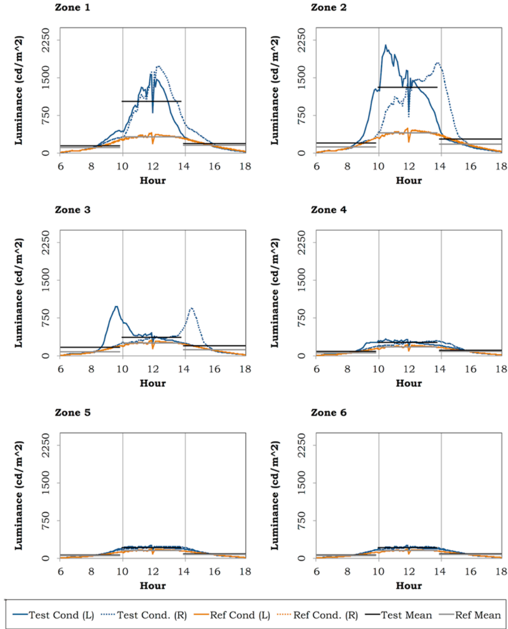
Fig. 9. Ceiling luminance by zone under clear sky conditions on April 9, 2011. Zone 1 is closer to the window and zone 6 is the farthest from the window. Phase 1, P1 system.
