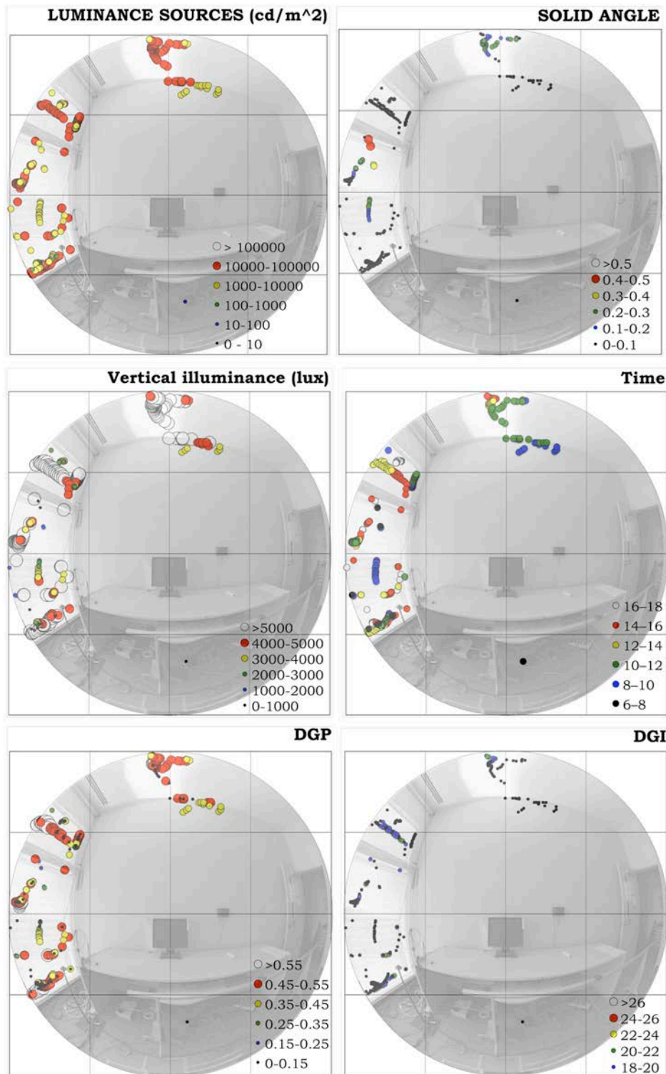
Fig. 22. A: Luminance of glare sources (cd/m 2 ), B: size of glare sources (st), C: range of vertical illuminance (lux) for the identified glare sources; D: time of day when the glare occurred, E: DGP associated with the glare sources, F: DGI associated with the glare sources. Data are given for the P1 system looking toward the west sidewall on March 12, 2013 under clear sky conditions. The lower
