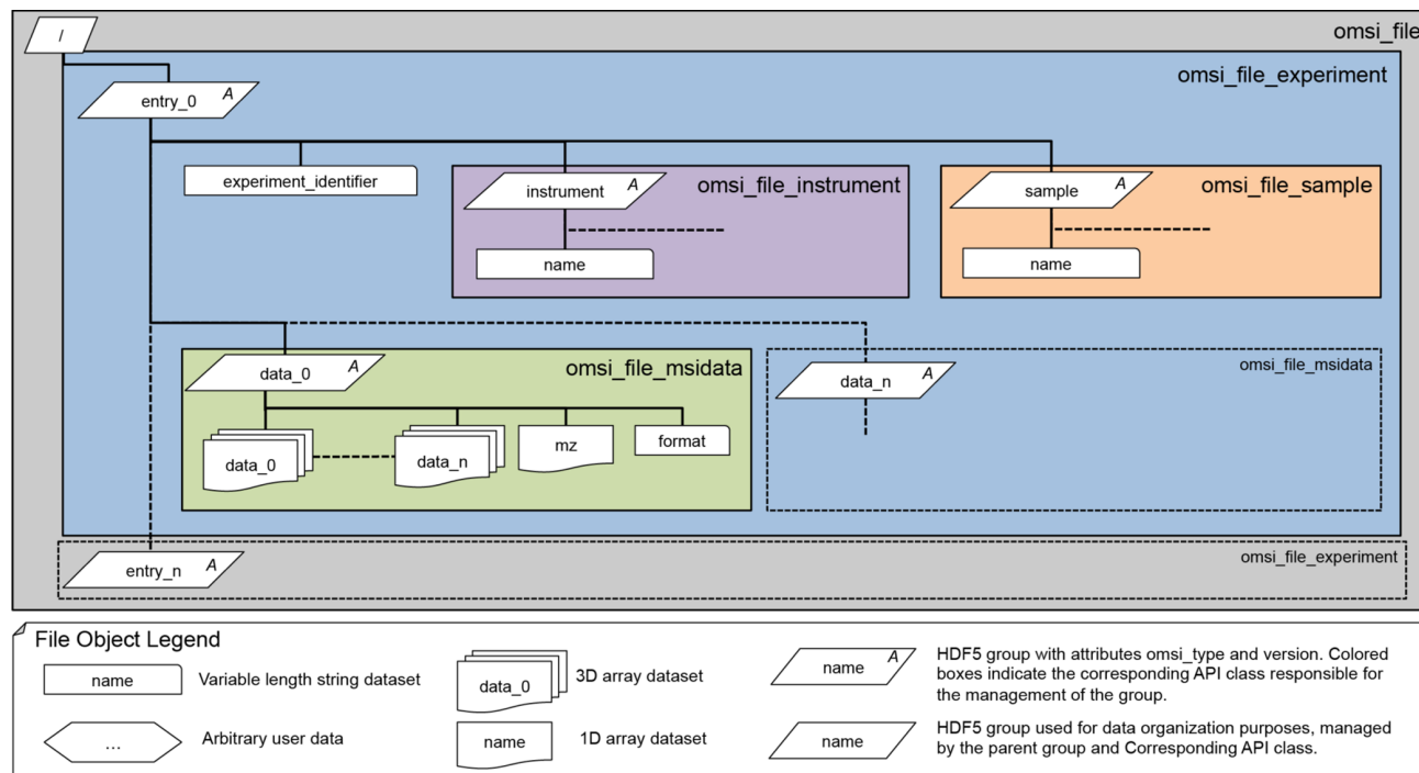
Figure 2. Overview of the hierarchy of the OpenMSI file format. The omsi file format and API follow the same semantic hierarchy. Each main HDF5 group is managed in the omsi file format API by a corresponding class (colored boxes) responsible for providing access to and creating the direct content of the group in the file.
