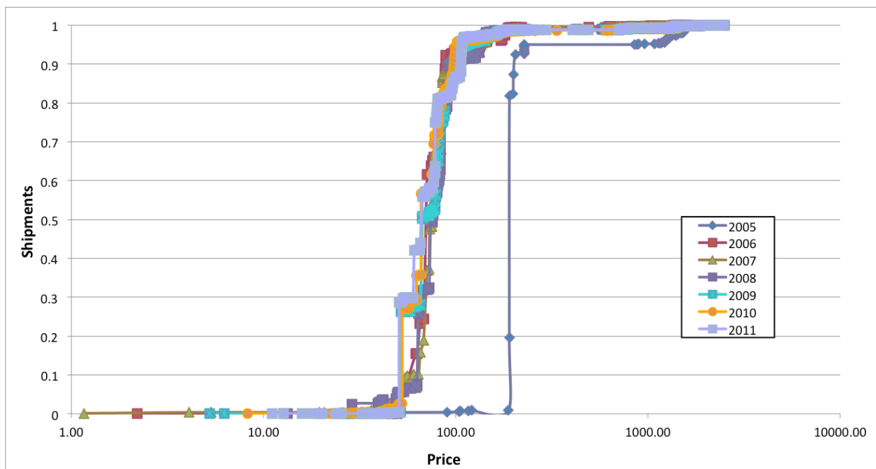
Figure A.2.1. NPD cumulative prices for 1-11 bottle capacity wine/beverage coolers by year
