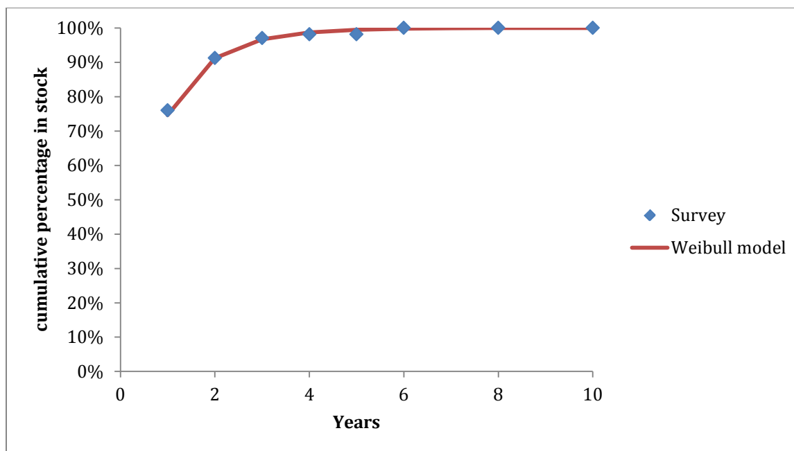
Figure 29. Lifetime function fit for non-vapor compression refrigerators
