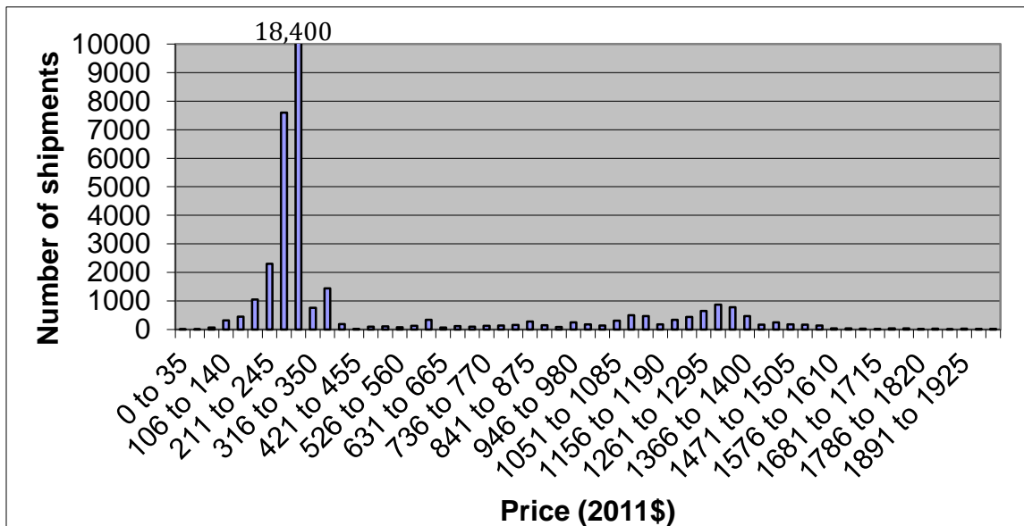
Figure 45. NPD average 2009-2011 prices for 40-59 bottle capacity wine/beverage coolers. Note that the vertical scale was expanded to show detail; the number of shipments at the one data point whose full height was truncated is labeled on the Figure.
