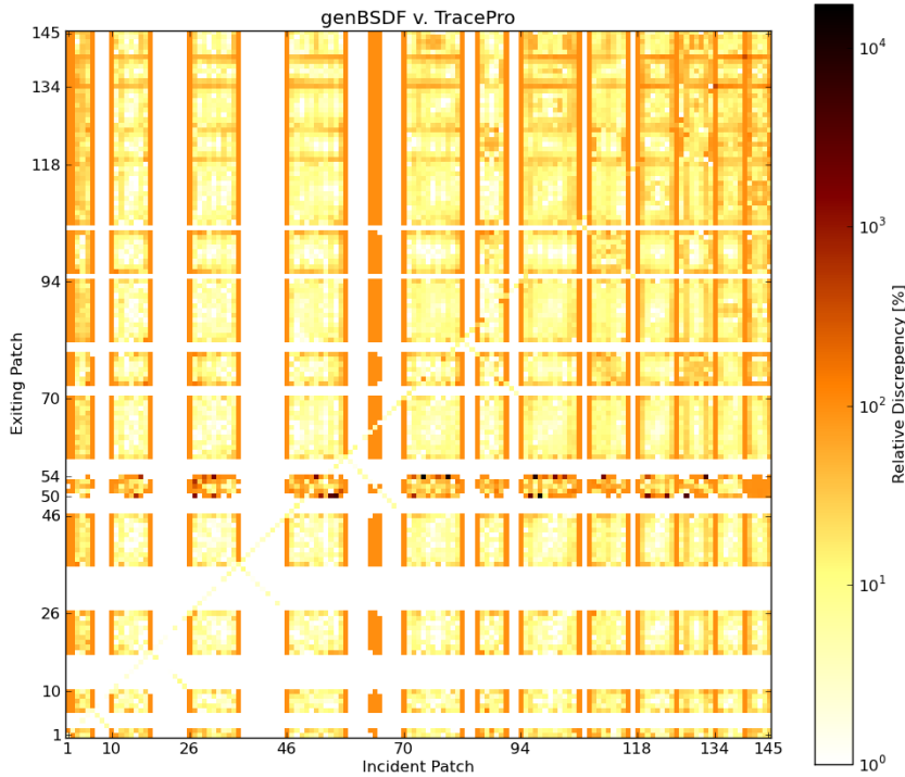
Fig. 5. Percent difference between genBSDF- and TracePro-generated BSRFs (transmission) for flat specular blinds positioned at a horizontal angle.
