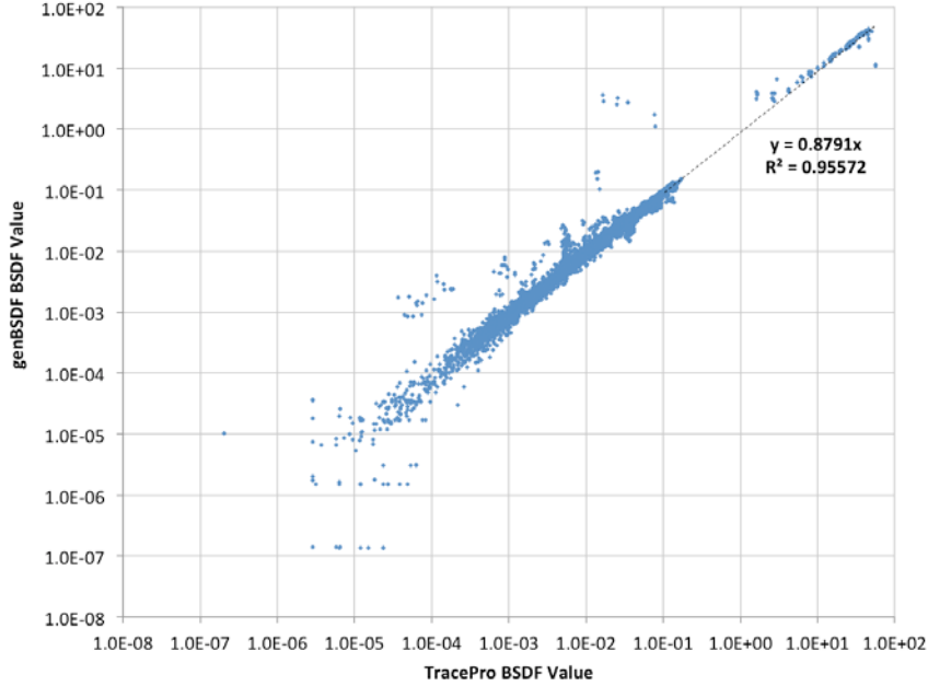
Fig. 4. Scatter plot of the genBSDF results versus the analytically derived, TracePro BSRF values for the specular Venetian blind. The 21,250 transmission values are correlated with a linear regression fit ( r^2=0.95572 ).
