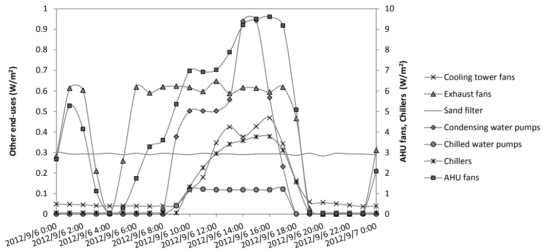
Figure 8 Hourly electrical power density of major HVAC end-uses on a typical weekday
