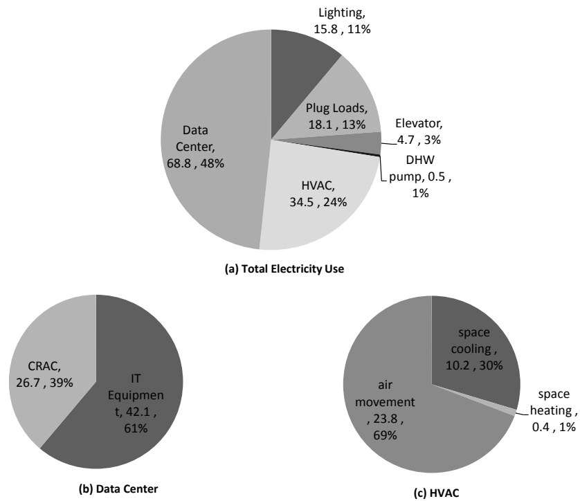
Figure 3 Annual breakdowns of electricity use intensity (unit: kWh/m²a)
