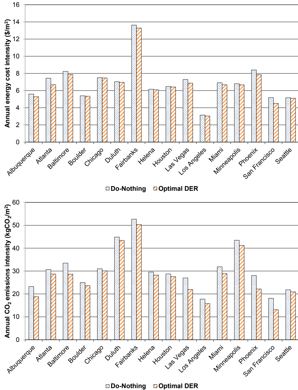
Figure 16 – Abatement of energy cost and CO 2 emissions intensities in the U.S. residential buildings through investment in DER (DER-CAM results).
