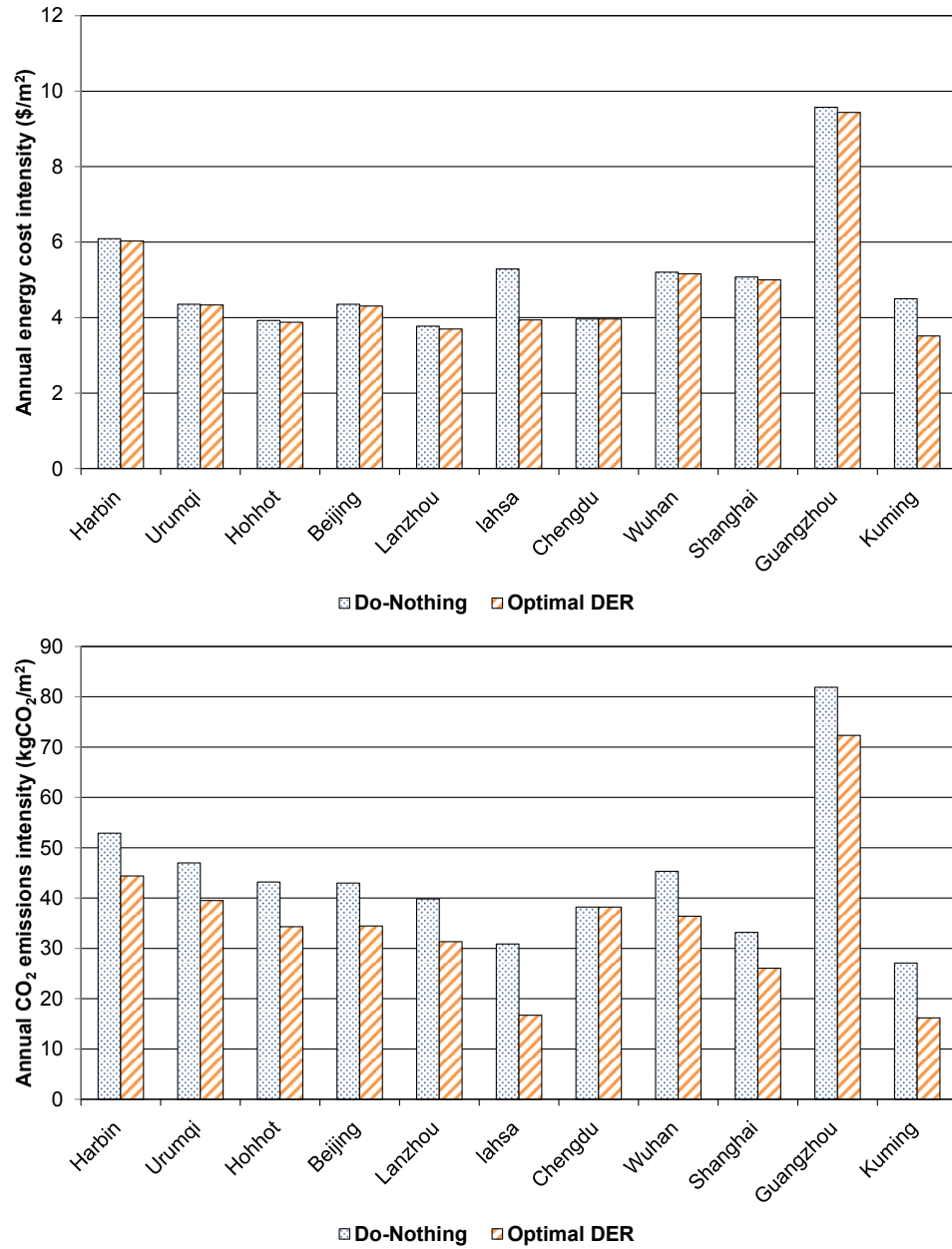
Figure 17 – Abatement of energy cost and CO 2 emissions intensities in the Chinese residential buildings through investment in DER (DER-CAM results).
