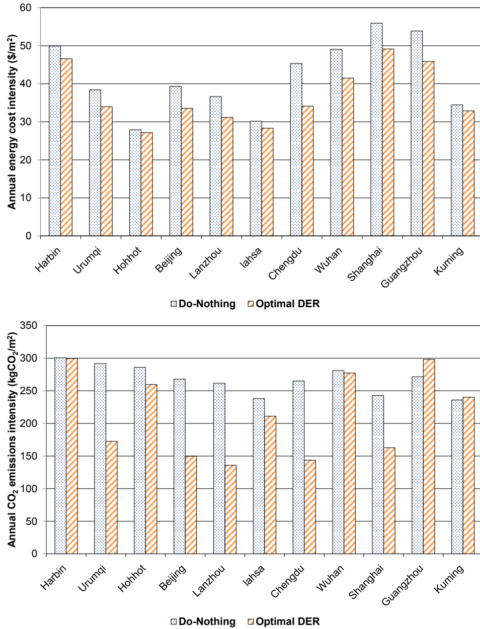
Figure 14 – Abatement of energy cost and CO 2 emissions intensities in the Chinese commercial buildings through investment in DER (DER-CAM results).
