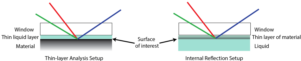
Figure 3.1: Schematic of the thin-layer analysis mode and the internal reflection mode for SFG of the solid-liquid interface.
