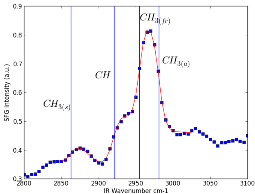
Figure 4.5: SFG spectra of pure isopropanol at the liquid/platinum interface. Fit is shown in red. The modes assigned are the \text{CH}_3 symmetric stretch ( 2863\text{ cm}^{-1} ), CH stretch ( 2921\text{ cm}^{-1} ), \text{CH}_3 fermi resonance ( 2955\text{ cm}^{-1} ) and \text{CH}_3 asymmetric stretch ( 2981\text{ cm}^{-1} ).
