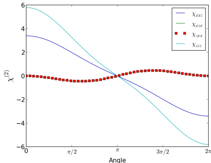
Figure 2.5: The magnitude of \chi_{xxz}^{(2)} , \chi_{xzx}^{(2)} , \chi_{zxx}^{(2)} and \chi_{zzz}^{(2)} of a methyl symmetric stretch mode as a function of its tilt angle with respect to the surface normal. It is worth noting that the xzx and zxx components of \chi^{(2)} are equal for the methyl group and their contributions to the overall SFG intensity become distinct only in the difference in the z and x components of the electric field strength and the Fresnel factor difference.
