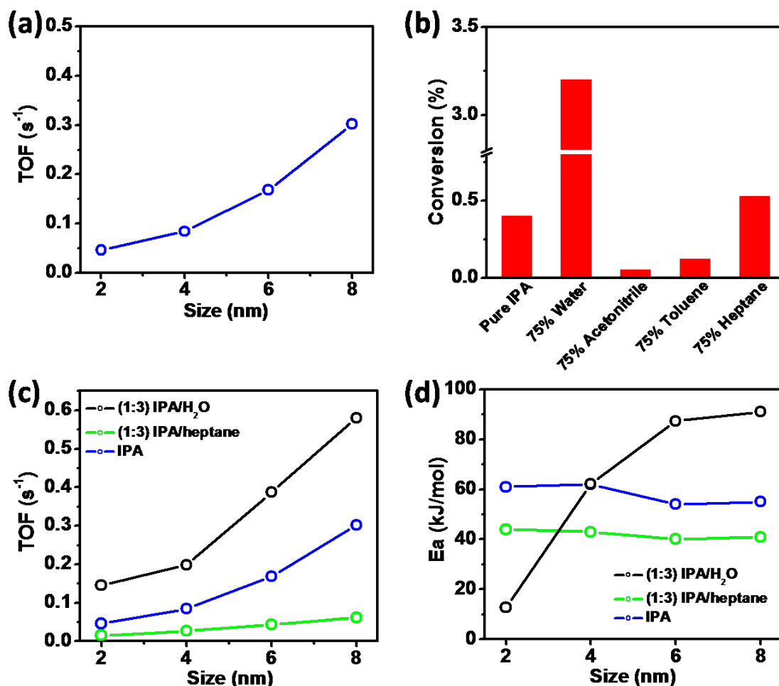
Figure 8.2: Liquid-phase IPA oxidation reaction. (a) TOF in pure IPA catalyzed by Pt nanoparticles with various sizes at 60 °C. (b) Reaction conversion in pure IPA and IPA diluted with various solvents, catalyzed by 4 nm Pt nanoparticles at 60 °C. (c) Comparison of size-dependent TOF in pure IPA and IPA diluted with water and heptane at 60 °C. (d) Comparison of reaction activation energy in pure IPA and IPA diluted with water and heptane, catalyzed by Pt nanoparticles with various sizes at 60 °C.
