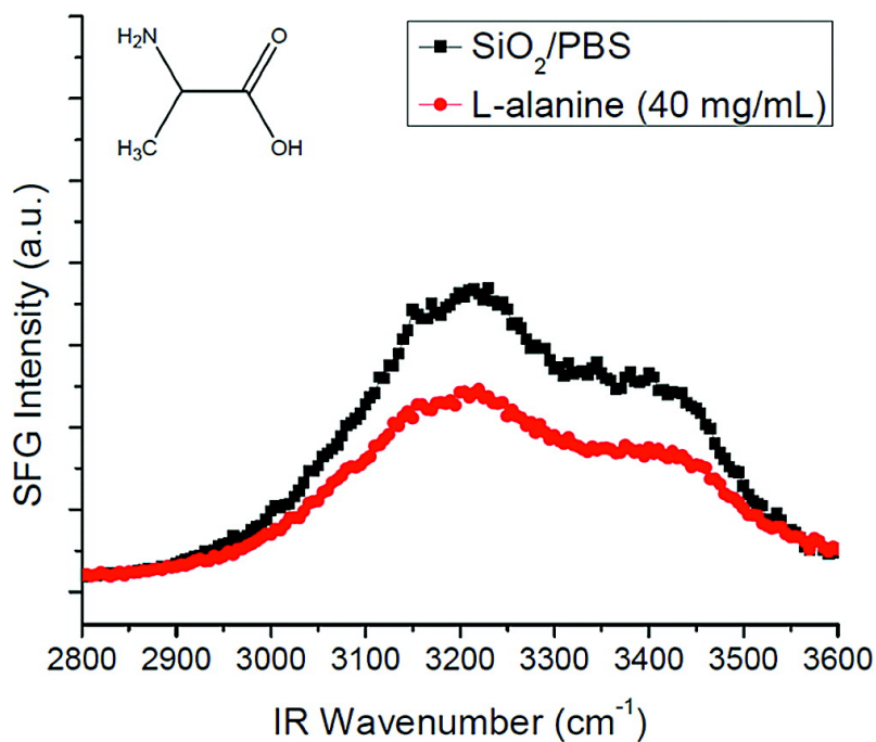
Figure 9.14: SFG spectrum of the SiO 2 /PBS interface before (black squares) and after (red circles) the addition of alanine (40 mg/mL). SFG signal at 3200 and 3400 \text{cm}^{-1} are reduced upon addition of the amino acid.
