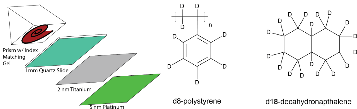
Figure 3.9: Left: Schematic of the catalyst used for SFG and reaction studies coupled with a \text{CaF}_2 prism using the custom index matching gel. A 2 nm adhesion layer is evaporated onto a glass slide, followed by 5 nm of platinum metal. The glass slide is index matched to a \text{CaF}_2 prism using a homemade index matching gel. Right: Molecular structure of the components of the index matching gel.
