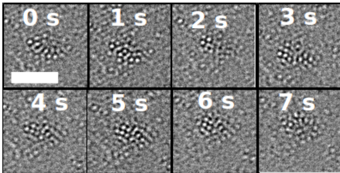
Figure 7.14: Ultrahigh resolution TEM images showing a very small particle fluidly moving between disordered structures. The scale bar in the top left image is 2 nm.
