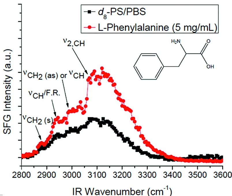
Figure 9.1: SFG spectrum of d_8 PS/PBS interface before (black squares) and after (red circles) addition of phenylalanine (5 mg/mL). The vibrational modes at 2875 and 2939 \text{cm}^{-1} are attributed to \text{CH}_2 symmetric and a CH combination band/Fermi resonance, respectively. The peak at 2991 \text{cm}^{-1} is identified as a CH combination band or a \text{CH}_2 asymmetric stretch. Finally, the largest peak at 3049 \text{cm}^{-1} is indicative of the aromatic CH \nu_2 stretch of the amino acid phenyl side chain.
