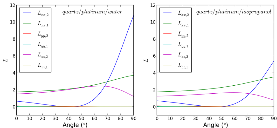
Figure 3.8: The calculated Fresnel factors for (left) the quartz/platinum/water system and (right) the quartz/platinum/isopropanol system. L_1 is the Fresnel factor for the quartz/platinum interface and L_2 the factor for the platinum/liquid interface.
