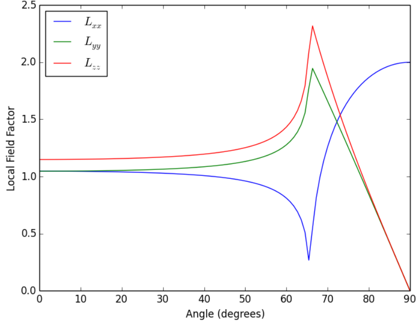
Figure 2.3: The real part of the local field factors for the quartz/water interface ( n_{\text{quartz}} = 1.46 , n_{\text{water}} = 1.33 , n_{\text{interface}} = 1.33 ) as a function of the incident angle using the thin layer model. The L here are most representative of those for the visible and SFG pulse in SFG experiments.
