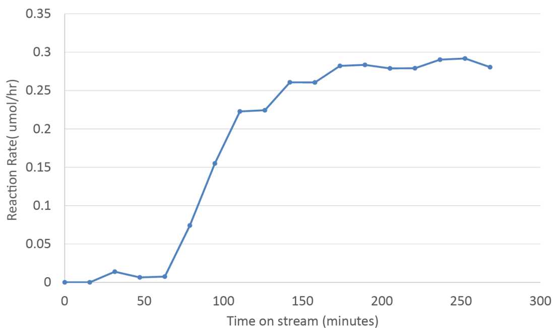
Figure 6.1: Reaction rates for ethanol oxidation to acetaldehyde as measured in the flow mode. The induction period exists in the first 60 minutes of reaction, followed by an increase in the acetaldehyde production rate. Conditions: 217 mM ethanol in water, 160 \mu\text{M} \text{O}_2 , 30 ^\circ\text{C} .
