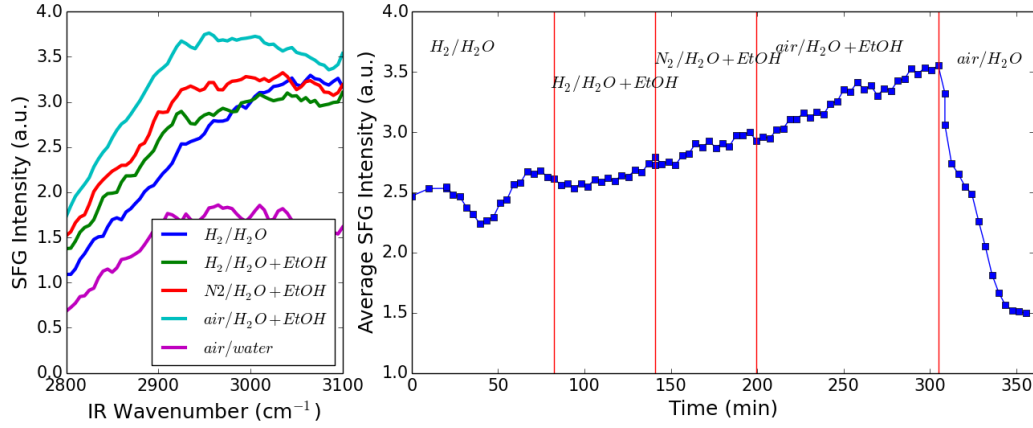
Figure 6.7: Left: Non-resonant SFG spectra of platinum under conditions of H 2 /H 2 O, H 2 /Ethanol, N 2 /Ethanol, O 2 /Ethanol, and O 2 /H 2 O. Right: The averaged signal for the SFG spectra under aforementioned conditions. Apparently neither water nor ethanol affects the non-resonant signal, but exposure to oxygen immediately causes the decrease in the signal similar to what is seen under reaction conditions.
