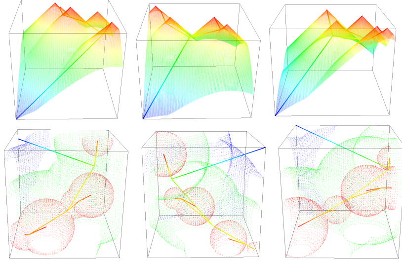
Fig. 7 Analytical functions. Rendering with embedded merge tree of three 2D functions f_1, f_2, f_3 (first row), and three 3D functions f_4, f_5, f_6 (second row).
