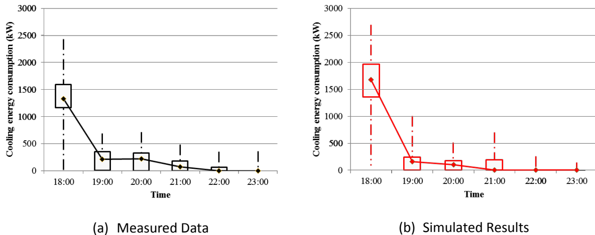
Fig. 17. The interquartile profile of the hourly cooling energy consumption during overtime on weekdays for the whole cooling season: (a) Measured data; (b) Simulated results from the model with overtime.
