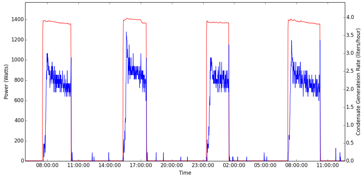
Figure 16 Typical Compressor Cycles and Condensate Removal Rate Time Series for Site WHD-SiteB03
