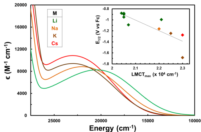
Figure 5. Electronic absorption spectra showing ligand to metal charge transfer (LMCT) absorption features of \text{Ce}^{\text{IV}}\text{MB} , \text{M} = \text{Li}, \text{Na}, \text{K}, \text{Cs} . 2-Cl (green), 4-BINOL (orange), 6-BINOL (brown), and 8 (red). (Inset) Plot of E_{1/2} vs LMCT max for 2 , 4 , 6 , and 8 .
