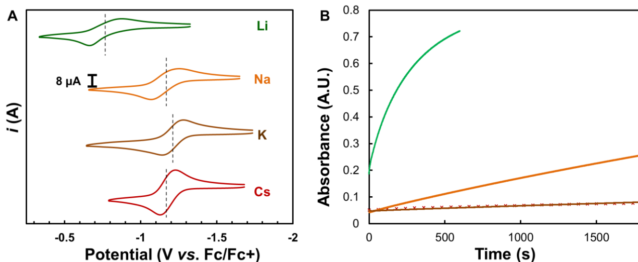
Figure 6. (A) Cyclic voltammograms measured for CeMB ( M = \text{Li} ( 1 ), \text{Na} ( 3 ), \text{K} ( 5 ), and \text{Cs} ( 7 )) in THF: \text{CH}_3\text{CN} (1:6) using a 3 mm diameter glassy carbon working electrode; v = 50 \text{ mV/s} ; [\text{Ce}] \approx 1 \text{ mM} ; [\text{NPr}_4][\text{BAR}_4^{\text{F}}] \approx 0.1 \text{ M} . Dashed lines drawn to illustrate positions of E_{1/2} . (B) Pseudo-first order rate data for 1 , 3 , 5 , and 7 in THF using UV-Vis absorption spectroscopy; [\text{Ce}]:[\text{Ph}_3\text{CCl}] = 1:10 . 1 (green), 3 (orange), 5 (brown), 7 (red).
