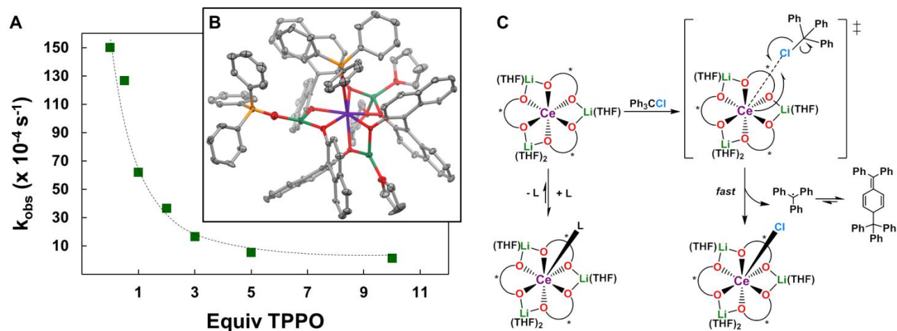
Figure 7. (A) k_{\text{obs}} under pseudo-first order kinetics (1:10 [1]:Ph 3 CCl) in toluene in the presence of varying equivalents of TPPO (dotted line drawn as a guide for the eye). (B) Thermal ellipsoid plot of 1-2TPPO, with ellipsoids shown at 30% probability. (C) Proposed inner sphere mechanism for the oxidation of 1 with trityl chloride.
