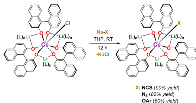
Scheme 2. Salt metathesis reactions of [\text{Li}_3(\text{THF})_5]_3[(\text{BINOLate})_3\text{Ce}-\text{Cl}]\cdot\text{THF} , 2-Cl .
