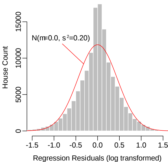
Figure 14 Regression residuals of 134,000 houses in ResDB. The normal distribution with the observed mean ( \mu ) and variance ( \sigma^2 ) is indicated by the red line.
