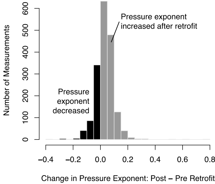
Figure 13 Change in pressure exponent after retrofit of 1800 homes.
