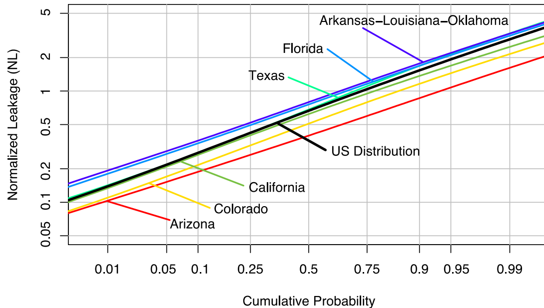
Figure 16 Estimated distribution of NL for single-family detached homes in US and in selected states.
