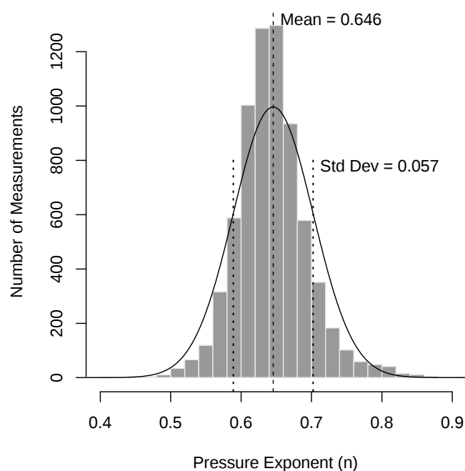
Figure 2 Distribution of pressure exponents from approximately 7,000 multi-point blower door measurements. The normal distribution is plotted using the observed mean and standard deviation as indicated by the dotted lines.
