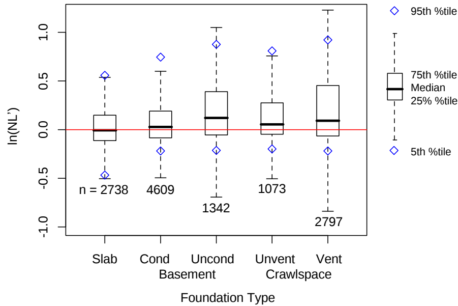
Figure 10 Model residuals of NL for homes with known foundation types (n = number of houses).
