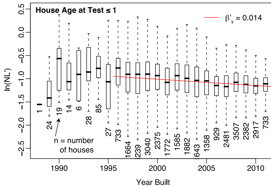
Figure 9 Coefficient estimate of year built, \beta_y (per year), for new homes built within 1 year on the date of test.
