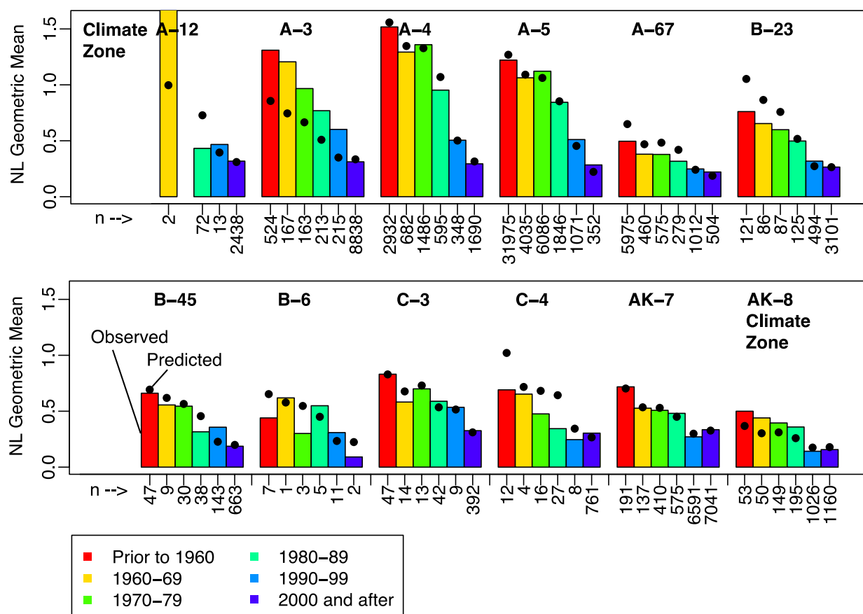
Figure 15 Comparison of observed and predicted geometric mean of NL for houses of different vintages and climate zones (n = number of homes).
