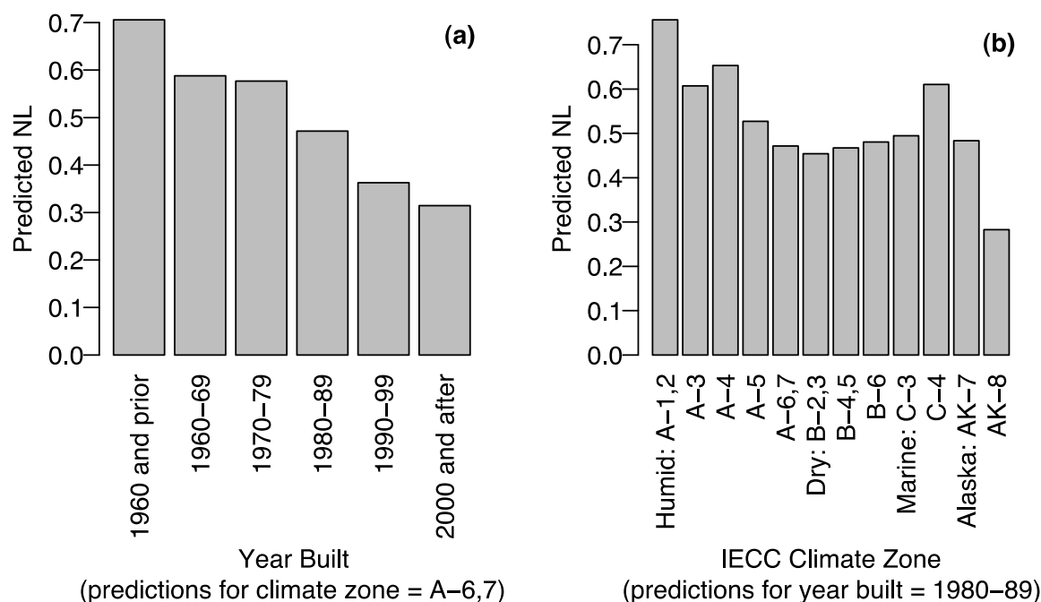
Figure 6 Normalized leakage (NL) predicted by the core regression model: (a) for homes as a function of year built and (b) in different climate zones. Predictions are made based on a one-story (height = 3 m) house with floor area = 150 m².
