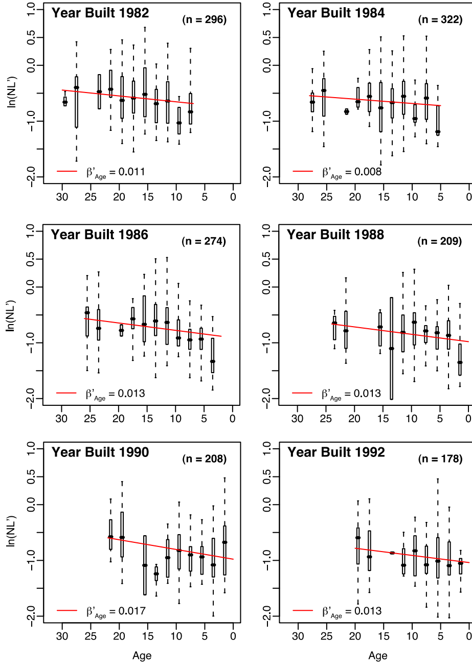
Figure 8 Coefficient estimates of house age at test, \beta'_{\text{Age}} , for houses built between 1982 and 1992 ( n = number of homes).
