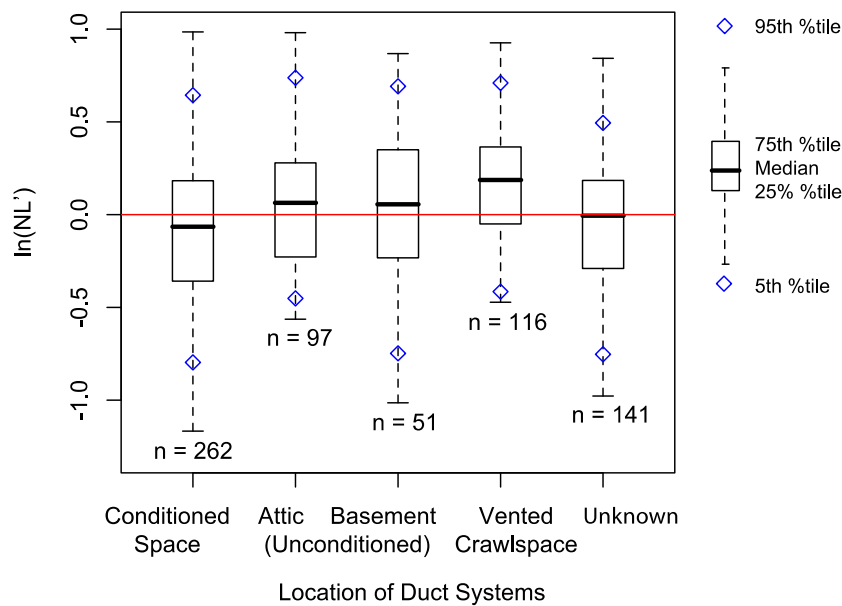
Figure 11 Model residuals of NL for homes from Home Energy Score pilot program where duct locations were indicated (n = number of houses).
