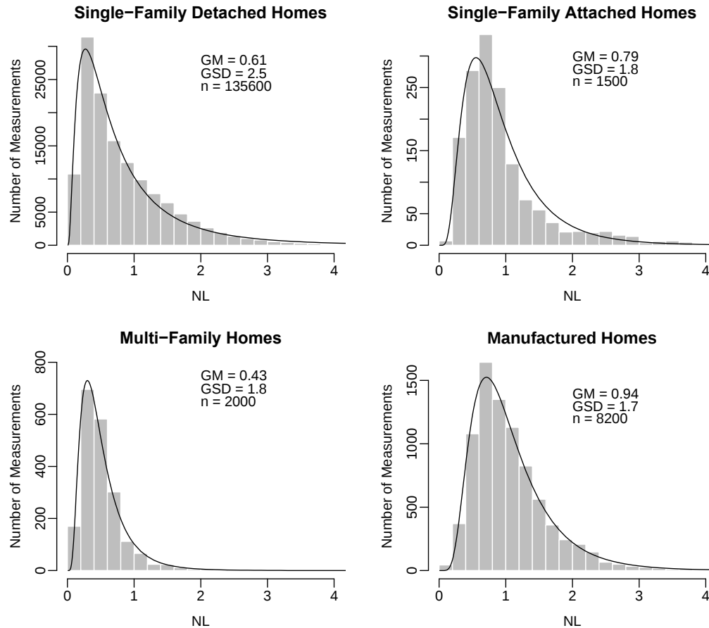
Figure 1 Histograms of normalized leakage (NL) of homes in ResDB. The geometric mean (GM) and geometric standard deviation (GSD) of NL are shown for each home type ( n = number of homes). The log-normal distribution, as described by the GM and GSD, is overlaid on top of the histogram.
