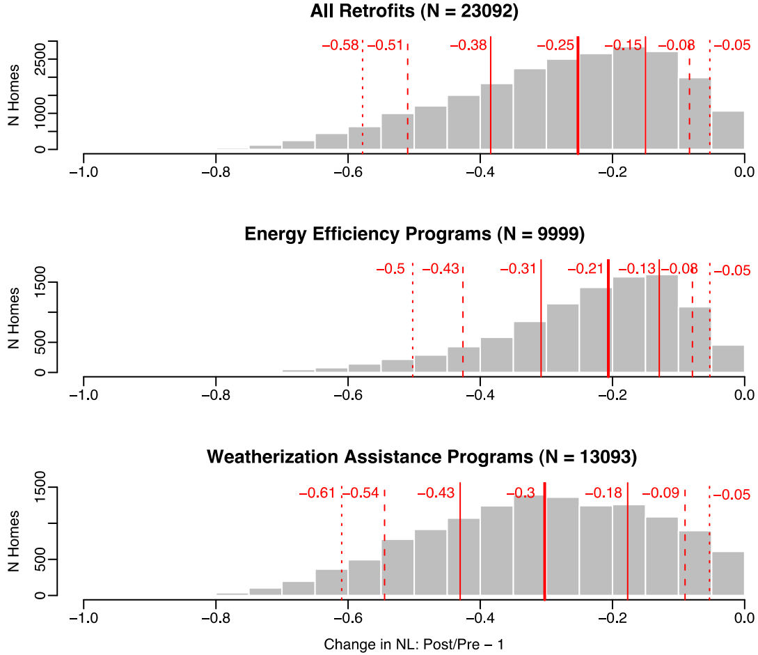
Figure 12 Improvements from retrofit as quantified by the reduction in NL. Summary statistics of the change in NL are indicated in red (from left to right): 5 th , 10 th , 25 th , 50 th , 75 th , 90 th , and 95 th percentiles.
