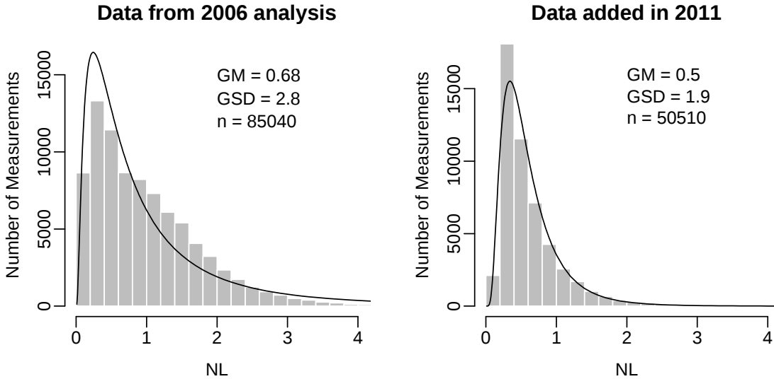
Figure 4 Histograms of normalized leakage (NL) of single-family detached homes analyzed previously in 2006 ResDB and recently collected in 2011. The geometric mean (GM) and geometric standard deviation (GSD) of NL are shown (n = number of houses). The log-normal distribution, as described by the GM and GSD, is overlaid on top of the histogram.
