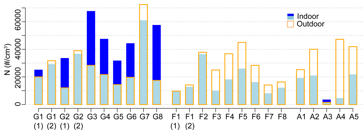
Figure 12 Average ultrafine particle counts measured in grocery (G), furniture/hardware (F), and apparel (A) stores. Darker blue shows the portion of indoor particles that exceeded the outdoor levels. Stores G1, G2, and F1 were sampled on two days: (1) and (2).
