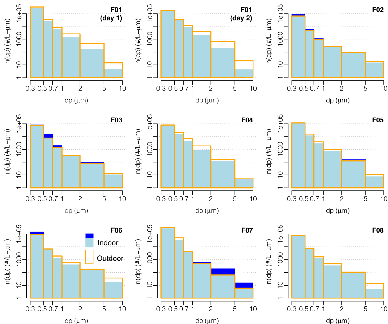
Figure 10 Number distributions of particles between 0.3 and 10 μm measured in eight furniture/ hardware stores. Darker blue shows the portion of indoor particles that exceeded the outdoor levels.
