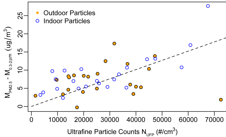
Figure 14 Relationship between the ultrafine particle counts measured by WCPCs (x-axis) and the predicted mass of particles <0.3 \mu\text{m} (y-axis). A total of 48 data points are shown here, including 21 store visits, and three stores (G1, G2, and F1) sampled for two days.
