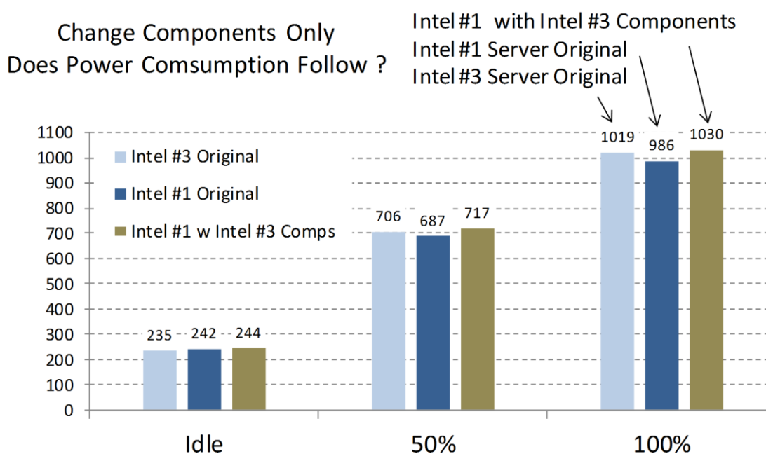
Figure 3-4: Intel Server Power Using One Set of Nodes
