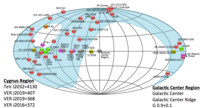
Figure 2: Left) The VERITAS sky catalog in Galactic coordinates. The different colored objects represent different classes of sources and the blue region is that visible to VERITAS.
