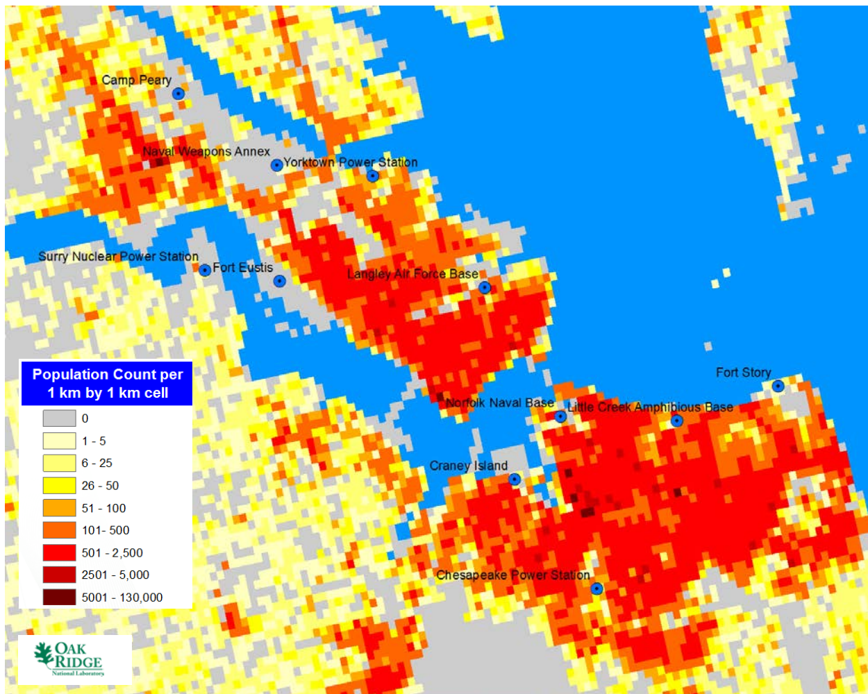
Fig. 4. Regional population density by cell (orange and red indicate higher population density).
