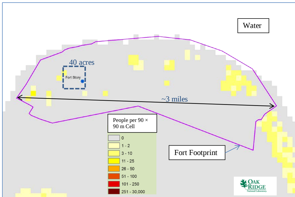
Fig. 19. Landsat™ daytime population near Fort Story.
