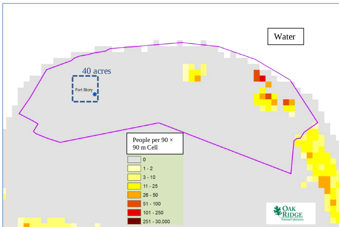
Fig. 20. Landsat™ nighttime population near Fort Story.
