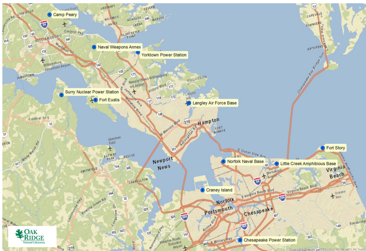
Fig. 1. Regional view of evaluated Hampton Roads sites.
