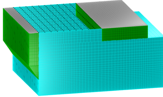
Figure 1-13: Wetted surface geometry modeled with cosine spacing in MultiSurf. Dipole panels (cyan), conventional body panels (green), interior surfaces for irregular frequency removal (gray). Black points illustrate the interior field point locations.
