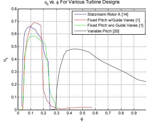
Figure 1-25: Wells turbine efficiency vs. flow coefficient for various turbine designs.
