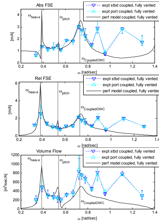
Figure 1-15: Experimental verification of \omega_{\text{CoupledOWC}} through RAOs of absolute FSE, relative FSE, and volume flow for a fully vented BBDB.
