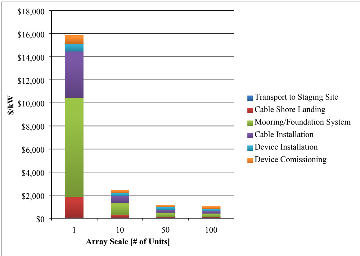
Figure 1-35: Installation cost breakdown ($/kW) per deployment scale.
