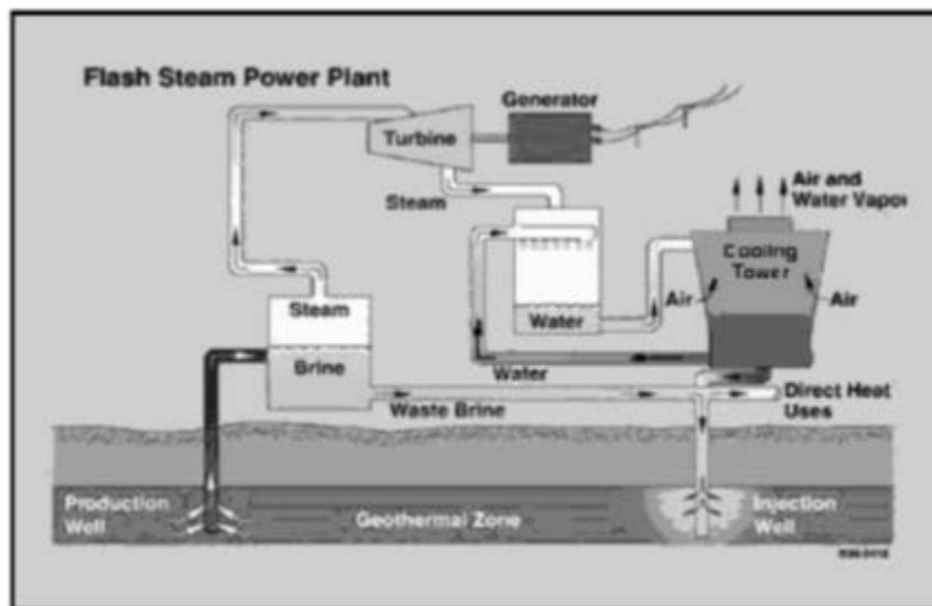
Figure 50. Flash Power Plant
