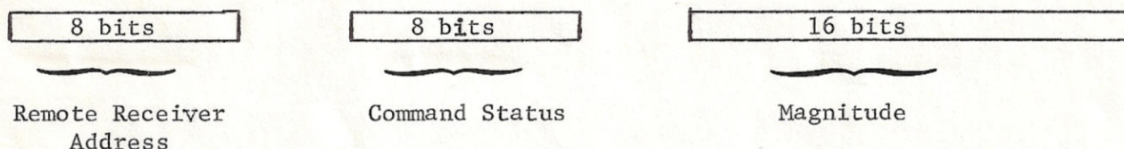
FIGURE 1 Datacom Word Format
