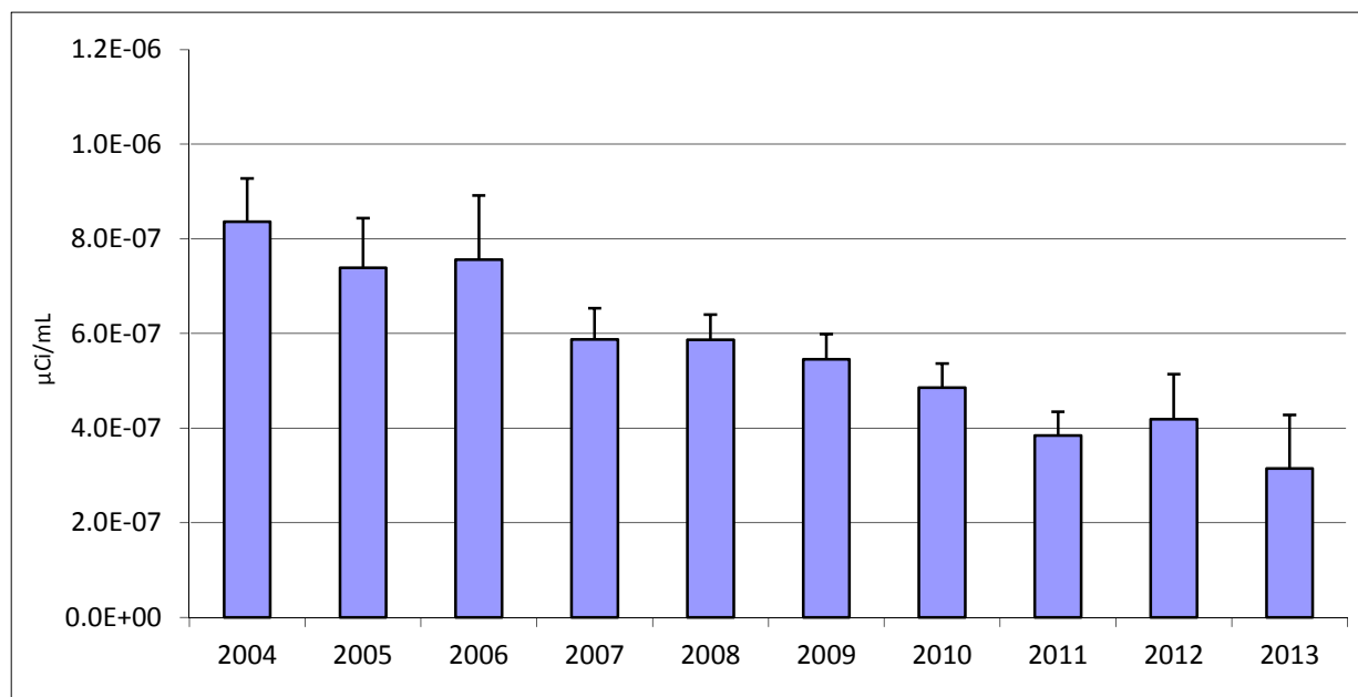
FIGURE 2-2 Average Concentration of Tritium in Surface Water at WNNADR: 2004-2013
