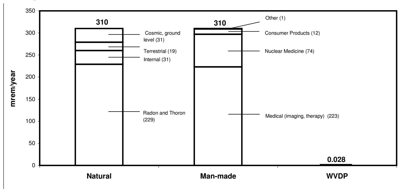
Comparison of Doses From Natural and Man-Made Sources to the Dose From 2013 WVDP Effluents
