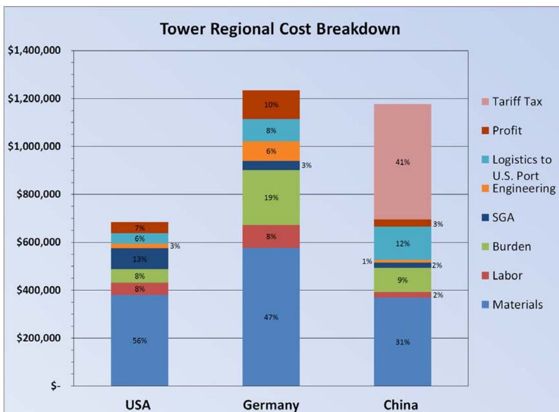
Fig. 1.1.3b Aggregated Regional Cost Breakdown in %
