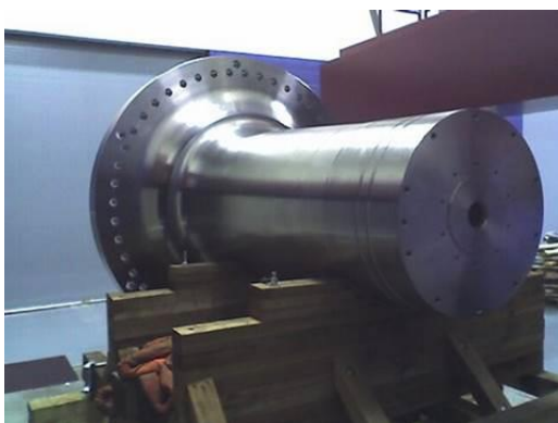
Fig. 2.12.2 Machine shaft 45,000 lb., 15' long and 8' diameter. McSwain Manufacturing, Ohio.
