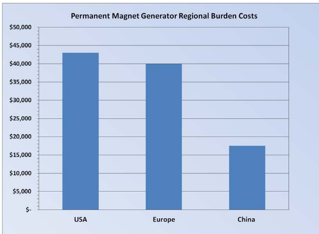
Fig. 1.3.11 Burden Regional Cost Breakdown (1MW PM Generator)
