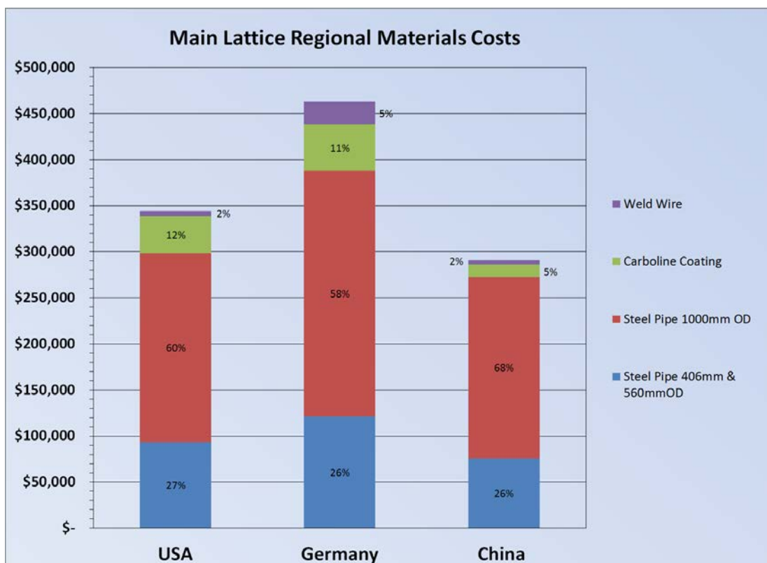
Fig. 1.4.4b Materials Regional Cost Breakdown in %
