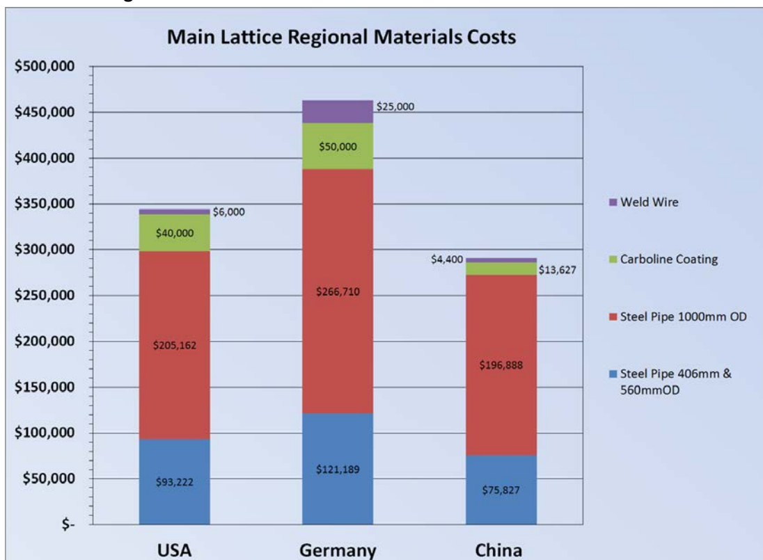
Fig. 1.4.4a Materials Regional Cost Breakdown in $
