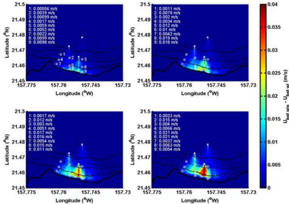
Figure 15. Evaluation of the effects of an obstacle array on the nearshore bottom orbital velocity. The model initiation parameters were: MWD = 0°; T_p = 10 s; and H_s = 1 m (upper left), 2 m (upper right), 3 m (lower left), and 4 m (lower right). The bold line denotes the shoreline and contour lines for 10 m, 20 m, 30 m, and 40 m are shown.
