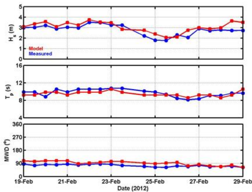
Figure 3. SWAN model validation results for Mokapu Point. Model data are shown in red and measured CDIP Station 098 data are shown in blue.
