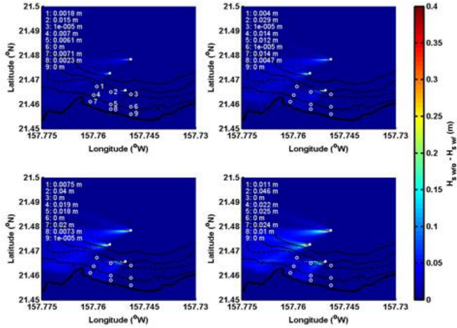
Figure 14. Same caption as Figure 11 but for MWD = 90°.
