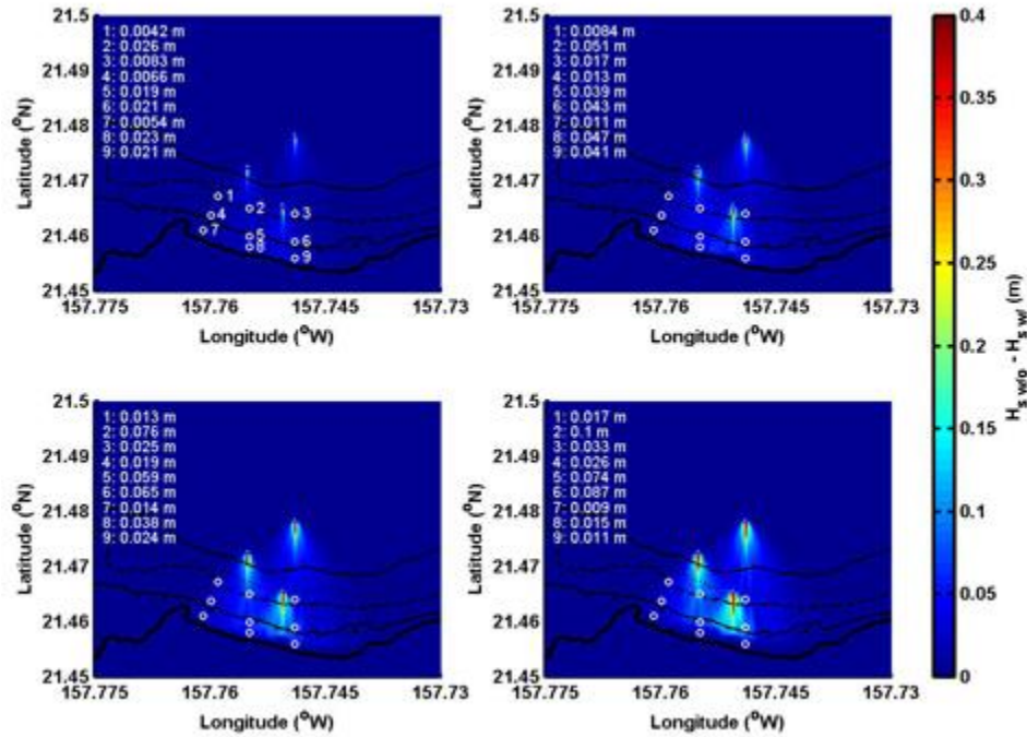
Figure 11. The effects of an obstacle array on the nearshore study area (obstacles – white squares – are not to scale). The model initiation parameters were: MWD = 0°; T_p = 10 s; and H_s = 1 m (upper left), 2 m (upper right), 3 m (lower left), and 4 m (lower right). The bold line denotes the shoreline and contour lines for 10 m, 20 m, 30 m, and 40 m are shown. Model output locations are indicated by white circles and are numbered in the upper left panel. The differences between SWAN simulated H_s without and with obstacles for each output location are indicated.
