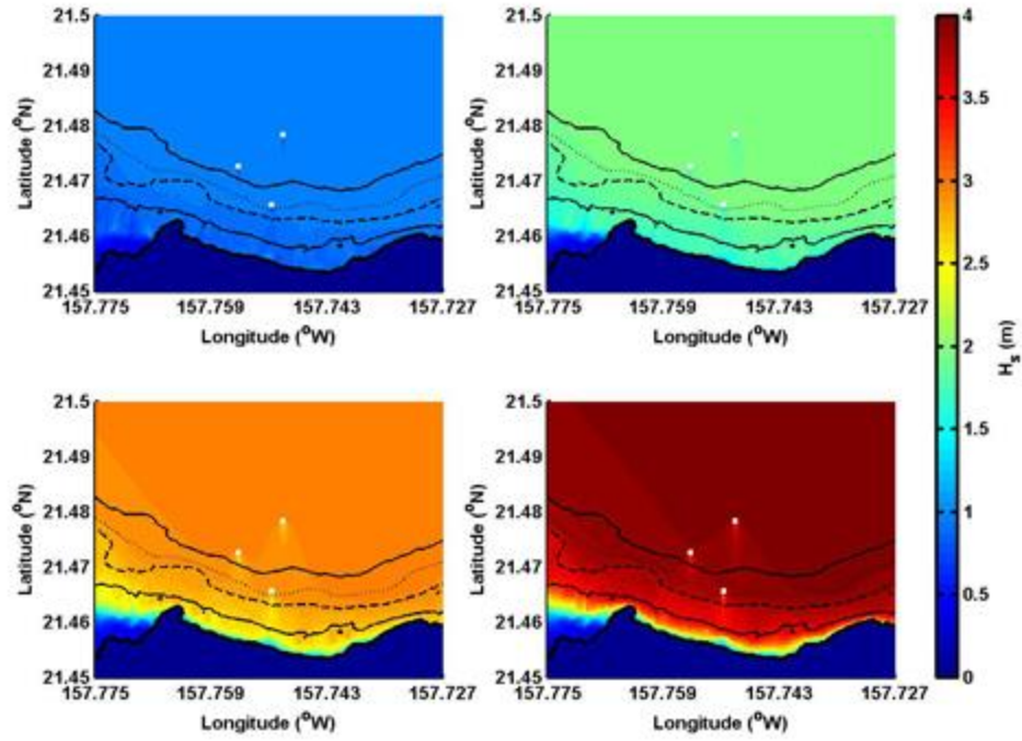
Figure 4. SWAN simulated significant wave height with model initiation parameters: MWD = 0^\circ ; T_p = 6 s; and H_s = 1 m (upper left), 2 m (upper right), 3 m (lower left), and 4 m (lower right). The bold line denotes the shoreline and contour lines for 10 m, 20 m, 30 m, and 40 m are shown. The model obstacles, shown as white squares, are not to scale.
