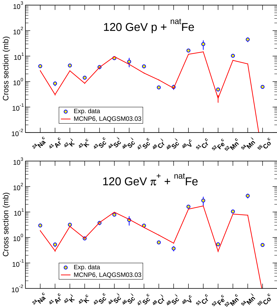
Figure 13: Detailed comparison between all cross section measured in Ref. [32] from interaction of 120 GeV protons and positive pions with ^{\text{nat}}\text{Fe} (filled circles) and those calculated by MCNP6 using the LAQGSM03.03 event-generator (red lines), as indicated.
