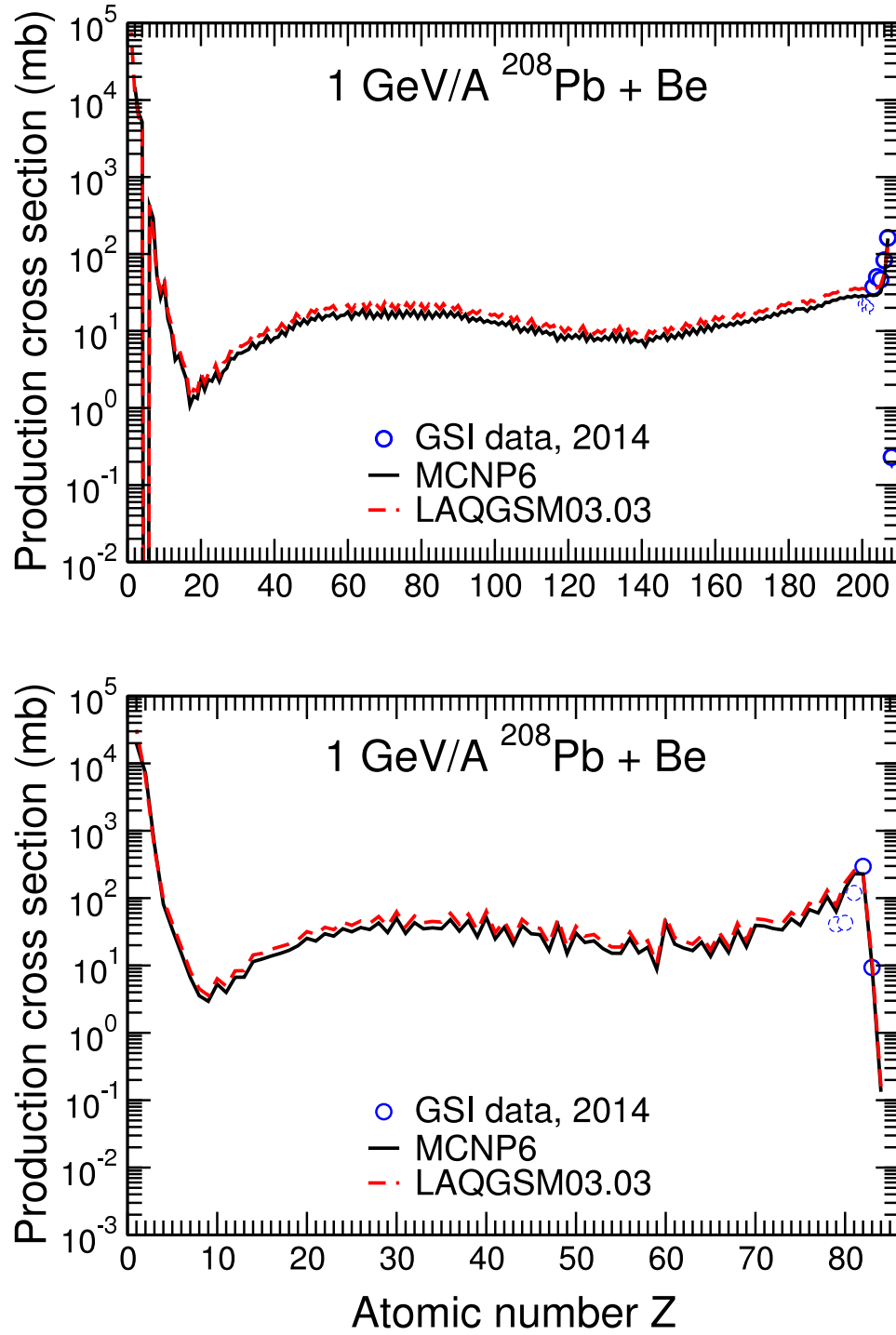
Figure 11: Comparison of calculated by MCNP6 and bf LAQGSM03.03 used as a stand alone code A - and Z -distributions of all products from the reaction 1 \text{ GeV/nucleon } ^{208}\text{Pb} + ^9\text{Be} with a rough estimate of several experimental values for such characteristics obtained summing the measured [31] (symbols) yields of only a neutron-rich part of all products (see more details in the text) from this reaction, as indicated.
