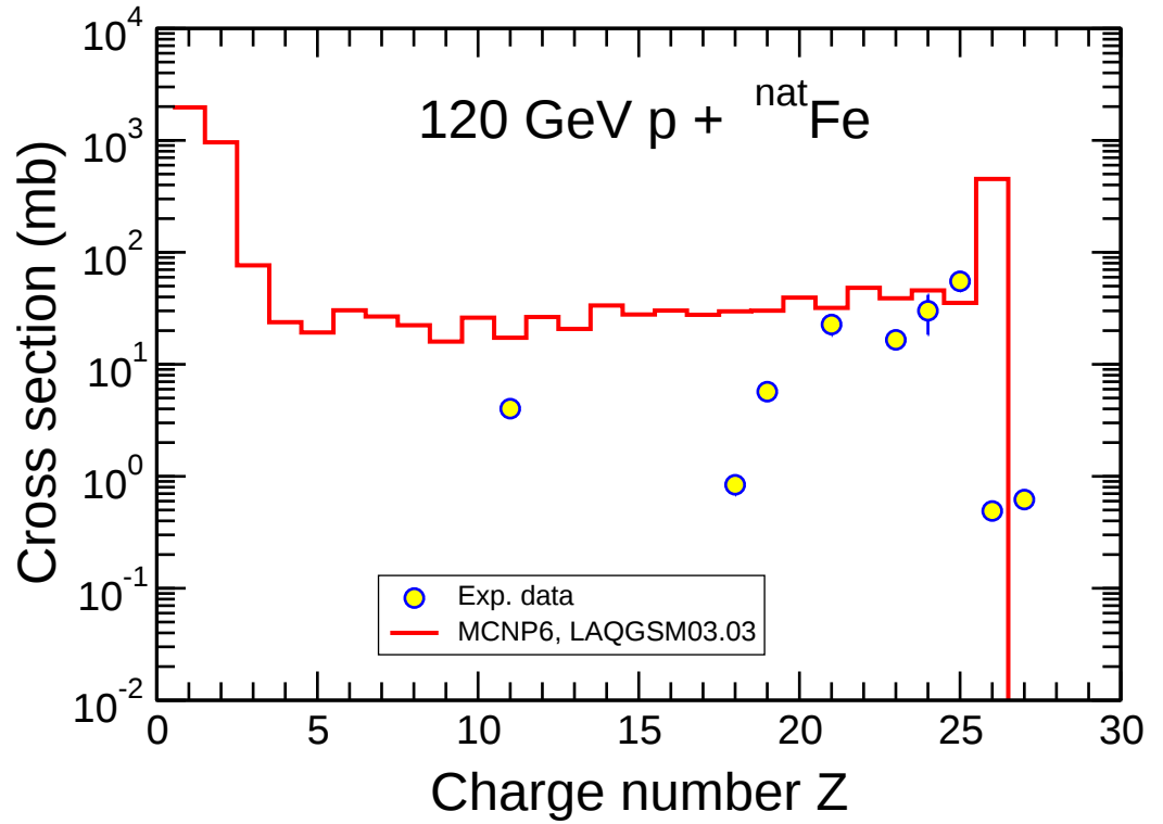
Figure 14: Experimental mass- and charge-number distributions of yields of all products measured in Ref. [32] from the 120 GeV p + ^{nat}\text{Fe} reaction (filled circles) compared with results by MCNP6 using the LAQGSM03.03 event-generator (red histograms), as indicated.
