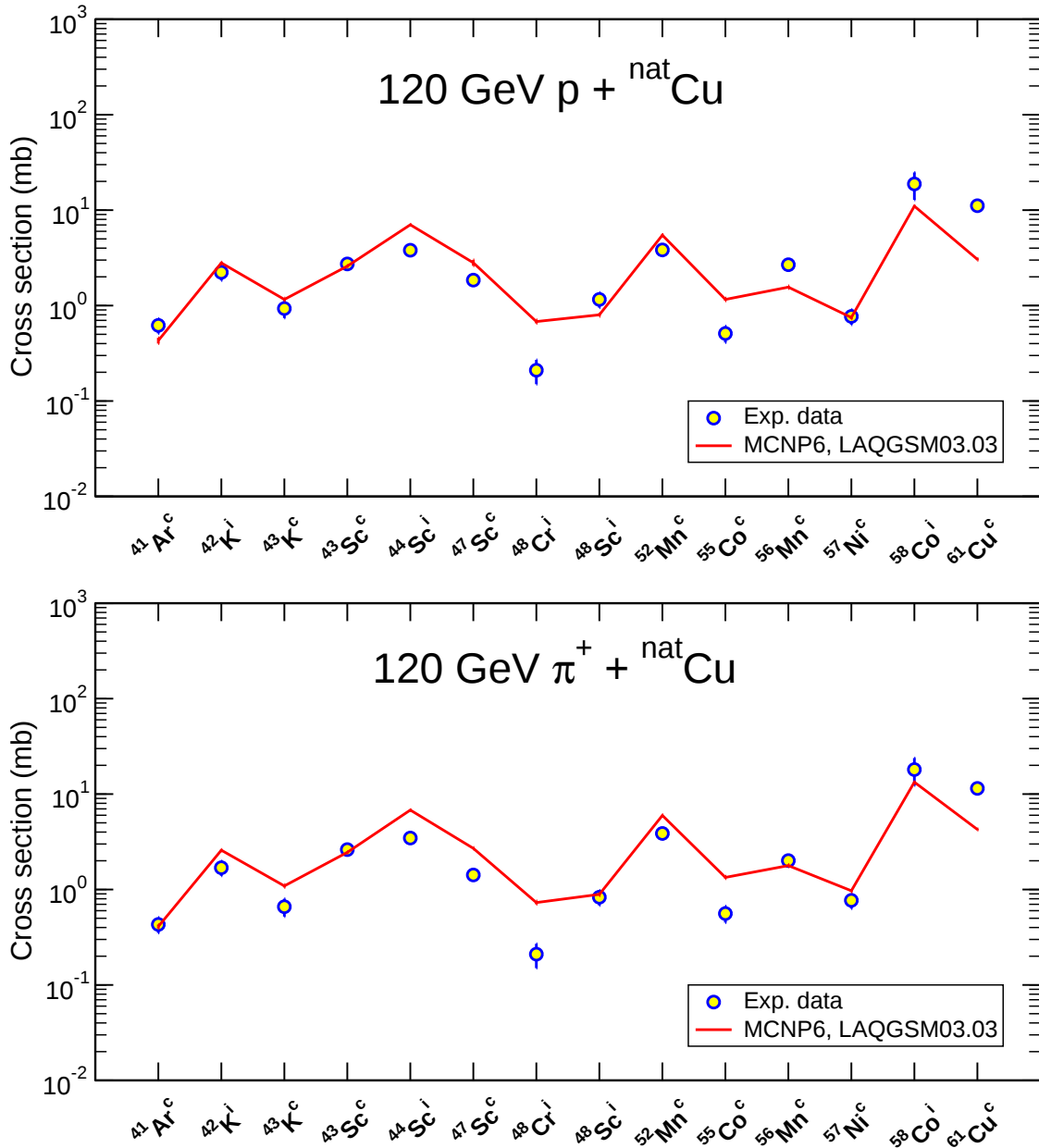
Figure 12: Detailed comparison between all cross section measured in Ref. [32] from interaction of 120 GeV protons and positive pions with ^{\text{nat}}\text{Cu} (filled circles) and those calculated by MCNP6 using the LAQGSM03.03 event-generator (red lines), as indicated.
