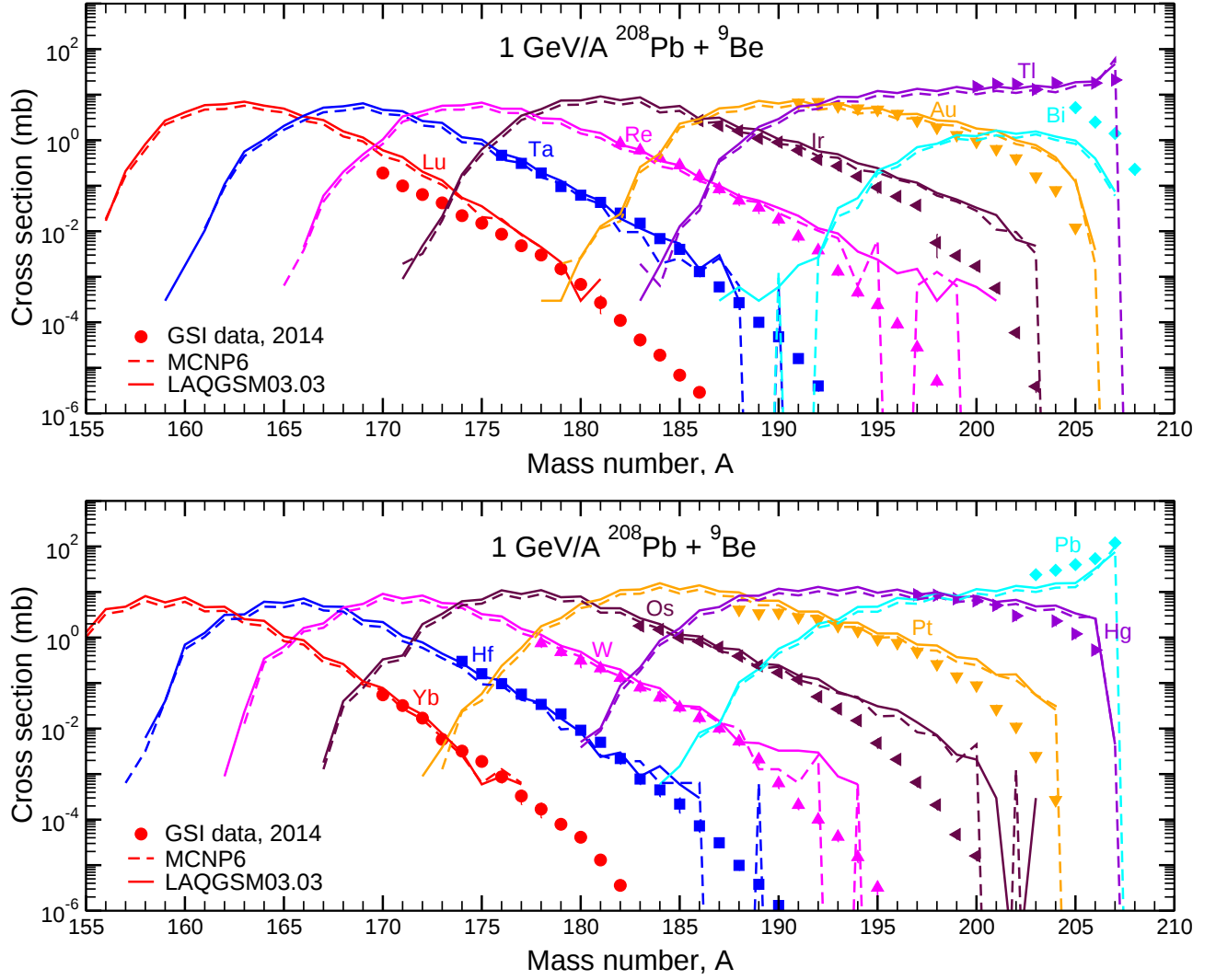
Figure 10: Experimental mass number distribution of yields of products with Z from 70 to 83 [31] (symbols) from the 1 \text{ GeV/nucleon } ^{208}\text{Pb} + ^9\text{Be} reaction compared with results by LAQGSM03.03 [9, 27] used as a stand alone code (color solid lines) and by MCNP6 using the LAQGSM03.03 event-generator (color dashed lines), as indicated.
