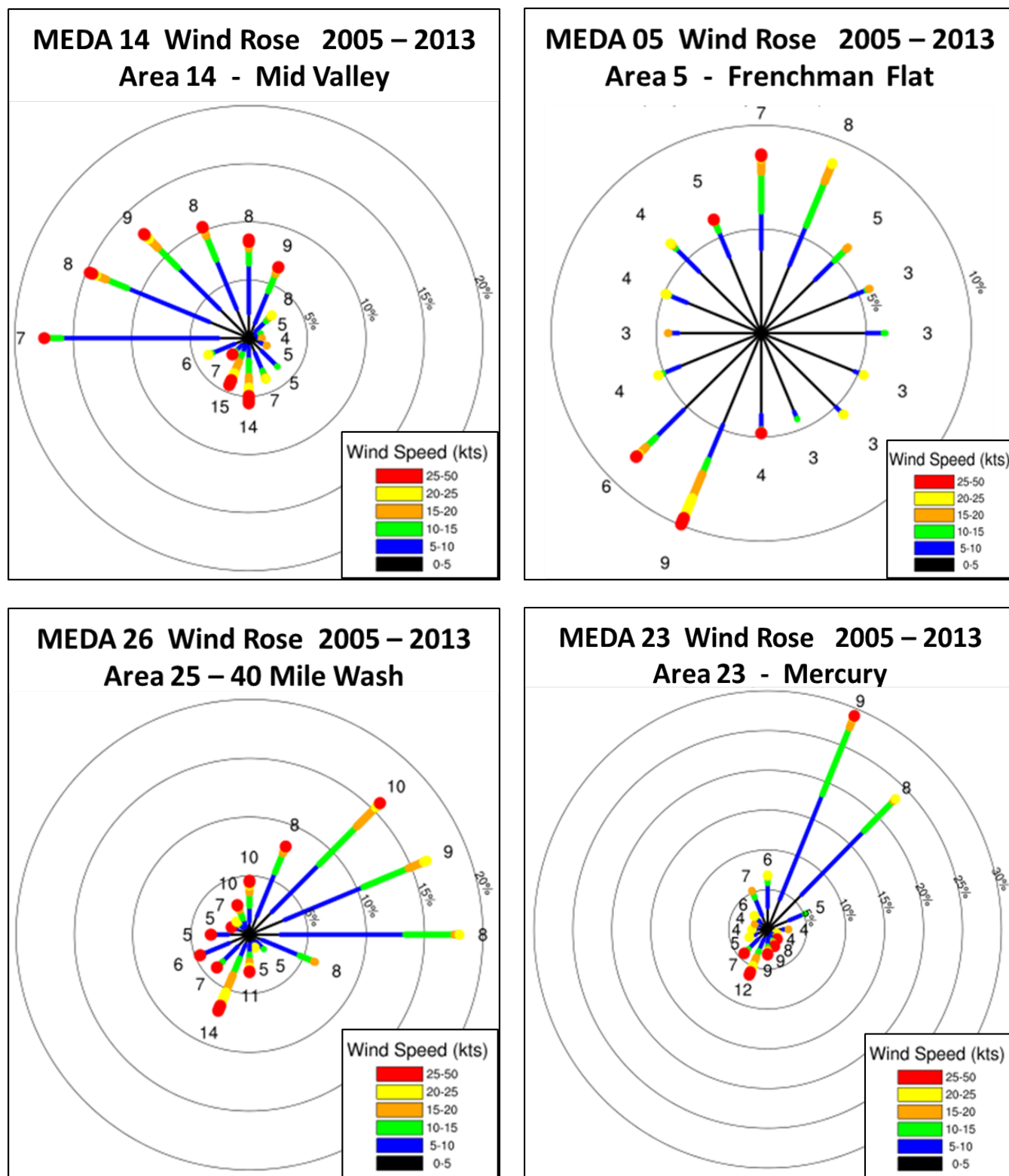
Figure A-17b. Wind rose climatology for the NNSS
