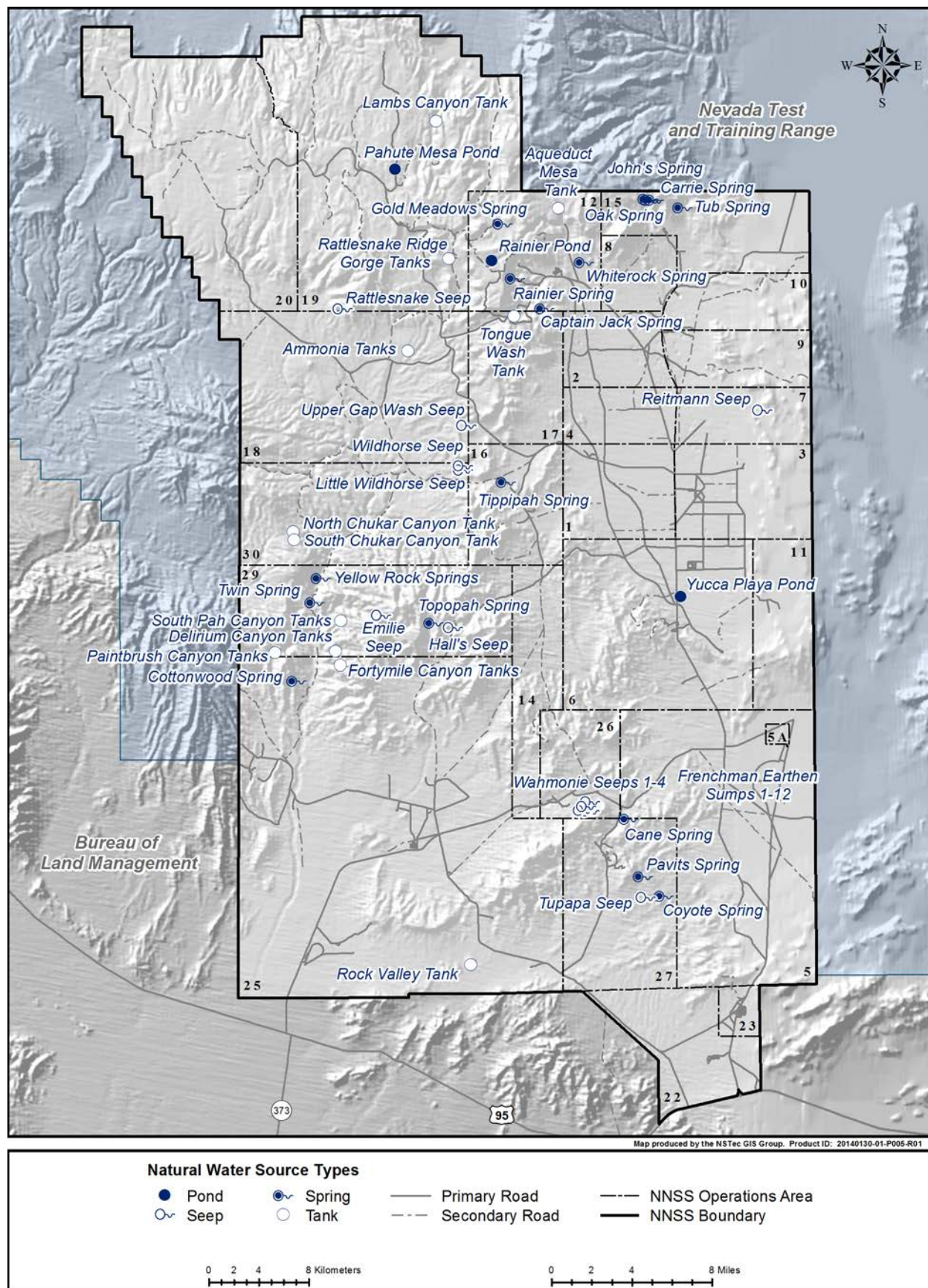
Figure A-20. Natural water sources on the NNSS (from Hall et al. 2014)
