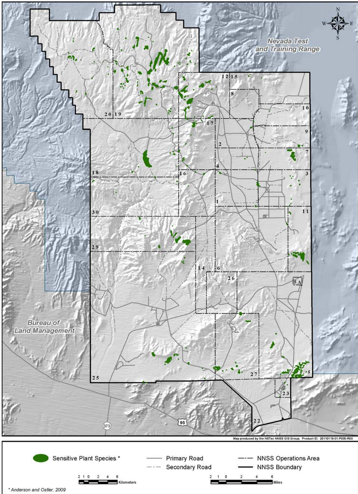
Figure A-19. Known locations of sensitive plant species on the NNSS (from Anderson and Ostler [2009])
