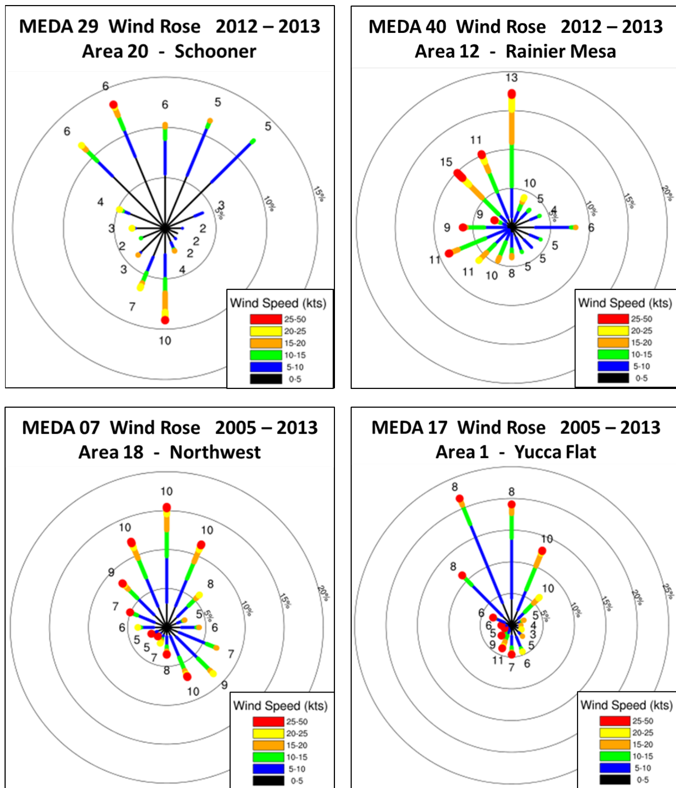
Figure A-17a. Wind rose climatology for the NNSS
