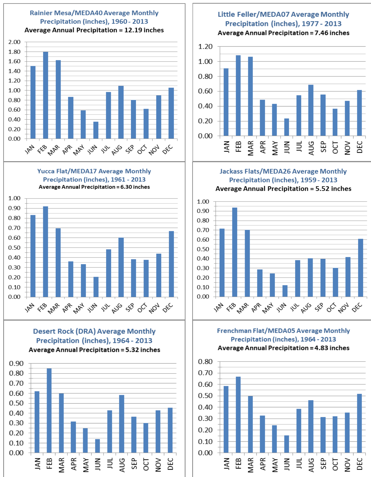
Figure A-15. Mean monthly precipitation at six NNSS rain gauge stations
