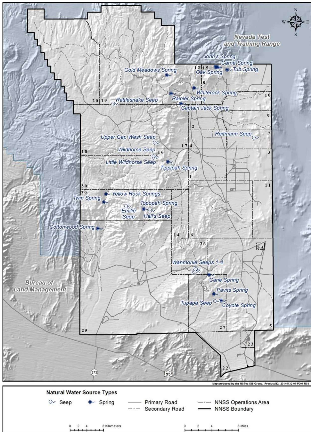
Figure A-4. Natural springs and seeps on the NNSS (adapted from Hall et al. 2014)
