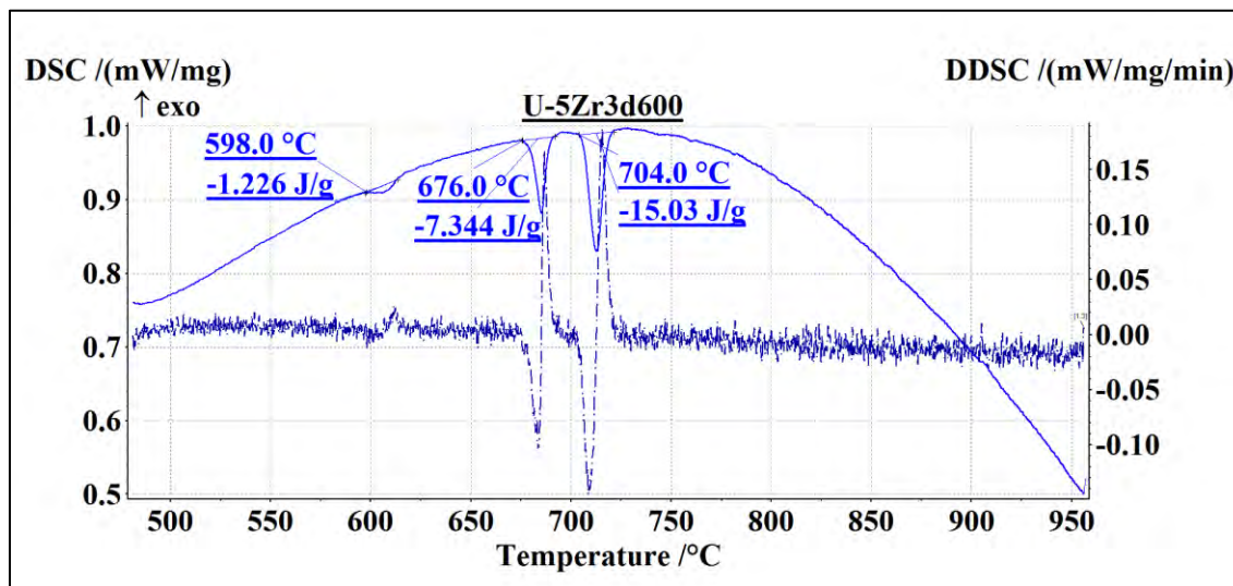
(a) U-5Zr3d600
