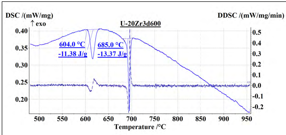
(a) U-20Zr3d600
