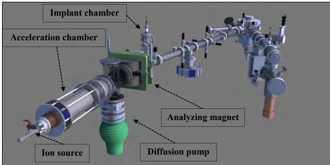
Figure 3-5: Schematic of a 140 keV accelerator used for \text{He}^+ ion-beam irradiation (figure courtesy of Michael Justinn General, Texas A&M University).
