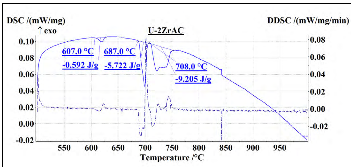
(b) U-2ZrAC
