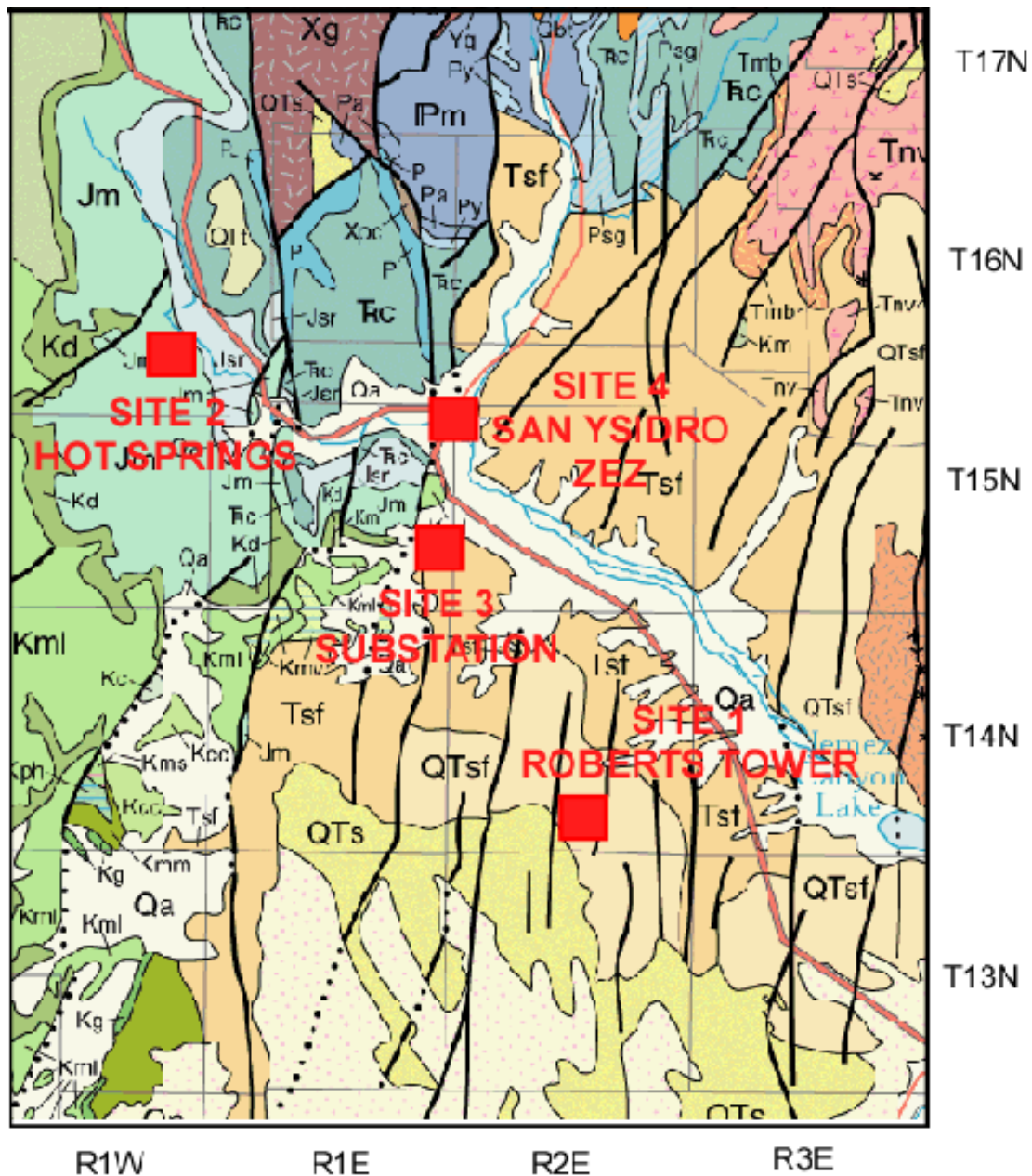
Figure 3. Geologic map of the Pueblo of Zia region. The brown hatched area in the northwest part of the map represents Precambrian basement (granite and metamorphic rocks) in the Nacimiento Mountains. The blue and green colors represent Paleozoic (blue) and Mesozoic (green) sedimentary formations. Units with labels P, Pa, Py, Psg and in part Trc represent the "redbed" sandstone reservoir targets buried at depth at the sites. The brown, orange, yellow, and cream colors are sediments and volcanic rocks, filling the Albuquerque basin of the Rio Grande rift. Bold black lines are fault zones. (Geology from NMBGMR).
