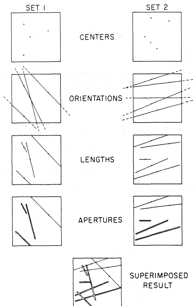
Fig. 3. Superposition of random sets of fractures.
