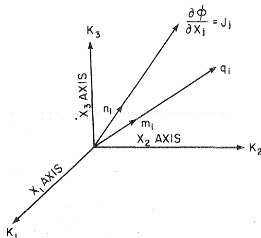
Fig. 1. General flow conditions in anisotropic media.
