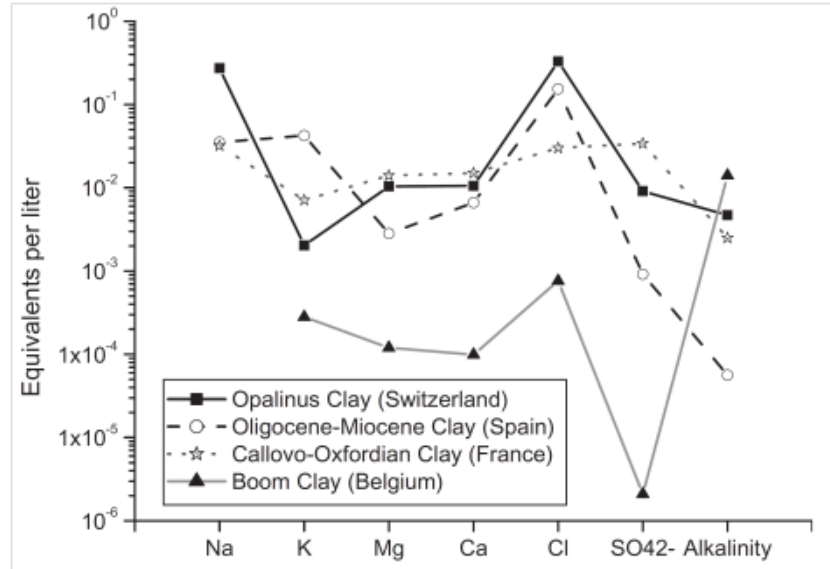
Figure 11. Composition of pore-waters in different argillaceous formations (from Turrero et al. 2006)
