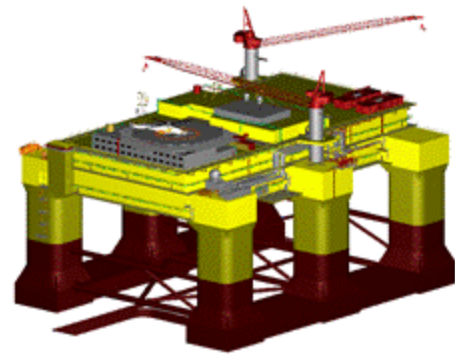
Figure 5-44. Example GBS platform
