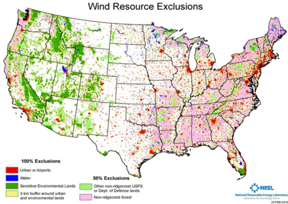
Figure 2-3. Wind resource exclusions
