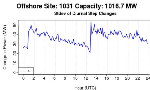
Figure 3-9. Standard deviation of diurnal mean 10-minute ramps in net power (MW) at a sample site
