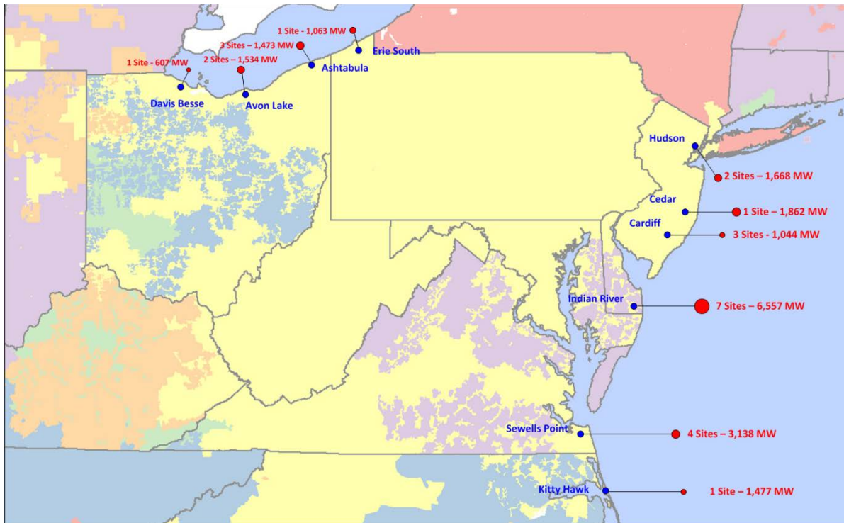
Figure 6-28. Map of wind site locations and onshore interconnections—PJM
