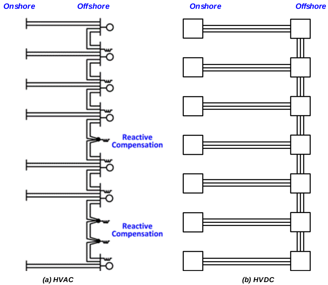
Figure 6-18. Offshore wind delivery system—backbone connection
