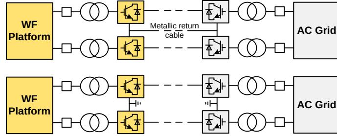
Figure 6-4. Bipolar HVDC connections
