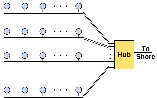
Figure 5-9 Offshore wind farm collection system with single-sided ring configuration
