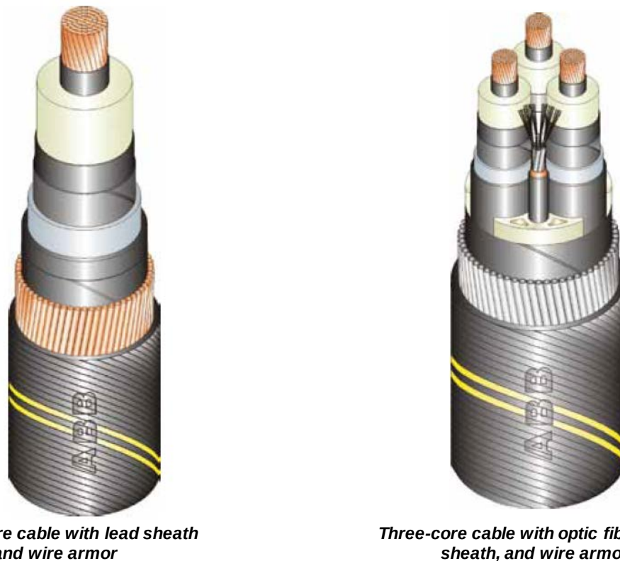
Figure 5-38. Single-core and three-core XLPE armored cables (Illustrations from ABB)
