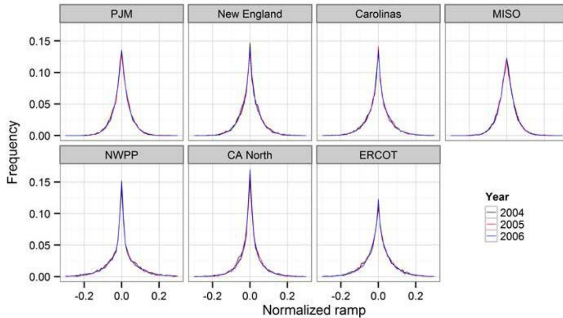
Figure 4-8. Normalized hourly ramp distributions for all three years
