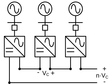
Figure 5-12 Series DC collection network
