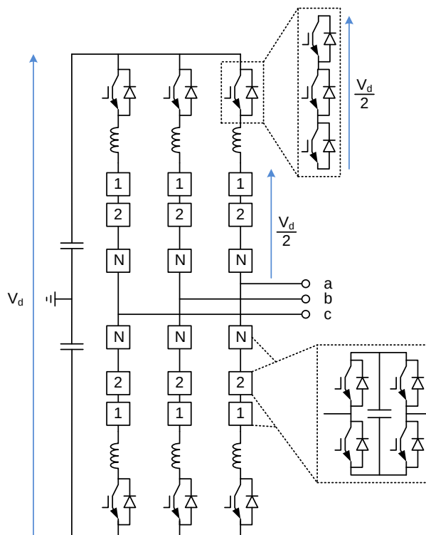
Figure 5-32. A series hybrid circuit, also known as an AAM converter
