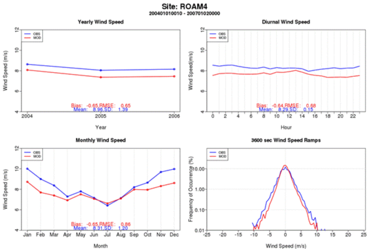
Figure 3-8. As in Figure 3-6, but for Rock of Ages, Minnesota.
