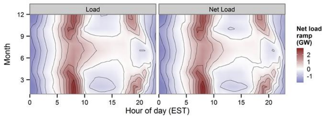
Figure B-11. Contour plots showing average load and net load ramp by month and hour of day for NWPP
