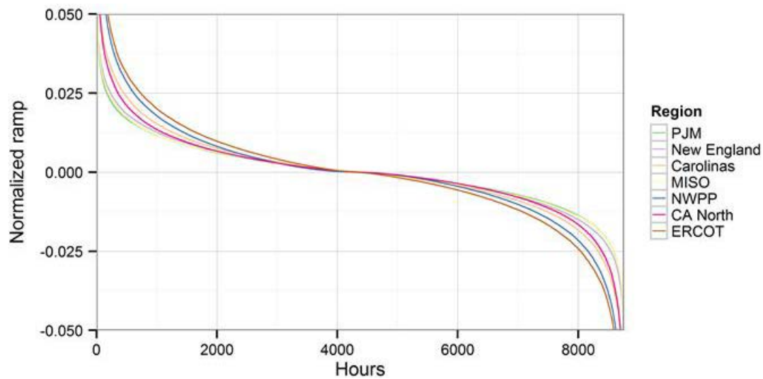
Figure 4-17. Normalized 10-minute ramp duration curves for 2006
