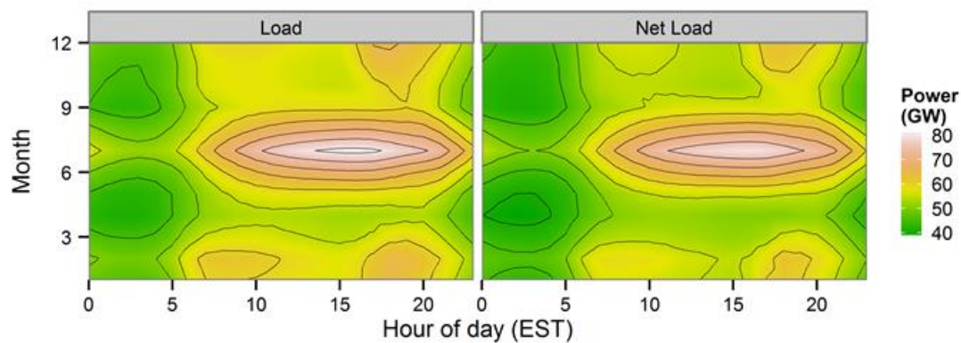
Figure B-6. Contour plots showing average load and net load by month and hour of day for MISO
