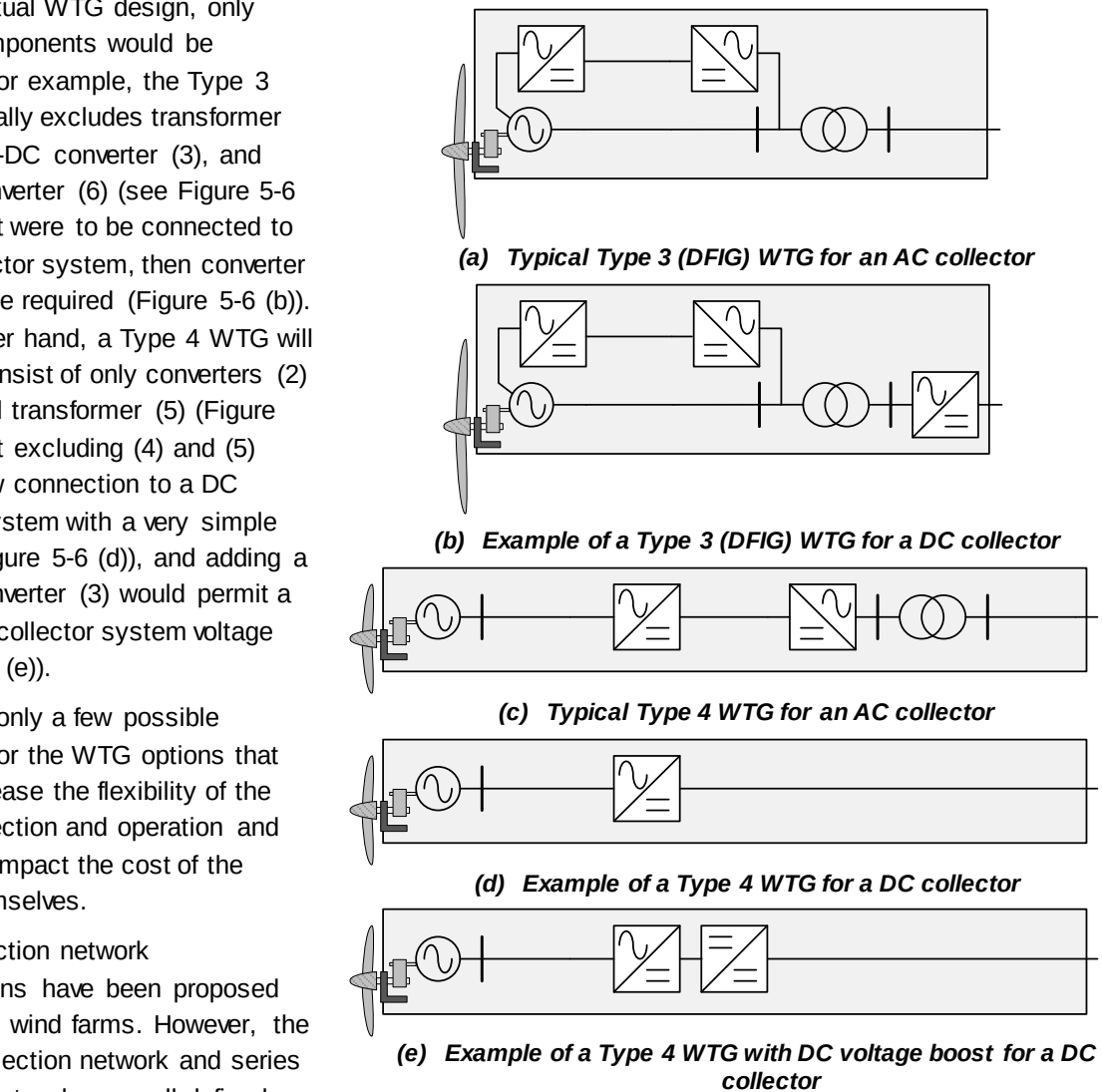
Figure 5-6. Example WTG topology options
