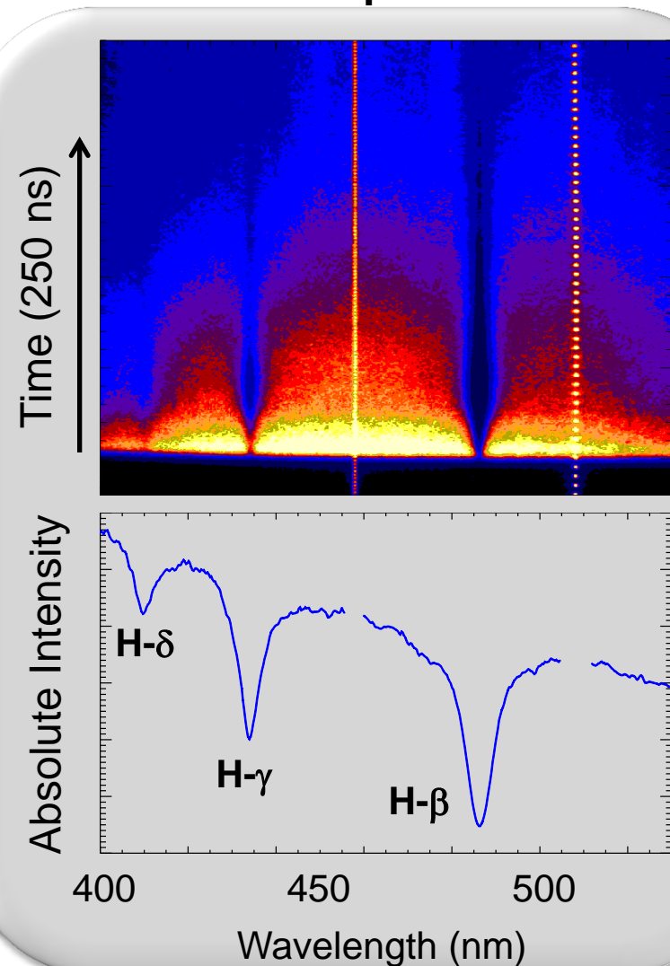
Absorption
