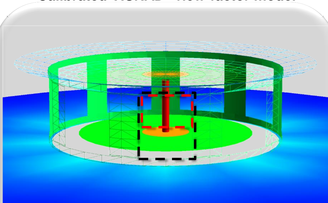
Calibrated VISRAD* view-factor model
