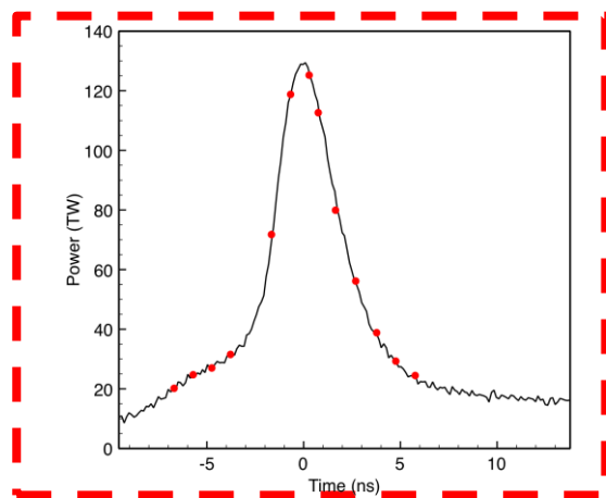
Absolute Power Measurements
