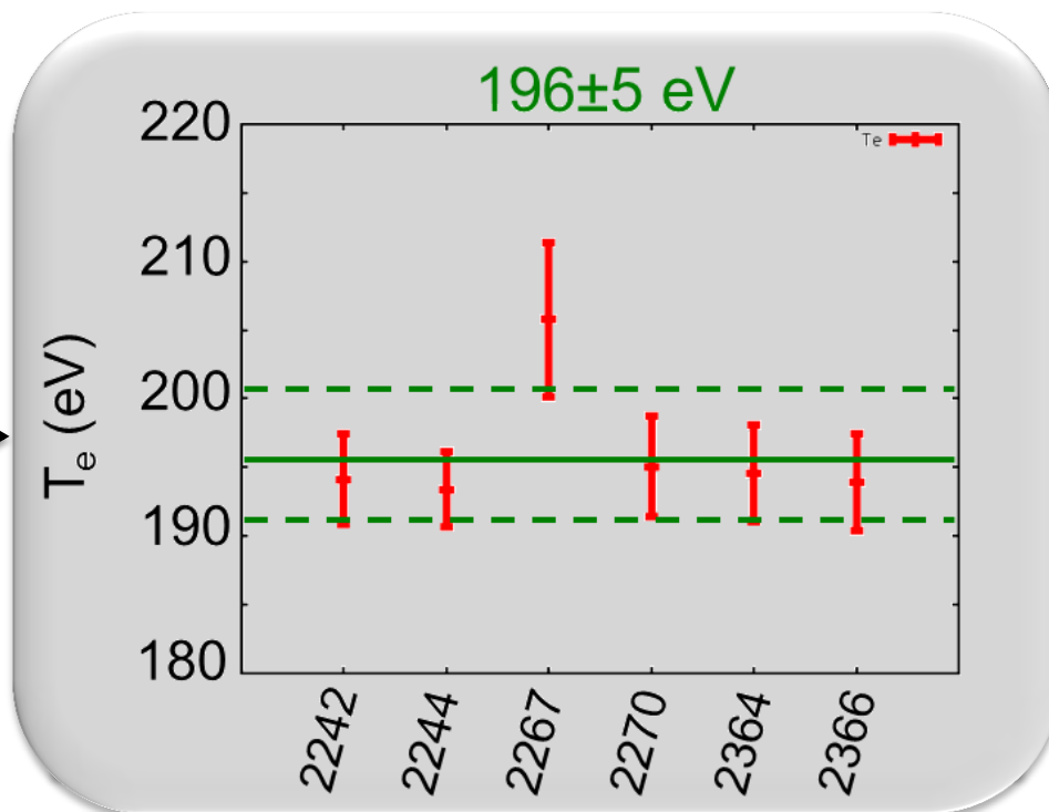
Axial Fe Foil Temperature
