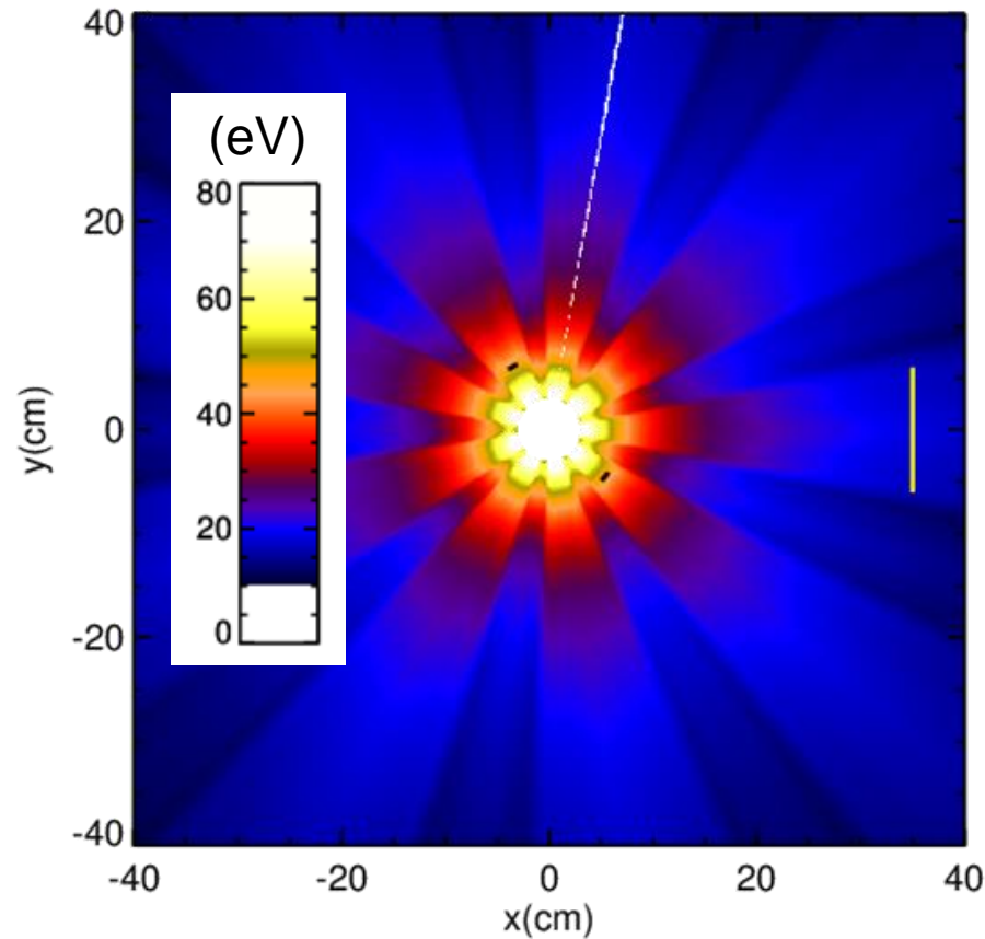
r- \theta Peak Brightness Temperature Contours
