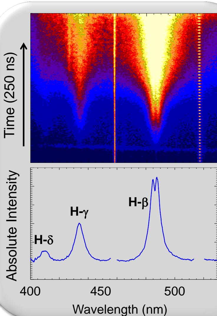
Emission
