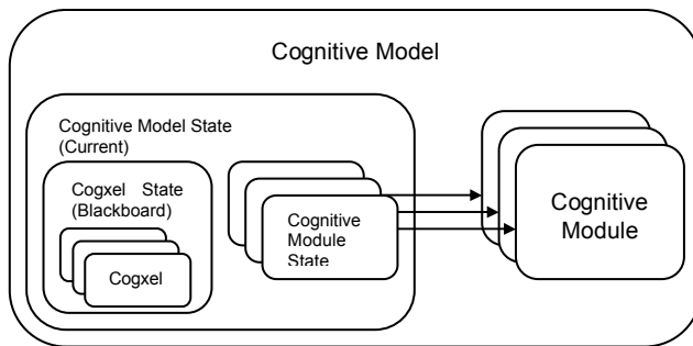
Figure 1. Cognitive Model components. One object encapsulates the entire state of the model. The design emphasizes modularity and state encapsulation.
