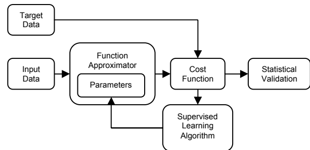
Figure 2. Typical supervised learner design pattern.
