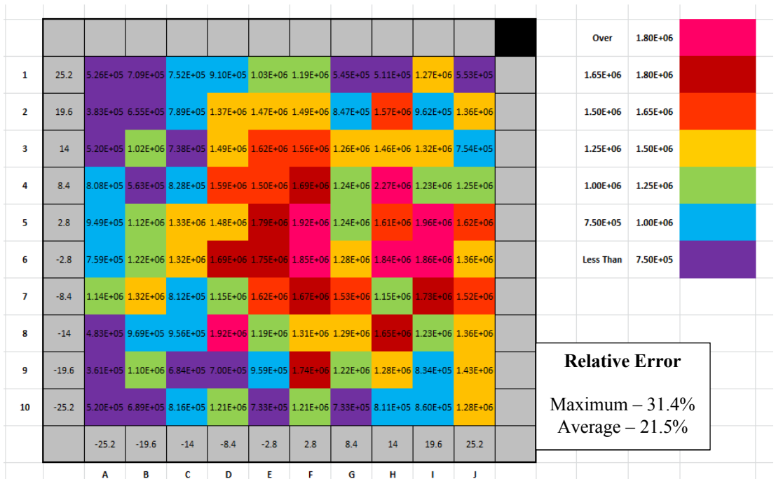
Figure 6 - 250:1 Aperture – Total Neutron Flux Calculated from MCNP Meshtally
