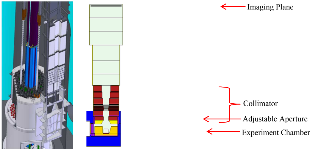
Figure 1 - Solid Works and MCNP Models of the ACRR Neutron Radiography System
