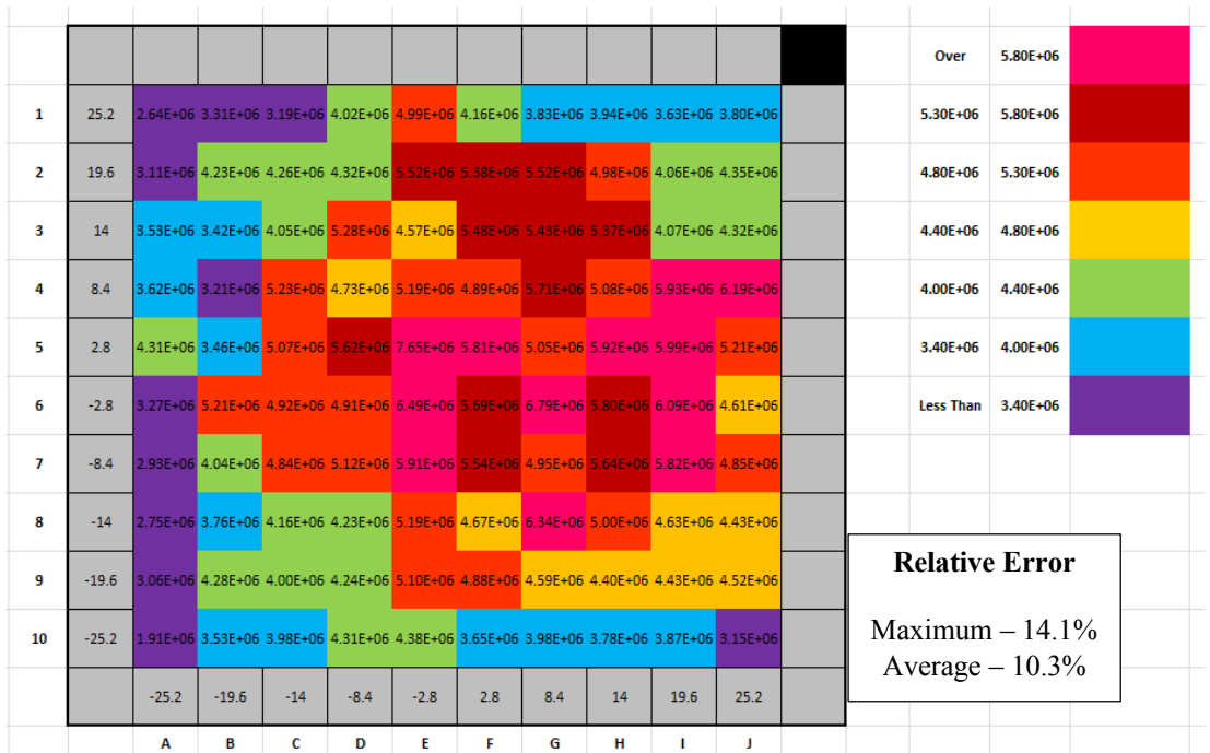
Figure 5 - 125:1 Aperture – Total Neutron Flux Calculated from MCNP Meshtally
