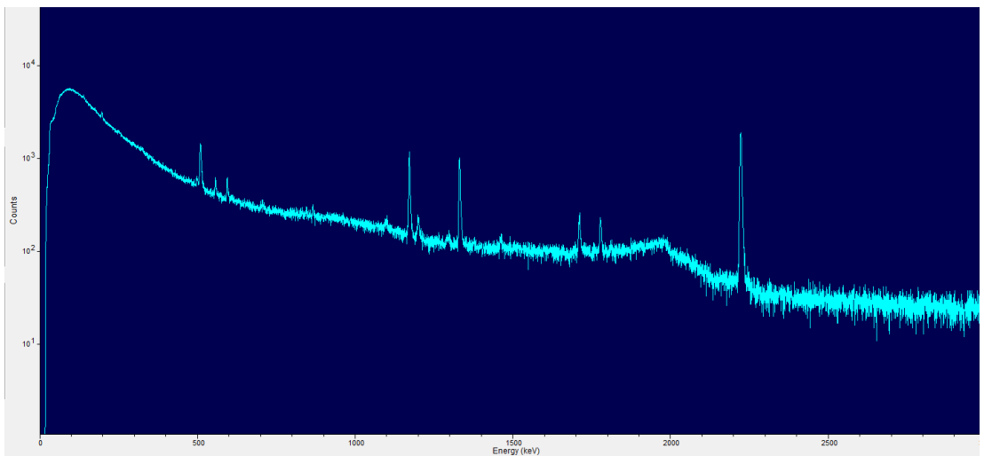
Figure 3 - HPGe Gamma Spectrum
