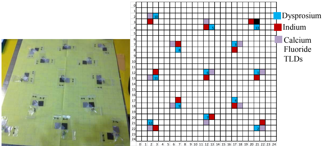
Figure 2 – Aluminum Plate with Dosimetry and Corresponding Foil Pattern
