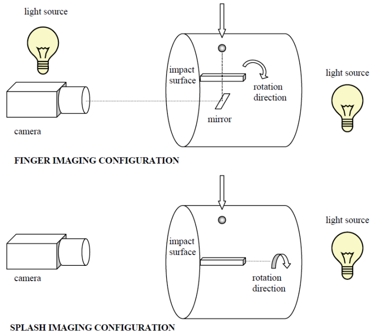
Figure 1. Camera and lighting configurations for splash (lateral) and finger (vertical) imaging.
