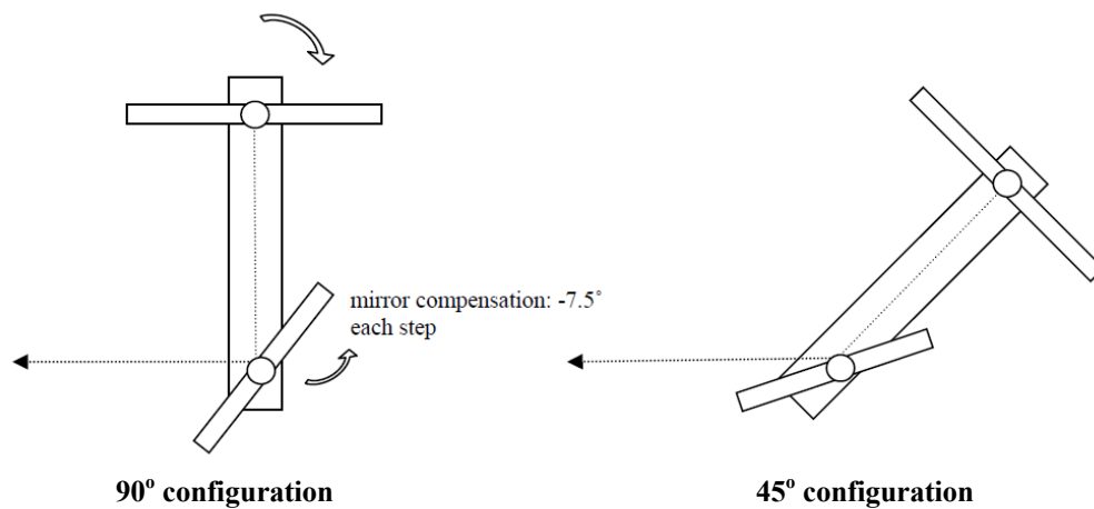
Figure 2. Impact surface and mirror configurations for finger imaging.
