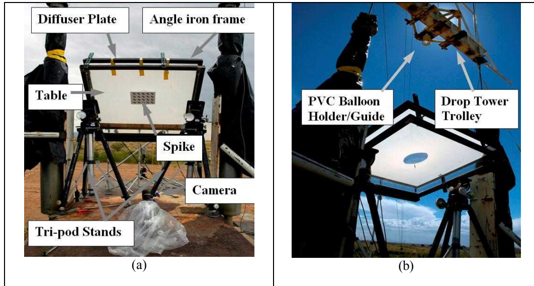
Figure 3. Experimental setup for large scale impact testing.
