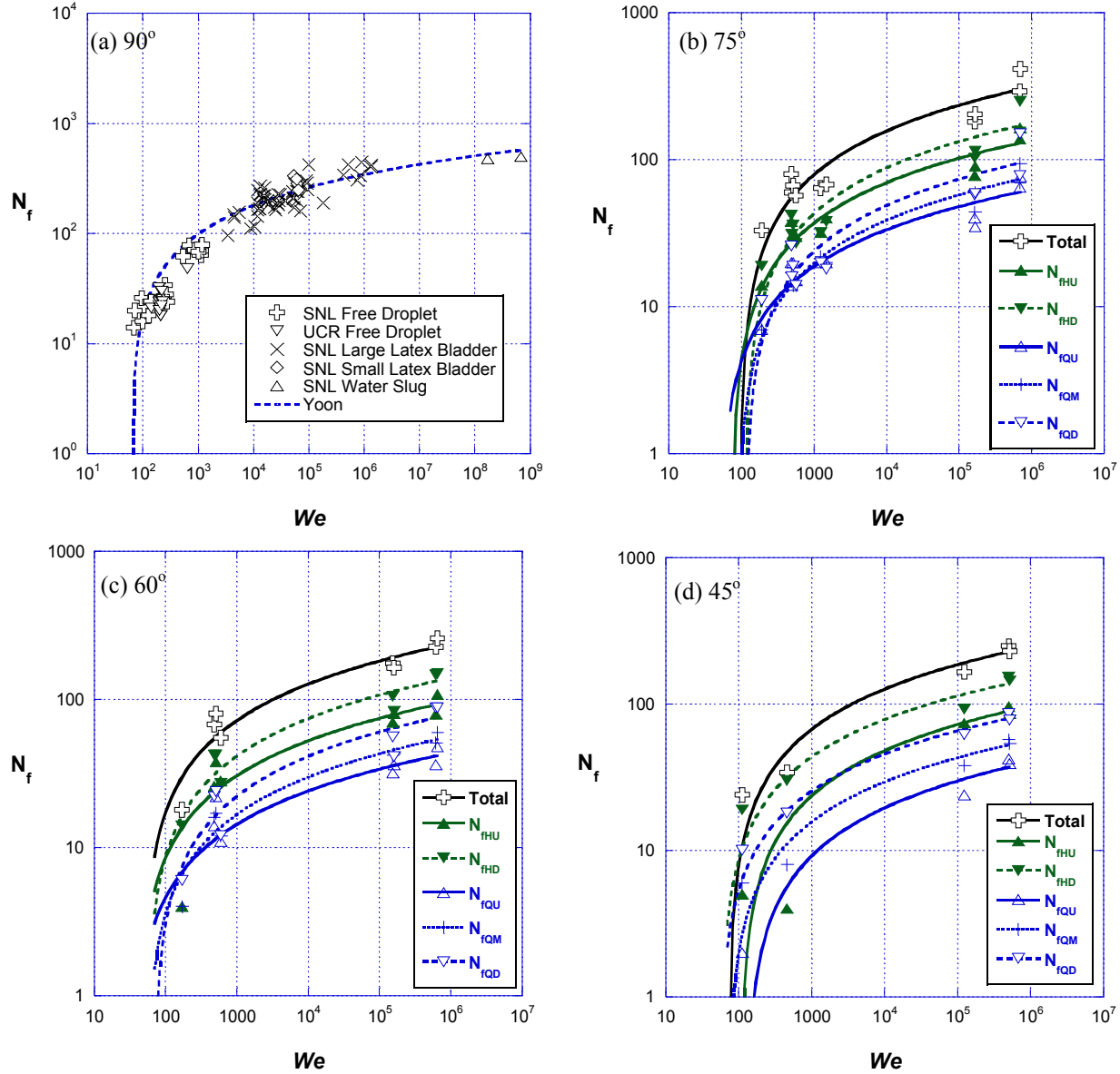
Figure 5. Number of fingers ( N_f ) vs. We at (a) 90^\circ , (b) 75^\circ , (c) 60^\circ , and (d) 45^\circ impact angles for water impacts. Results are from the Sandia small droplet tests, UCR pressure vessel tests at 1 atm, and the Sandia drop tower tests.
