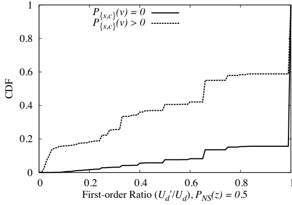
Fig. 5. The CDF for the first-order ratio of the ODP/SC08 hostnames.
