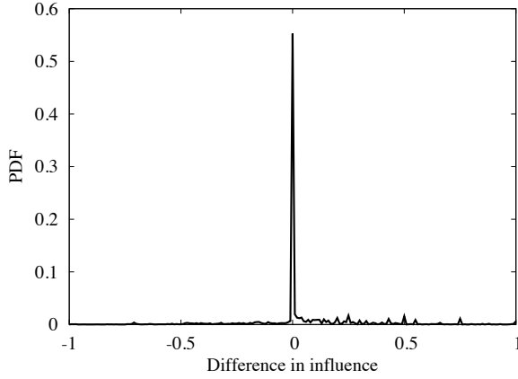
Fig. 3. The distribution of differences between the theoretical and empirical level of influence for each sample ODP name. Positive values indicate that the model predicted more influence than was observed.
