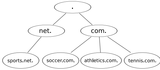
Fig. 1. The zone hierarchy for the the zone data shown in Table I.
