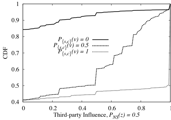
Fig. 6. The CDF for the third-party influence of the ODP/SC08 hostnames.
