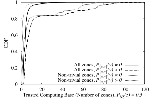
Fig. 4. The CDF for the size of the TCB of ODP/SC08 hostnames. Included are the CDF for the number non-trivial and total zones in the TCB, for P_{\{s,c\}}(v) = 0 and P_{\{s,c\}}(v) > 0 .
