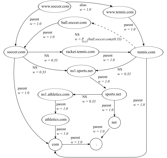
Fig. 2. The dependency graph for the domain name www.soccer.com , derived from the zone data in Table I. The solid lines represent active influence, and the dashed lines represent passive influence.
