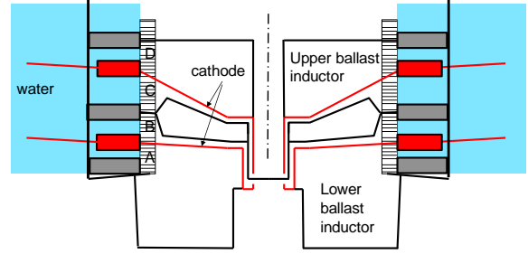
Figure 5. Schematic of the convoluteless method for inverting the polarity of a triaxial drive in vacuum.
