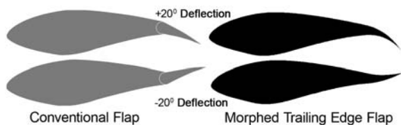
Figure 2. Conventional Flap and Morphing Trailing Edge Flap Shapes, 20% Chord Flap Length, \pm 20^\circ Deflection.
