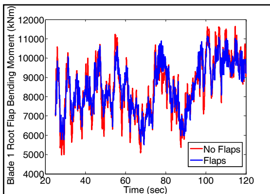
Figure 4. Impact of Morphing Trailing Edge Technology Control on Blade Root Flap Moment of WindPACT 1.5MW Turbine at 12m/s wind speed. Trailing Edge is 20% Chord, +/- 10° Maximum Deflection, 100°/sec Deflection Rate Limit.
