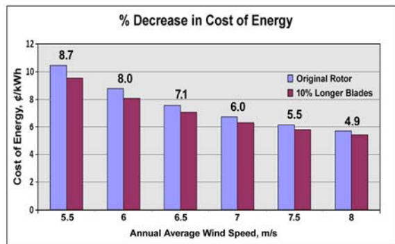
Figure 8. Impact of 10% Growth in Blade Length on the Cost of Energy for the WindPACT 1.5MW Turbine with AALC. MorphingTrailing Edge with 20% Chord, +/-10° Maximum Deflection, 100°/sec Deflection Rate Limit.
