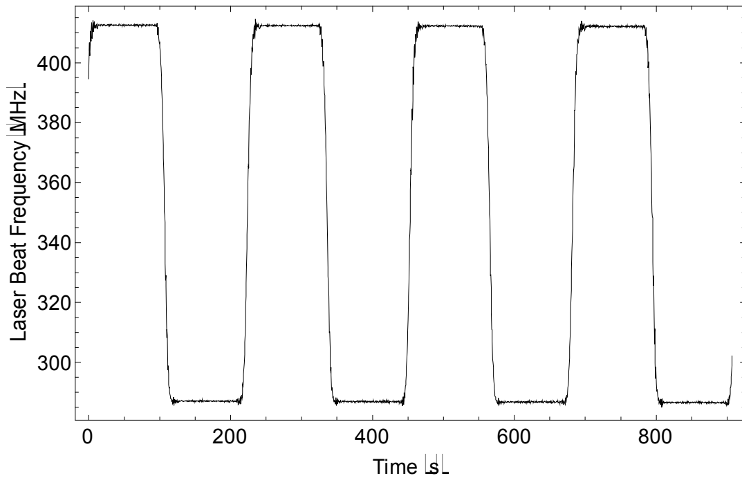
Fig. 3. An example of the laser beat frequency signal as the source masses are moved between the inner and outer positions changing the gravitational pull on the pendulum bobs. The 125 MHz signal corresponds to a change in pendulum bob separation of 90 nm.
