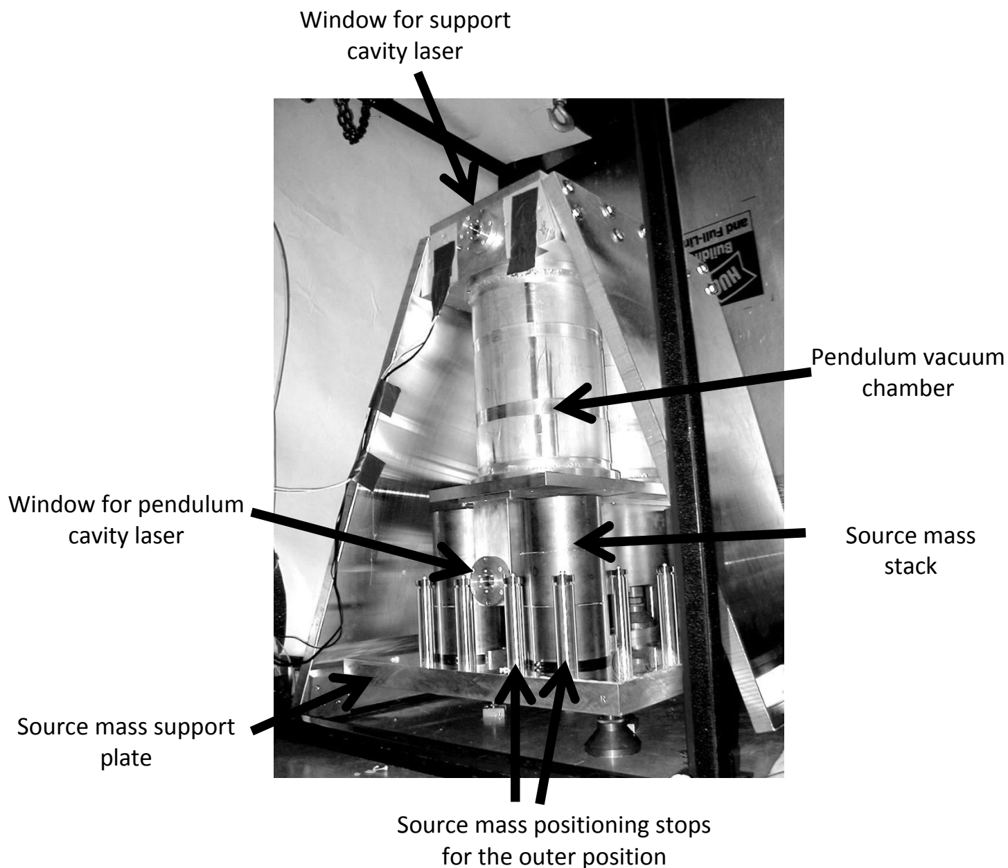
Fig. 2. A photograph of the apparatus. The pendulums are enclosed in a vacuum chamber, and the windows for the top and bottom cavity lasers can be seen. The vacuum chamber hangs from two “wing” plates that are bolted near the top of the chamber, so that it does not touch the source mass support palate. A source mass stack containing three tungsten billets can be seen. The stack float on an air bearing and was positioned by moving against stops that contact the source mass stack half way up. An insulated compartment was constructed around the apparatus to protect it from drafts.
