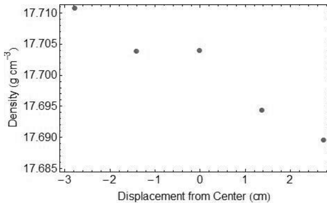
Fig. 7. The density of 1 inch diameter by 1 inch high cylinders cut along a diameter of one of the tungsten billets as a function of position.
