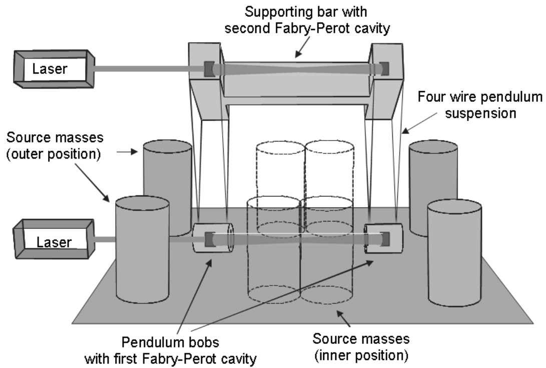
Fig. 1. A schematic of the apparatus. When the source masses are moved from the inner to the outer position, the change in the gravitational field causes the pendulum bob separation to change. This displacement is measured by beating a laser locked to a Fabry-Perot cavity formed from mirrors embedded in the pendulum bobs with a second laser locked to a cavity in the pendulum support.
