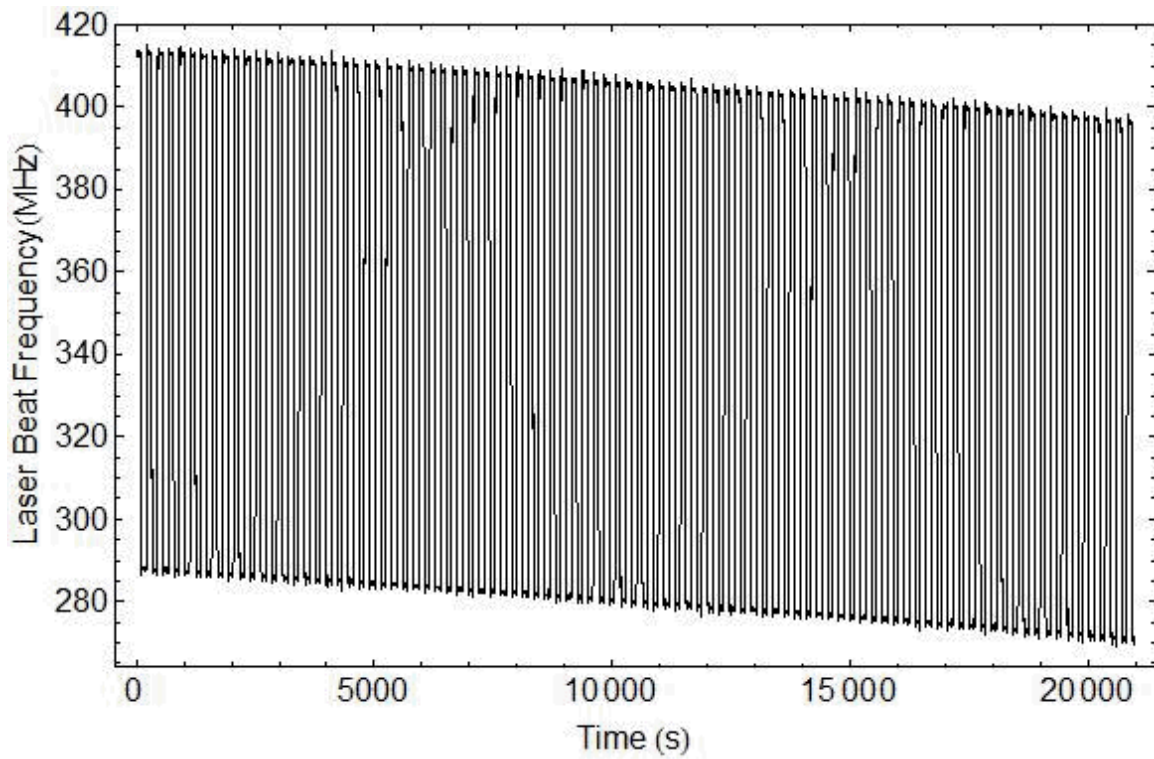
Fig. 4. A longer section of data from the set shown in Fig. 3. A slow drift in the pendulum displacement can be seen. This drift is consistent with 5 to 10 \mu\text{rad} change in floor tilt that is observed in the laboratory over the course of a day coupling into the signal due to the slight difference in the lengths of the two pendulums.
