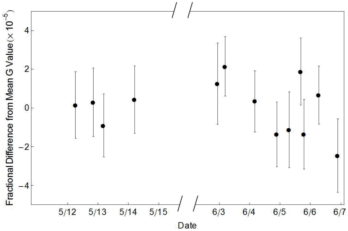
Fig. 5. The predicted G values from the individual data runs taken in 2004 as the fractional deviation \times 10^{-5} from the mean value of (6.672\ 34 \pm 000\ 15) \times 10^{-8} \text{ m}^3 \text{ kg}^{-1} \text{ s}^{-2} . The error bars include the uncertainty calculated from the data scatter within each data set root sum squared with the 1.5 \times 10^{-5} uncertainty associated with the day to day variations in the position measurements used in the calculation for G . The other systematic components not included in these error bars but are included in our uncertainty in our mean G value.
