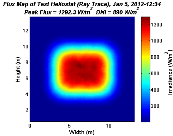
Figure 6: Simulated irradiance distribution on the long-range heliostat target on January 5, 2012 at 12:34 pm. reflectivity=.85, slope error = 1 mrad, DNI=890, Focal length=1500m, peak flux = 1292 W/m 2
