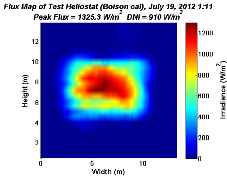
Figure 9: Flux map of test heliostat beam as rendered by LRHT on July 19, 2012 at 1:11pm. DNI=910, peak flux = 1325 W/m 2
