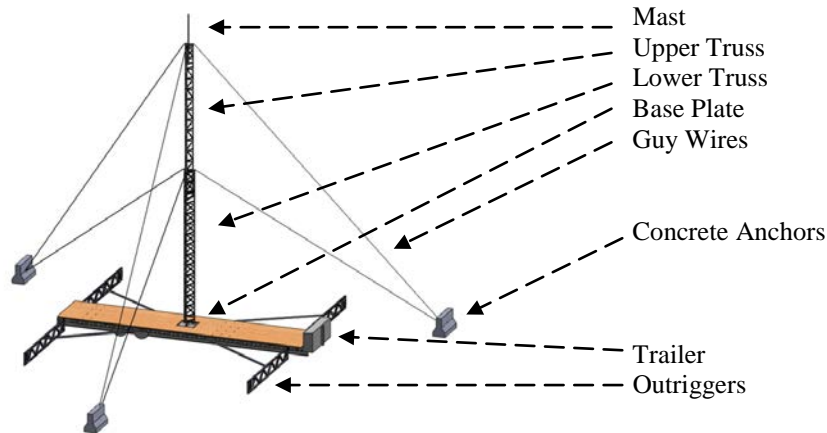
Figure 1: Long-range heliostat target assembly
