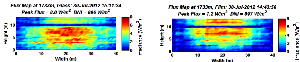
Figure 12: LRHT flux maps of two single facets made of glass (left) and reflective film (right) at a distance of 1733 m.
