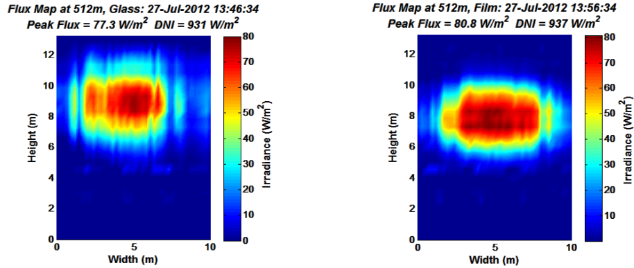
Figure 10: LRHT flux maps of two single facets made glass (left) and reflective film (right).
