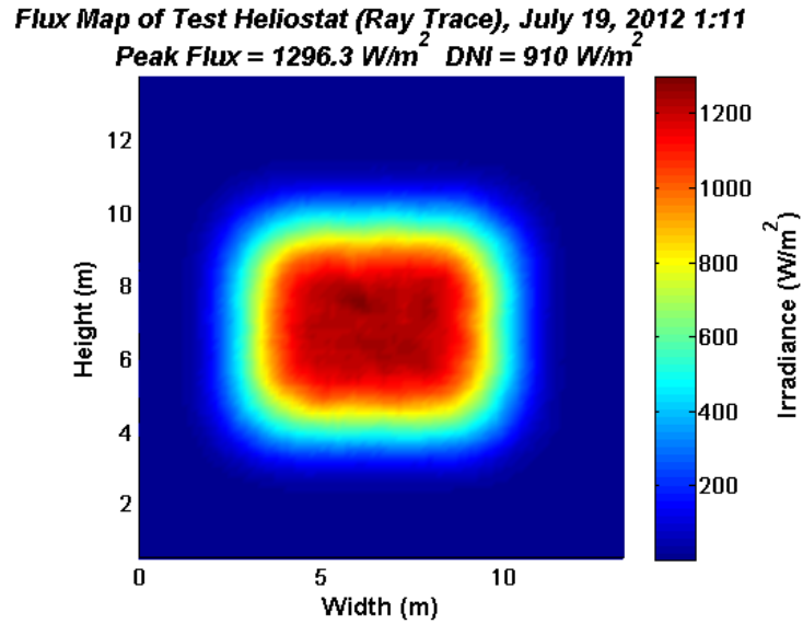
Figure 8. Simulated irradiance distribution on the long-range heliostat target at 1:11pm, July 19, 2012, DNI = 910 W/m 2 , RMS slope error = 1 mrad, reflectivity = 0.85, focal length = 1500 m. Peak flux=1,296W/m 2 .
