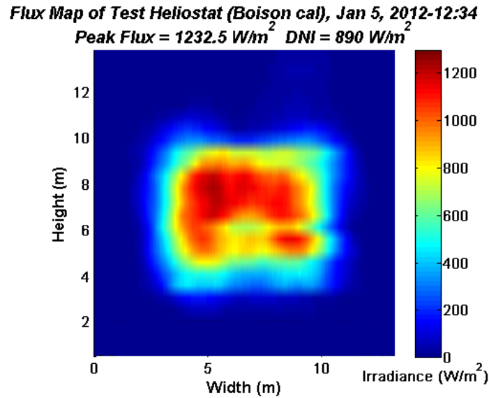
Figure 7: Flux map of test heliostat beam as rendered by LRHT on January 5, 2012 at 12:34 pm. DNI=890, peak flux = 1233 W/m 2
