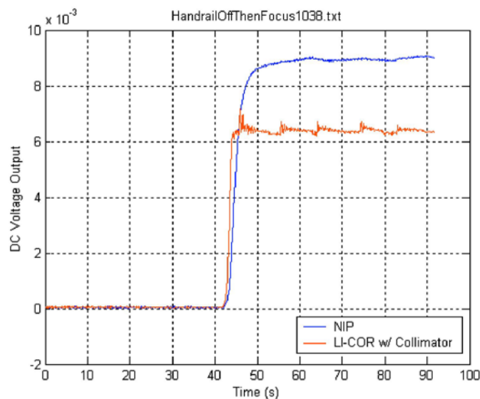
Figure 4: Voltage response of LI-COR and NIP. (Figure provided courtesy of Dan Fisher)
