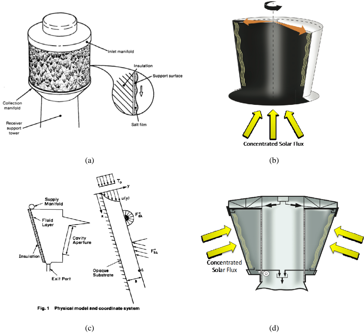
Figure 6. Falling liquid films for heat absorption in (a) direct-exposure, external receivers for a surround field [80]; (b) direct-exposure, internal receivers for a surround field; (c) direct-exposure, internal receivers for a north-facing field [75]; and (d) indirect-exposure, internal film receivers for surround or north-facing fields.
