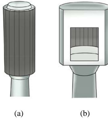
Figure 3. Schematics of tubular (a) external and (b) cavity receivers.
