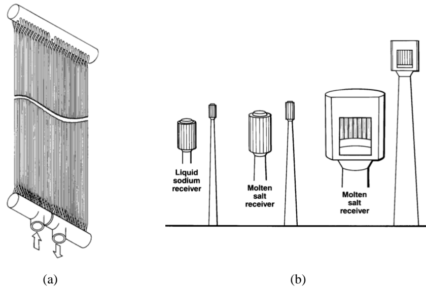
Figure 5. (a) Schematic of a tubular panel and (b) relative tower heights/receiver sizes for a liquid sodium and molten salt tubular receivers (from [7]).
