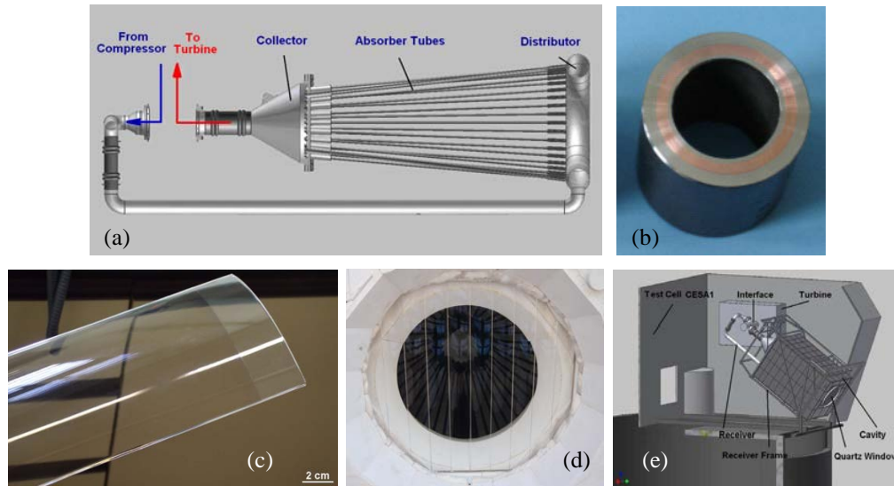
Figure 2. Design concepts from DLR: (a) tubular air-turbine receiver, (b) multi-layer tube with copper in between Inconel, (c)-(d) segmented parts of glass tubes to form a window on the receiver aperture, and (e) schematic of receiver and microturbine on top of a tower [30, 31, 33].
