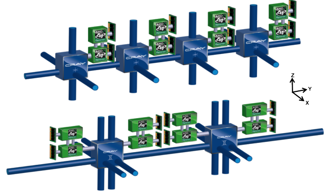
Fig. 3. XE6 Gemini (bottom) and SeaStar (top) interconnects. Image courtesy of Cray, Inc.
