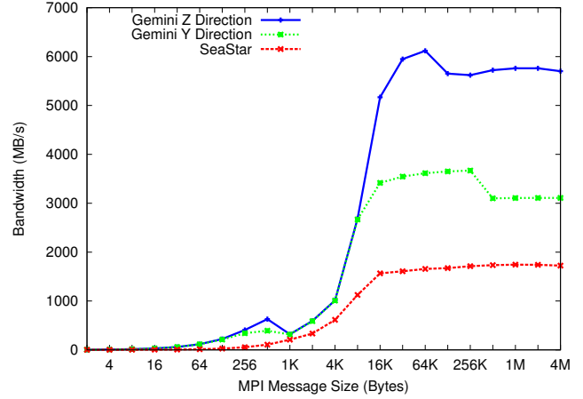
Fig. 5. Point-to-Point Bandwidth: Gemini vs. SeaStar
