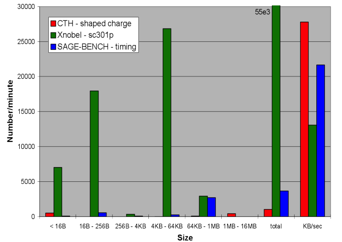
Fig. 7. Per core point-to-point message traffic for the three applications. Note that the total volume for xNOBEL continues well off the view of this graph, up to 55,000 messages per minute.
